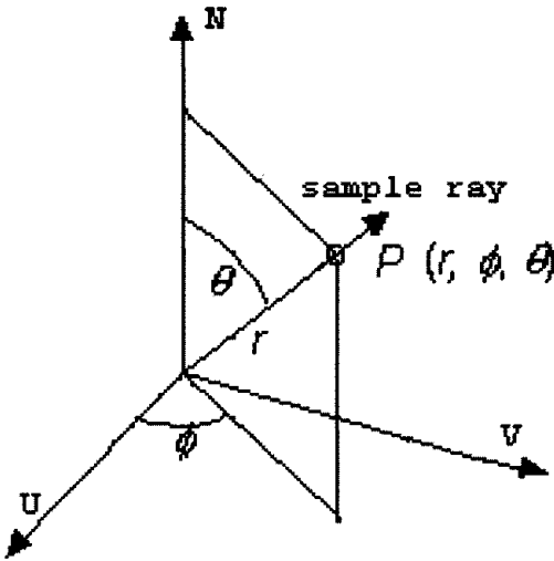
Figure 13. P is a point on the hemisphere. r is the radius of the hemisphere. \theta has a range of [0, 90] degrees. \phi has a range of [0, 360] degrees.
