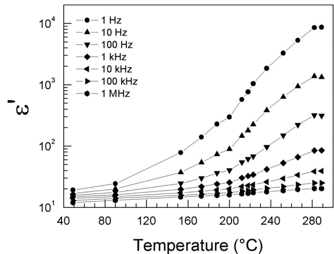
FIG. 5. Temperature dependence of the measured dielectric constant of the \text{Ba}_2\text{BiSbO}_6 between 1 Hz and 1 MHz.
