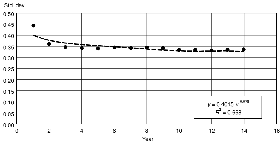
Fig. 10. \sigma -Convergence at NUTS 3 level – differences in GDP p.c. among Landkreise in 1992–2006 measured by standard deviation level
