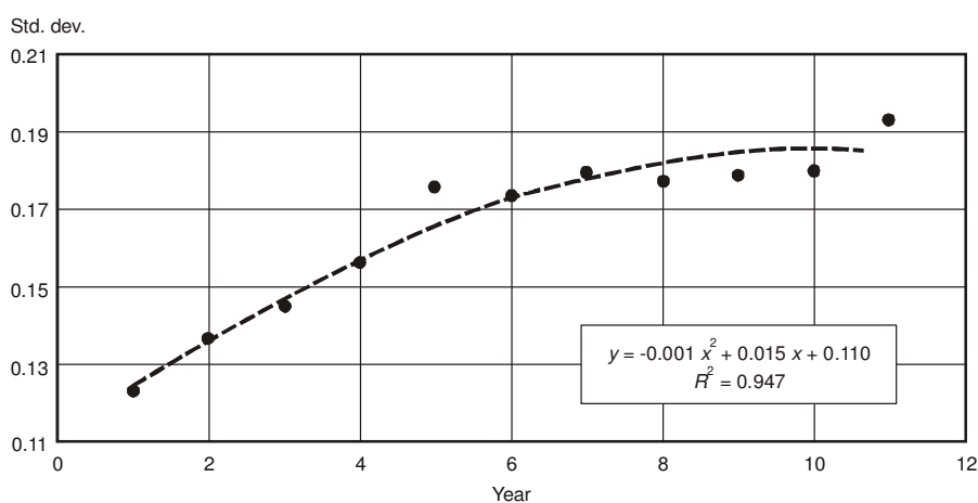
Fig. 2. \sigma -Convergence at NUTS 1 level (a) – differences of GDP p.c. among Polish regions in years 1995–2005 measured by standard deviation
