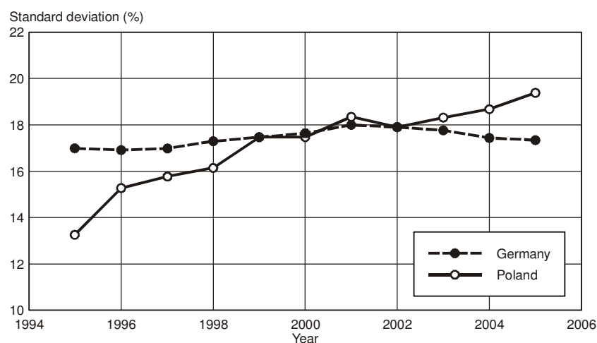
Fig. 1. GDP p.c. differences in Poland and Germany (NUTS 2 level, standard deviation %)
