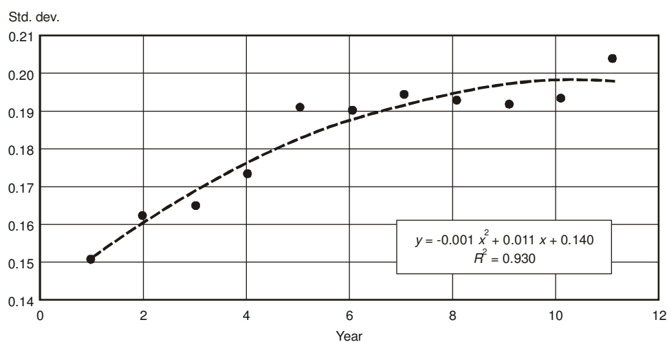
Fig. 4. \sigma -Convergence at NUTS 2 level (a) – differences in GDP p.c. among 16 voivodships in years 1995–2005 measured by standard deviation
