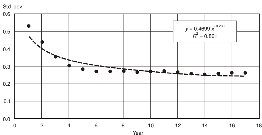
Fig. 8. \sigma -Convergence at NUTS 1 level – GDP p.c. differences among 16 Bundesländer in 1991–2007 measured by standard deviation level
