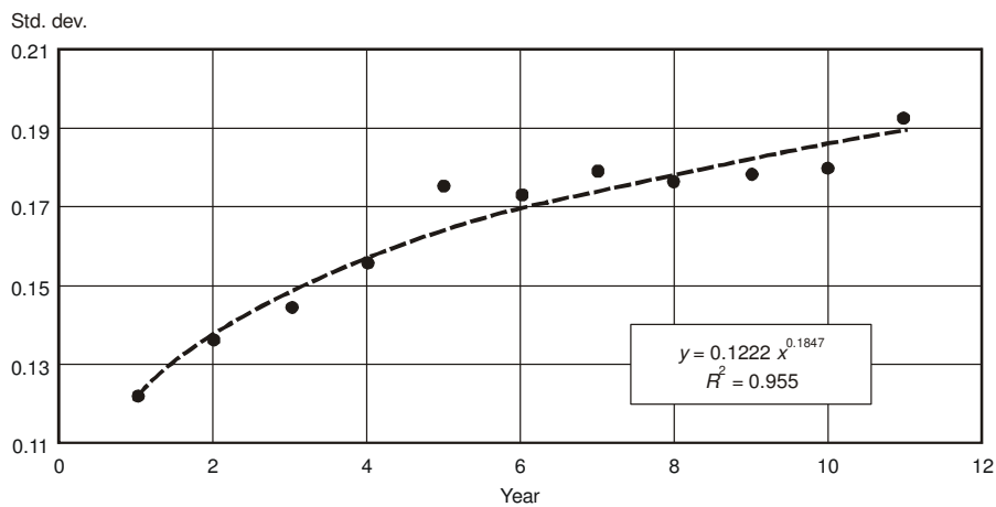
Fig. 3. \sigma -Convergence at NUTS 1 level (b) – differences of GDP p.c. among Polish regions in years 1995–2005 measured by standard deviation
