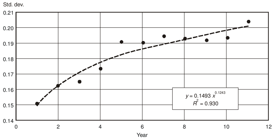
Fig. 5. \sigma -Convergence at NUTS 2 level (b) – differences in GDP p.c. among 16 voivodships in years 1995–2005 measured by standard deviation
