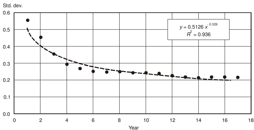
Fig. 7. \sigma -Convergence between former DDR and BRD in 1991–2007 measured by standard deviation level
