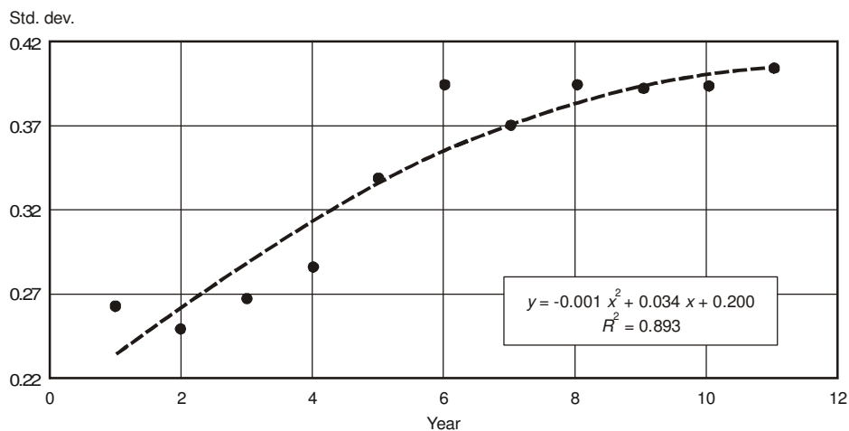
Fig. 6. \sigma -Convergence at NUTS 3 level – differences in GDP p.c. among group of poviats in years 1995–2005 measured by standard deviation
