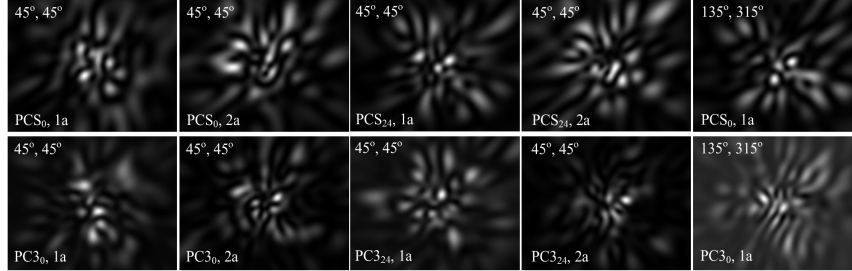
Fig. 3. Normalized p-DI images of J_{ss}(y, z) of 640 \times 480 pixels derived from different OCMs and orientations of C(\theta_0, \phi_0) . The upper and lower labels are values of (\theta_0, \phi_0) and (ID_{cell}, ID_{RI}) for OCM.
