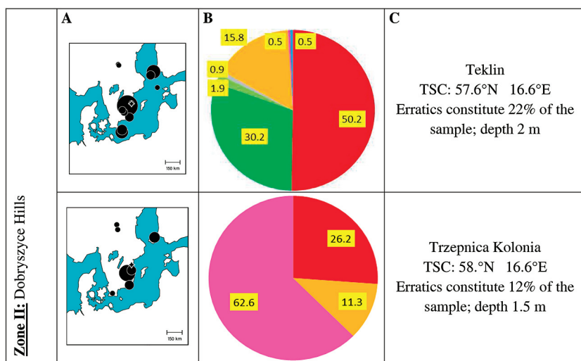
Fig. 14. Extended petrographical analysis of the coarse gravel (20–60 mm fraction) from zone II A: Source areas of the indicator erratics with locations of the TSC (theoretical stone centre); B: Percentages of the various petrographical types of the coarse (20–60 mm) gravel; C: Additional information
