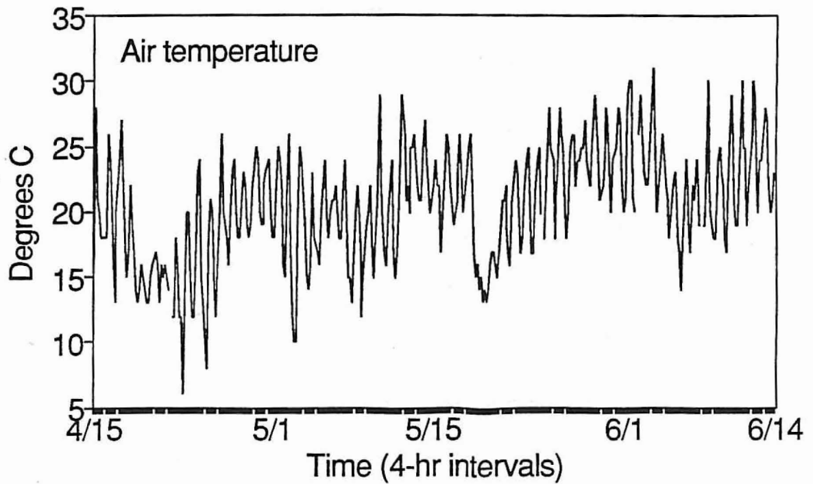
Figure 7. Air temperature ( ^{\circ}\text{C} ) measured at Barnhill's Landing, NC, for the period 15 April to 14 June 1991.
