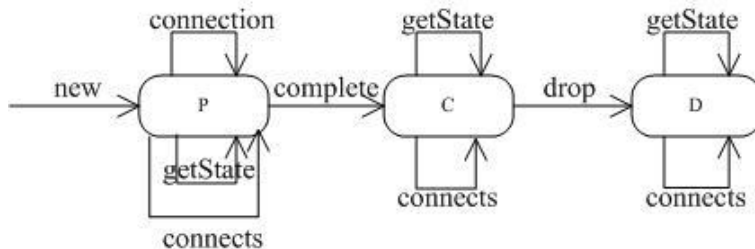
Figure 4: State model of connection class
