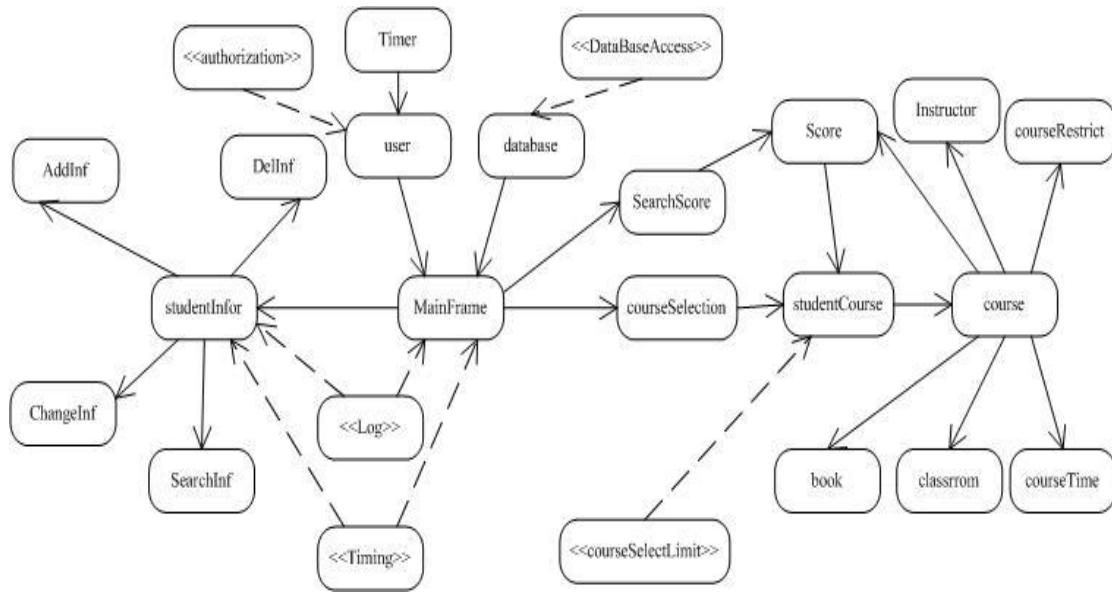
Figure 22: Architecture of SIMS
