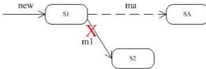
Figure 8: FSM for Advice type around
