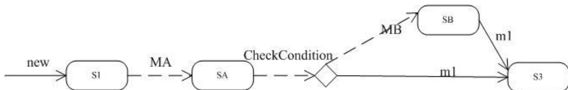
Figure 11: FSM for A \cdot B
