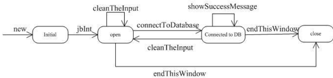
Figure 13: State model for class AddInf
