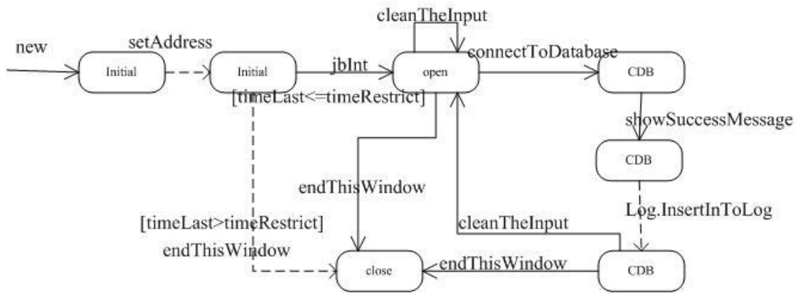
Figure 17: Woven model for AddInf
