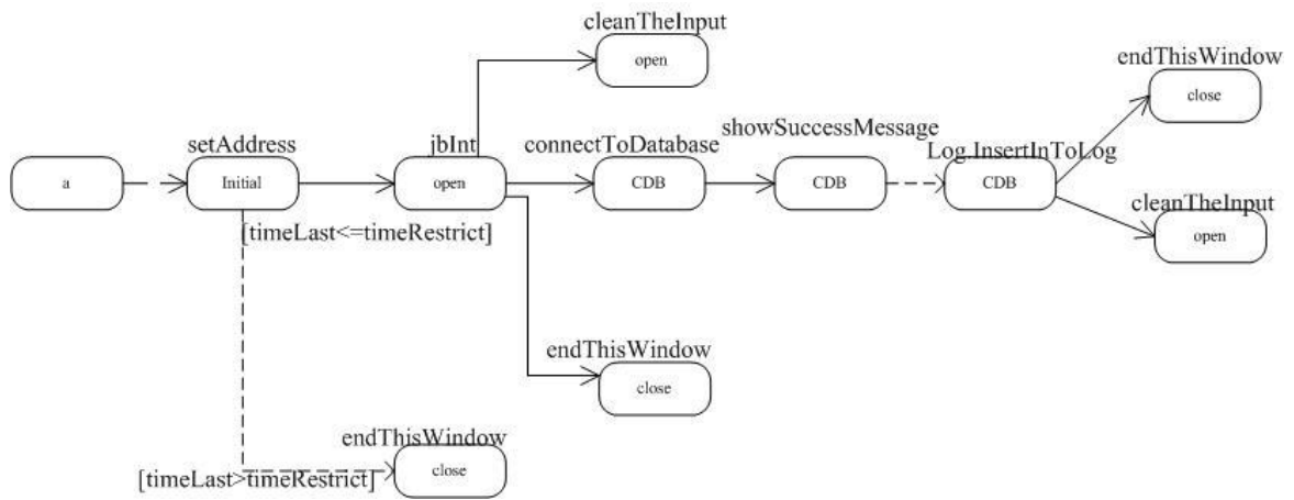
Figure 20: Transition Tree without Prioritizing
