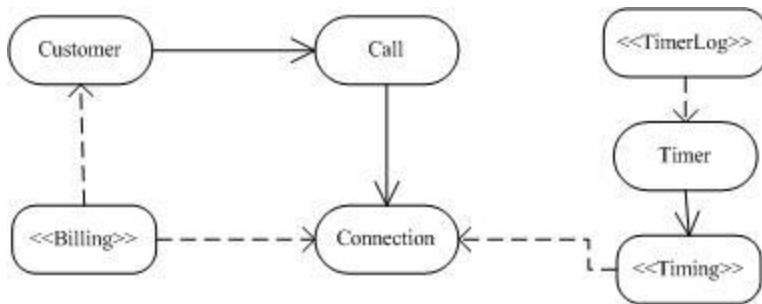
Figure 21: Architecture of Telecom
