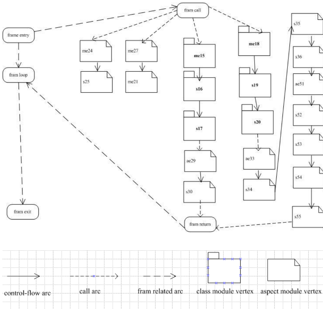
Figure 18: FCFG for connection class, Timing Aspect, and Billing Aspect
