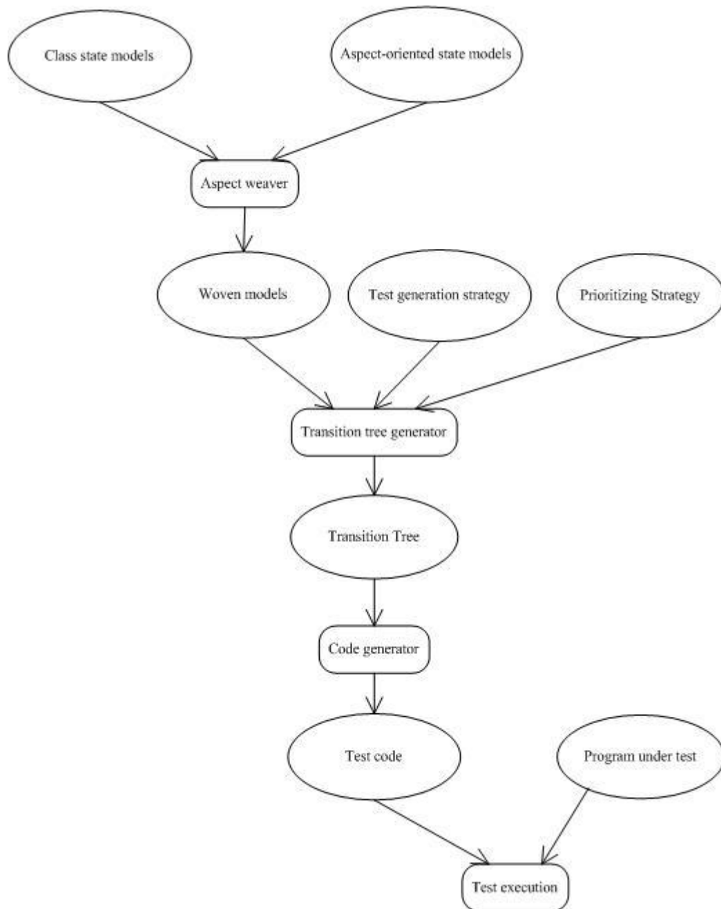
Figure 19: Overview of testing process
