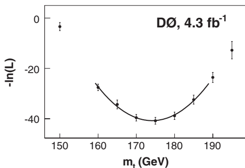
FIG. 1. -\ln L as a function of m_t for the combined ee , e\mu , and \mu\mu channels. A parabolic fit is shown near the minimum value in m_t .
