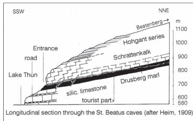
Fig. 1. Longitudinal section through the St Beatus caves (after Heim, 1909).
