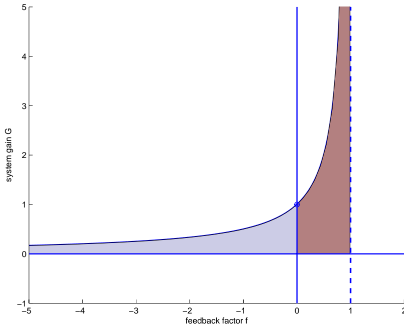
Fig. 2.1: Non-linear relationship between system gain G and feedback factor f . The bluish (reddish) shaded area under the curve illustrates a damping (amplification) of the system response, resulting from a negative (positive) feedback factor. The circle represents the system response without indirect feedbacks. The system behaviour for f > 1 yields physically implausible results and is not shown.
