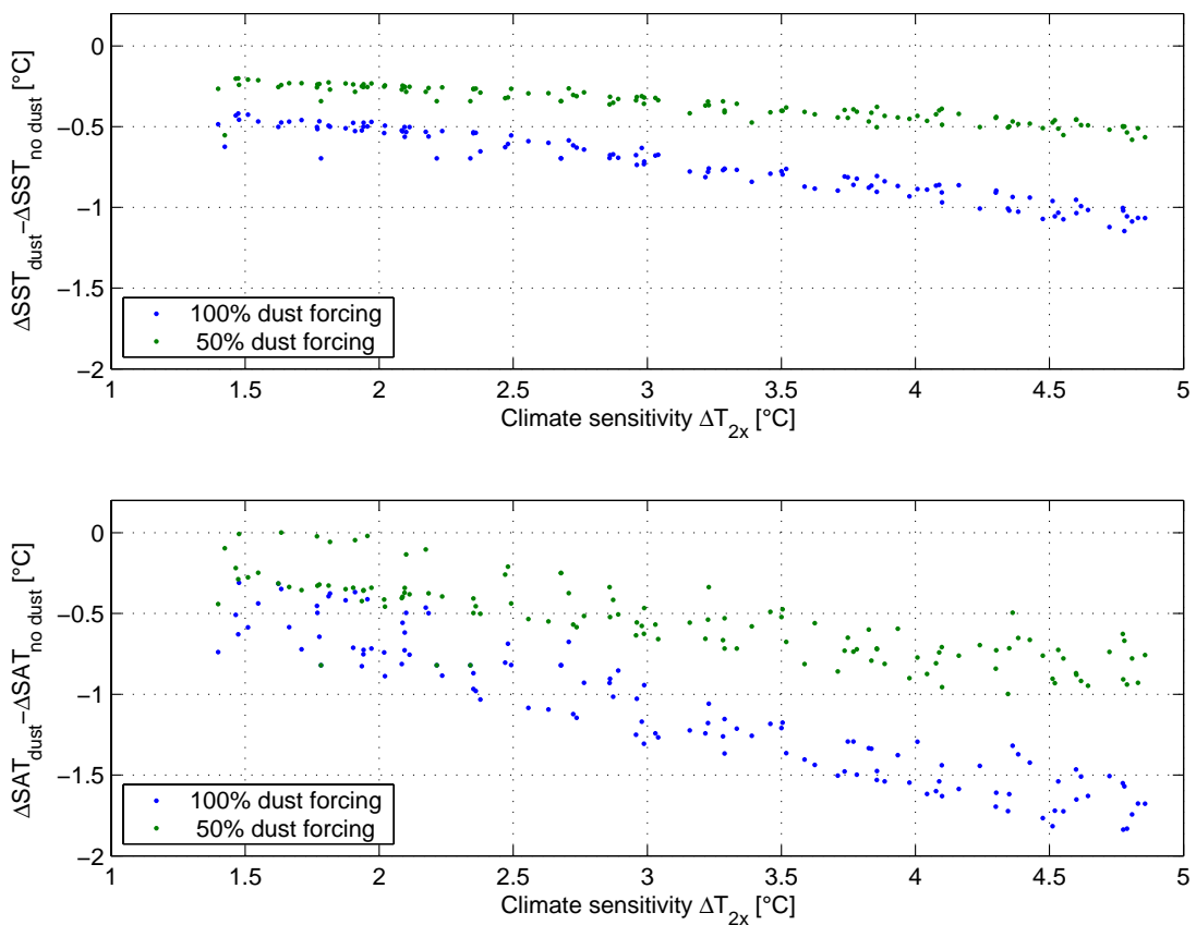
Fig. 5.15: Additional glacial cooling through dust forcing. Shown is the difference in LGM cooling between model versions, which account for dust forcing (green dots: 50% dust forcing, blue dots: 100% dust forcing) and the same model versions without being forced by glacial dust, illustrated for tropical Atlantic SST decrease (upper panel) and Eastern Antarctic SAT decrease (lower panel).
