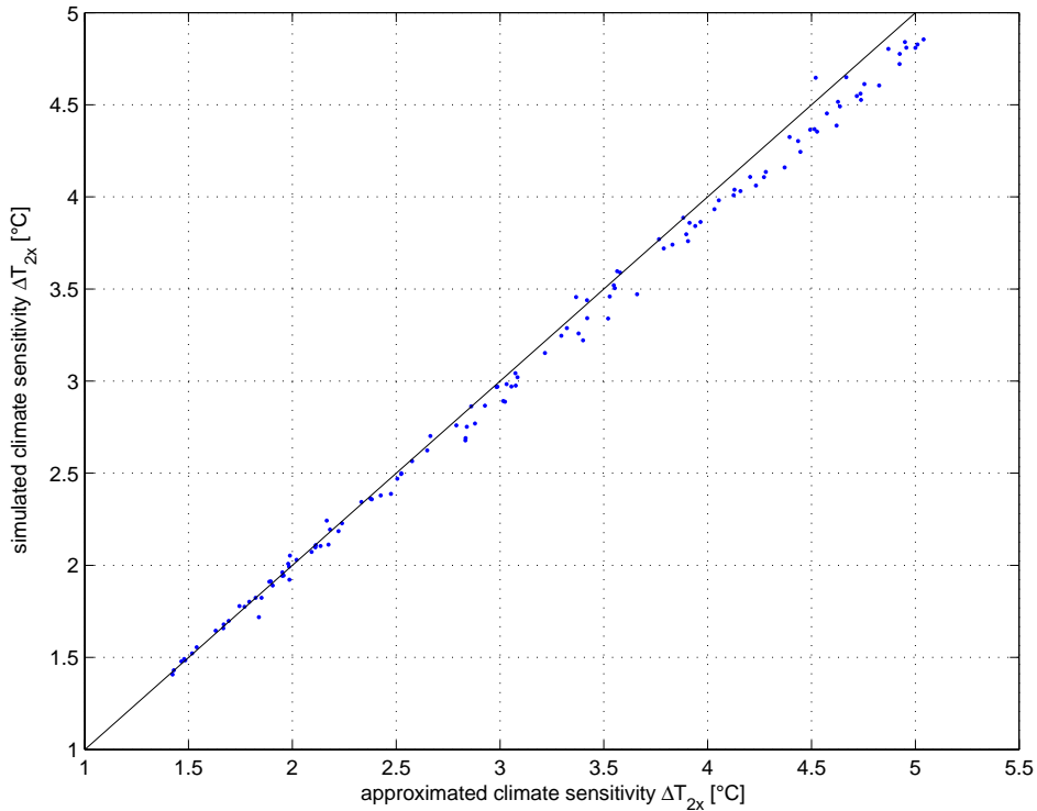
Fig. 5.18: Comparison of approximated and simulated change in global-mean equilibrium surface temperature for a doubling of CO 2 . Approximated temperature responses have been inferred by assuming that the system response can be described by a linear superposition of all individual model feedbacks (equation 2.13). Feedback strengths and simulated temperature changes have been inferred from model versions of the correlated parameter ensemble (constrained by present-day data).
