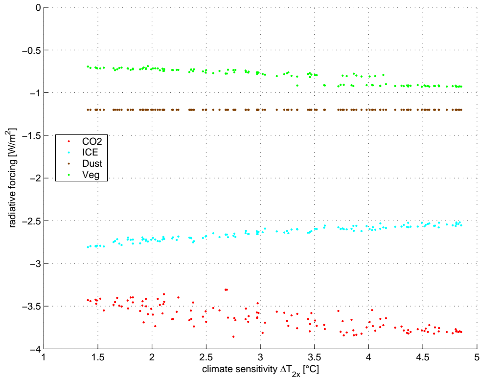
Fig. 5.5: Simulated global annual-mean radiative forcing for all main individual glacial forcing agents (red: CO 2 , cyan: ice sheets, brown: dust, green: vegetation). Shown are estimates of all model versions (correlated ensemble), which are consistent with present-day climate characteristics. Besides dust forcing all estimates slightly depend on the set of chosen model parameters (see text).
