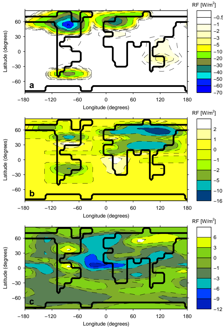
Fig. 5.8: Spatial LGM forcing. Shown is the annual mean radiative forcing for glacial ice sheets (a), vegetation cover (b), and dust (c). All values represent the ensemble mean of model versions constrained by tropical proxy-data. Note that apparent geographical overlap between ice sheet and vegetation forcing results from the facts that due to a coarse spatial model resolution some grid cells are only partially covered by ice sheets, and in these grid cells both, ice sheets and vegetation forcing, are nonzero. Another reason for the apparent overlap is the used graphical interpolation, which causes a smoothing of the contour lines.
