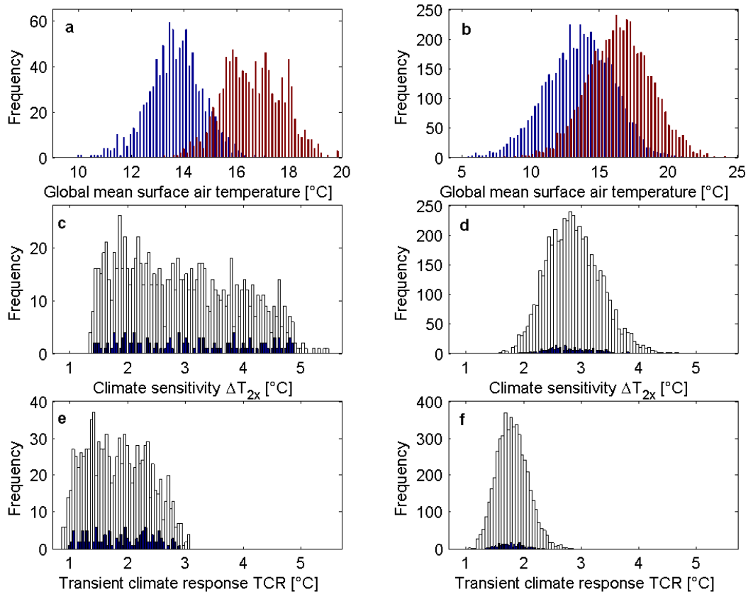
Fig. 5.1: Frequency distributions for pre-industrial and 2xCO_2 climate characteristics (left: correlated ensemble, 1000 runs), right: uncorrelated ensemble (5000 runs)). a , b : simulated equilibrium global-mean surface air temperature for 280 p.p.m. (blue) and 560 p.p.m. CO_2 (red); c , d : corresponding distribution of climate sensitivity \Delta T_{2x} , calculated as the difference of the two equilibria, and e , f : transient climate response TCR. Dark blue bars (c-f) denote model versions consistent with present-day data. The nearly uniform shape (c and e) mainly result from the chosen sampling scheme (see section 4.3).
