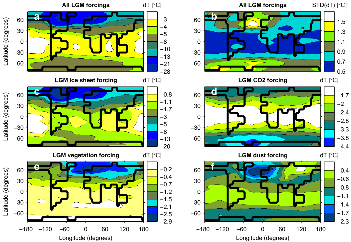
Fig. 5.9: Spatial LGM cooling. Shown is the annual SAT temperature anomaly (glacial / pre-industrial) resulting from the prescription of all main forcings (a), and from individual forcings of ice sheets (c), CO 2 (d), vegetation (e) and dust (f). All data represent the mean values for the ensemble constrained by tropical SST proxy-data. The spread from the mean is illustrated in (b).
