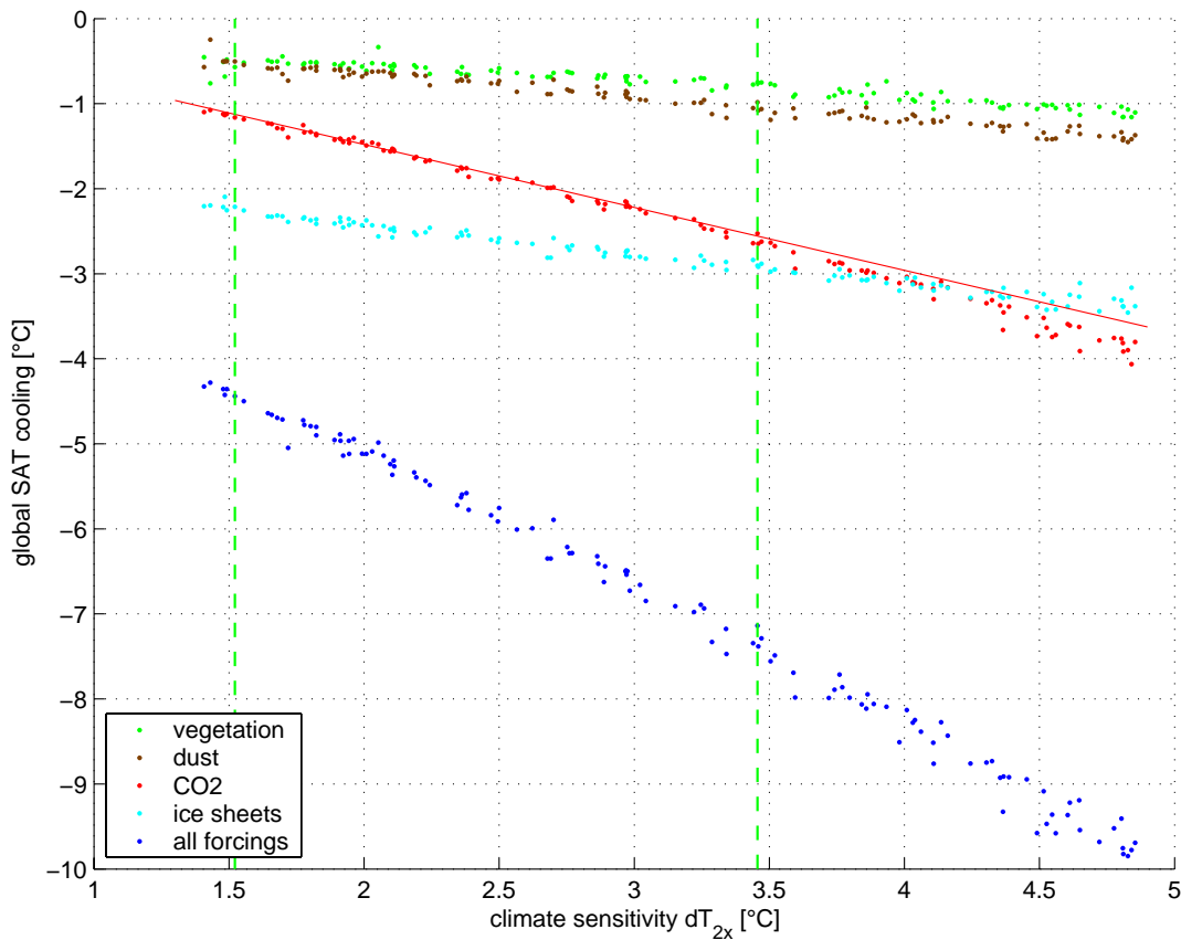
Fig. 5.6: Contribution of individual forcings to global LGM cooling. Shown is the magnitude of simulated global annual-mean SAT cooling between the pre-industrial and LGM climate, arising from the prescription of all main glacial forcings (dark blue dots). Additionally the change in SAT for individual forcing components is illustrated (green: vegetation, brown: dust, red: CO 2 , cyan: ice sheets). The solid red line represents a theoretical approximation, which assumes a linear relation between the temperature anomaly resulting from lowered CO 2 levels and CO 2 radiative forcing (see main text). Vertical green lines indicate the range of model versions, consistent with a tropical Atlantic SST cooling of 3.0^{\circ} \pm 0.9^{\circ}\text{C} .
