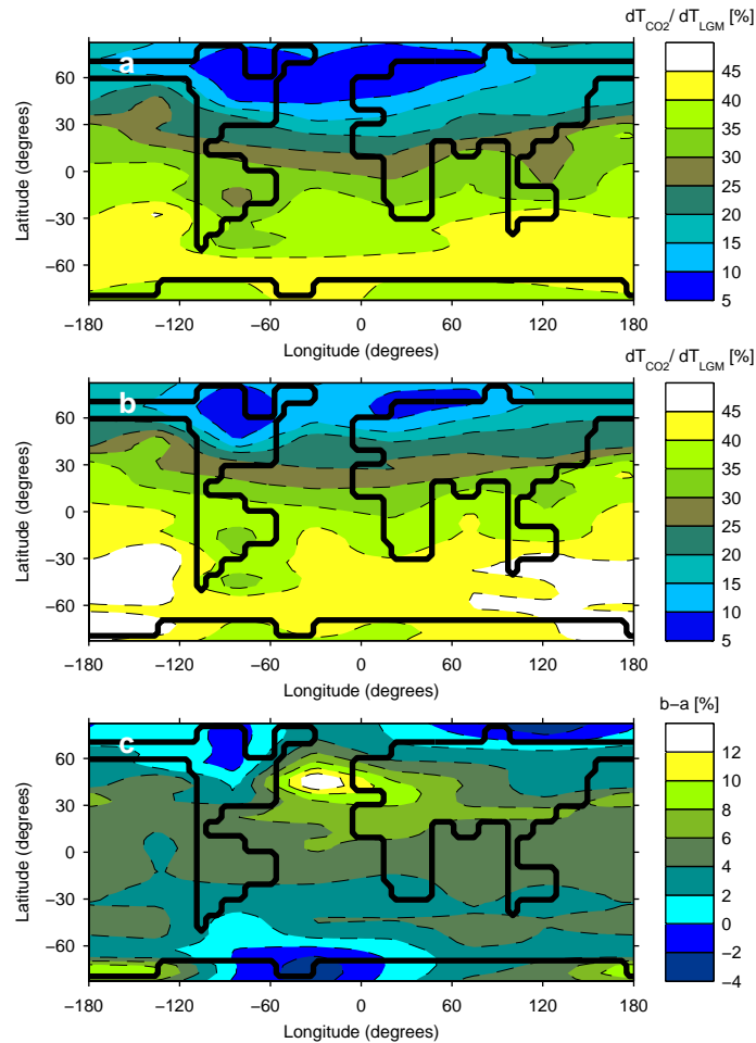
Fig. 5.11: Ratio of CO 2 attributable SAT cooling to total LGM SAT cooling. Panel (a) and (b) show the percentage of LGM cooling, caused by the glacial drop in the concentration of GHGs, for the ensemble mean of all present-day consistent model versions. Simulation results from (a) were inferred from an additional ensemble with prescribed glacial CO 2 content while keeping all other boundary conditions fixed to pre-industrial values, for (b) all boundary conditions were set to LGM conditions, but CO 2 fixed to its pre-industrial value. The difference (in %) between both experiments (b-a) is illustrated in the lowest panel (c).
