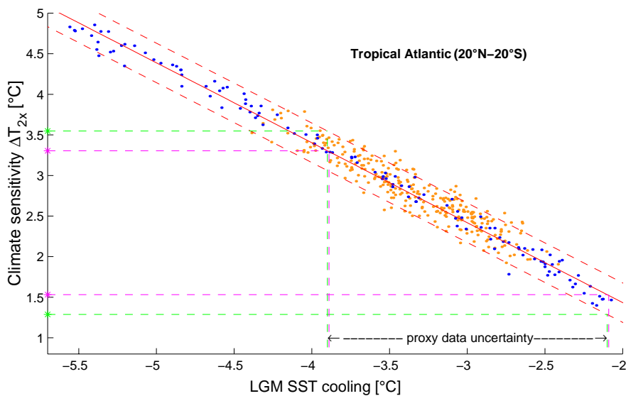
Fig. 5.14: Inferring \Delta T_{2x} from LGM data. Simulated annual mean tropical Atlantic SST cooling (averaged from 20°N-20°S) is shown for correlated (blue dots) and uncorrelated parameter ensembles (orange dots). The red curve shows the linear fit to the correlated ensemble, the red dotted lines represent the fit-error, conservatively estimated from the uncorrelated ensemble as the 5-95 percentile of the spread of deviations from the fit. Only runs consistent with present-day data are shown. Purple (green) dashed lines illustrate the range of \Delta T_{2x} (including fit-error bounds) consistent with a mean tropical Atlantic SST cooling of 3.0 \pm 0.9^\circ\text{C} .
