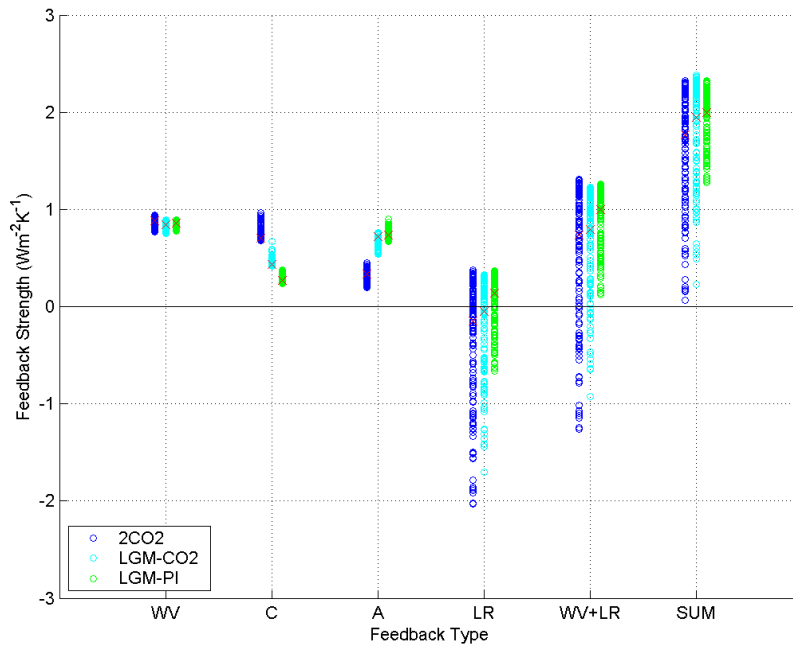
Fig. 5.21: Dependence of the feedback strengths on the climate state and forcing pattern. Shown are the individual mean feedback strengths for the correlated ensemble for a 2xCO_2 and for two glacial scenarios. In case of the first glacial experiment ( LGM-PI ) the transgression from the glacial to the pre-industrial climate is analysed (full set of glacial forcings), whereas in the second experiment ( LGM-CO 2 ) only changes in the CO_2 content (from 170 p.p.m. to 230 p.p.m.) constitute the forcing. All model versions are consistent with pre-industrial climate characteristics.
