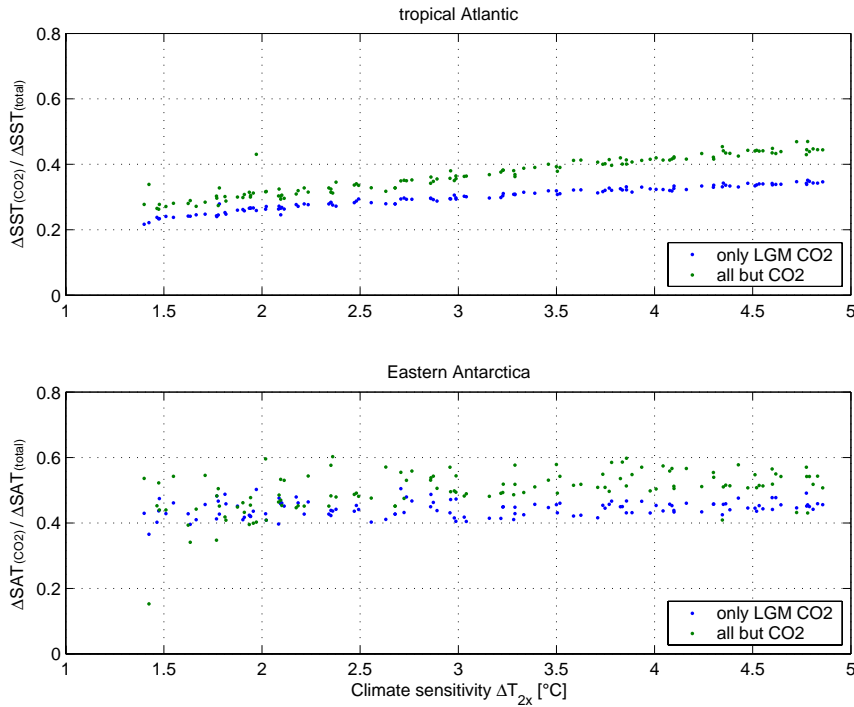
Fig. 5.12: Fraction of LGM cooling attributable to CO 2 lowering. Shown is the ratio of annual mean LGM cooling, attributable to CO 2 concentration changes, to total LGM cooling (tropical Atlantic SSTs: upper panel, Eastern Antarctic SAT: lower panel). Blue dots represent model results obtained for changes in CO 2 content only (SIM_CO 2 _LGM), green dots for prescribing all glacial forcings but CO 2 (SIMabCO 2 _LGM).
