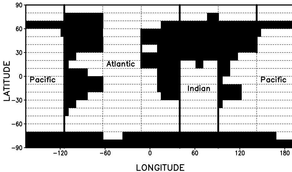
Fig. 4.1: Continental mask of CLIMBER-2. Solid lines separate the three ocean basins (Pacific, Atlantic, Indic), dashed lines illustrate the atmospheric grid boxes.
