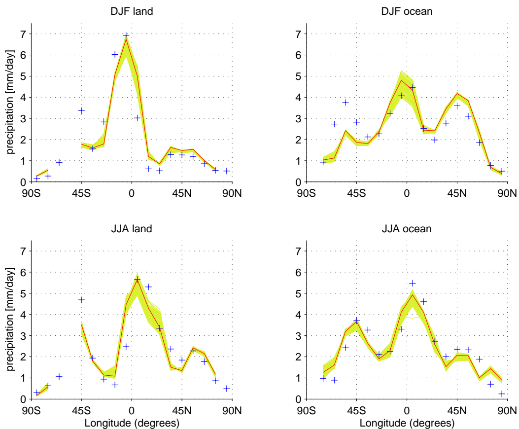
Fig. 5.3: Zonally averaged precipitation over land and oceans, shown for northern hemisphere winter (upper panel) and summer (lower panel). The light-green lines represent the latitudinal profile of all present-day consistent model members from the correlated ensemble (123 runs), while the red line illustrates the profile for the basic CLIMBER-2 parameter combination. Blues crosses show an estimate from observational data (JAEGER, 1976).
