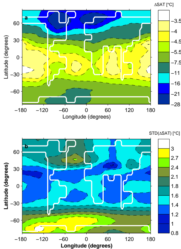
Fig. 5.10: Regional mean SAT cooling. The upper panel (a) shows the annual mean SAT anomaly between the LGM and pre-industrial climate for all present-day consistent ensemble members, the lower panel (b) shows the corresponding standard deviation among those model versions.
