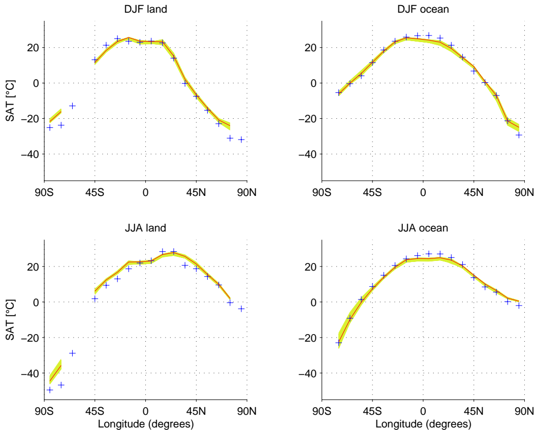
Fig. 5.2: Zonally averaged surface air temperature (SAT) over land and oceans, shown for northern hemisphere winter (upper panel) and summer (lower panel). The light-green lines represent the latitudinal profile of all present-day consistent model members from the correlated ensemble (123 runs), while the red line illustrates the profile for the basic CLIMBER-2 parameter combination. Blue crosses show an estimate from observational data (GUACA, 1993).
