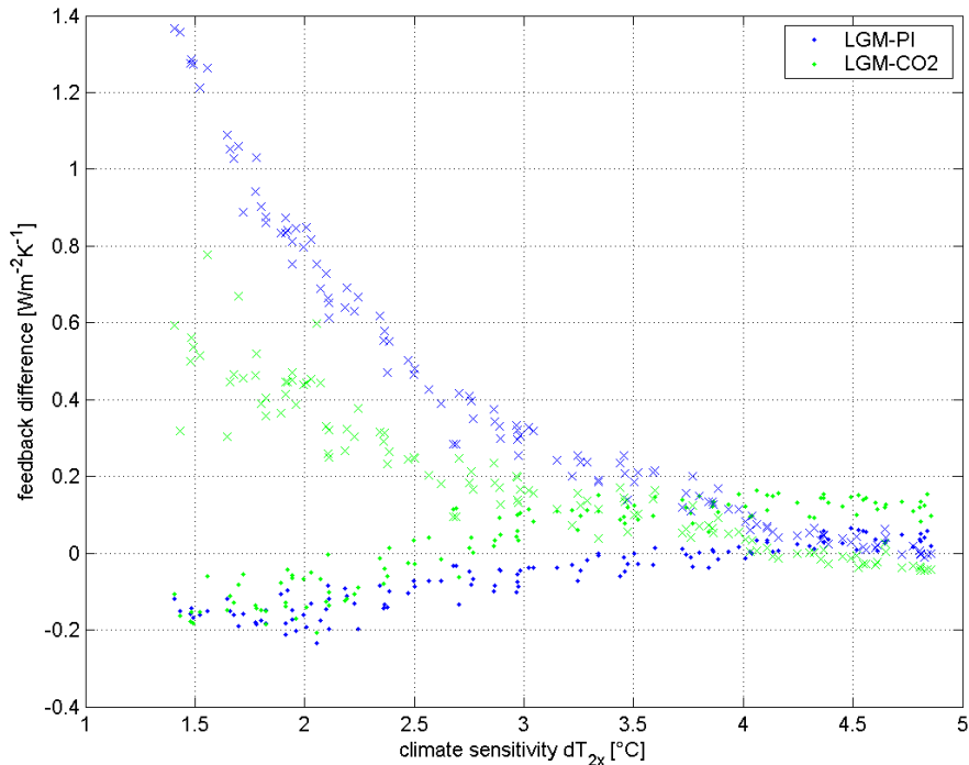
Fig. 5.23: Contribution of individual feedbacks to the discrepancy in the aggregate mean feedback strength. The difference in the magnitude of individual feedbacks between the 2x\text{CO}_2 and both glacial experiments ( LGM-PI : blue, LGM-CO 2 : green) is shown for the combined albedo and cloud feedback (dots) as well as for lapse rate feedback (crosses). Positive (negative) values indicate a larger (smaller) feedback in the glacial experiments than in the doubling of \text{CO}_2 simulations.
