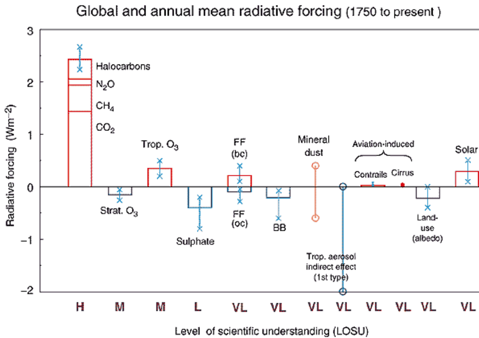
Fig. 3.2: Global, annual mean radiative forcings for the industrial period (1750 to 2000); figure from IPCC (2001). The height of the rectangular bar indicates that a central or best estimate value while its absence denotes no best estimate is possible. The vertical line about the rectangular bar with “x” delimiters indicates an estimate of the uncertainty range, a vertical line without a rectangular bar and with “o” delimiters denotes a forcing for which no central estimate can be given owing to large uncertainties. A “level of scientific understanding” index is accorded to each forcing, with H, M, L and VL denoting high, medium, low and very low levels, respectively.
