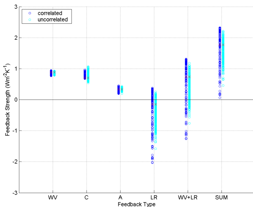
Fig. 5.17: Range of simulated model feedbacks for correlated (dark blue) and uncorrelated (cyan) parameter ensembles. Shown are the mean feedback strengths for all individual global feedback components (WV: water vapour, C: cloud, A: albedo, LR: lapse rate). Additionally the range of the combined effect of water vapour and lapse rate (WV+LR) and the sum of all feedbacks (SUM) are shown. Positive values indicate an amplification of an initial radiative perturbation, negative values a weakening. All model versions shown are consistent with pre-industrial climate constraints.
