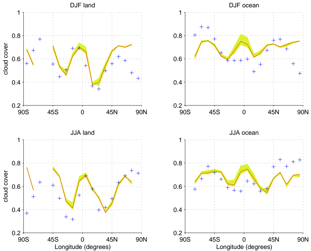
Fig. 5.4: Zonally averaged cloud cover over land and oceans, shown for northern hemisphere winter (upper panel) and summer (lower panel). The light-green lines represent the latitudinal profile of all present-day consistent model members from the correlated ensemble (123 runs), while the red line illustrates the profile for the basic CLIMBER-2 parameter combination. Blues crosses show an estimate from observational data (WARREN, 1988).
