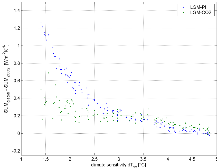
Fig. 5.22: Difference in the feedback behaviour between the 2\times\text{CO}_2 experiment and the glacial experiments. Shown is the difference in the aggregate mean feedback strength (SUM) between the experiments LGM-PI and 2\times\text{CO}_2 (blue dots) and between LGM-CO 2 and 2\times\text{CO}_2 (green dots) for each model version from the correlated parameter ensemble (only pre-industrial consistent model members). The climate sensitivity (abscissa) of a given model version represents the change in equilibrium surface temperature inferred from a doubling of \text{CO}_2 from 280 p.p.m. to 560 p.p.m.
