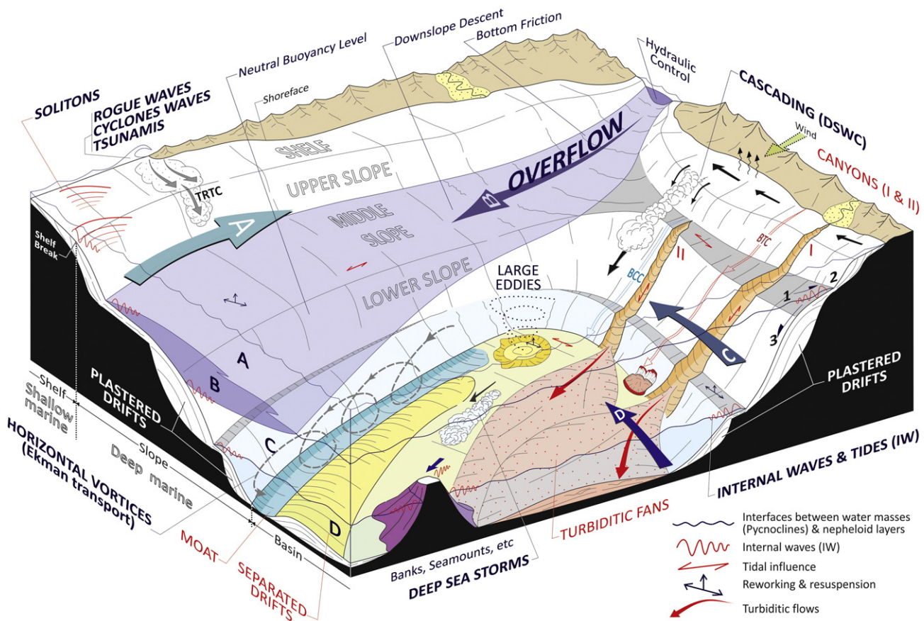
Fig. 1. 3D sketch depicting the possible oceanographic processes in deep-water environments. In addition to density currents and overflows, the velocity at the seafloor can also be affected by barotropic currents or intermittent processes like cascading, giant eddies, deep sea storms, vortices, internal waves, internal tides, tsunamis, cyclone waves and rogue waves. (From Rebesco et al., 2014, with permission from Elsevier).
