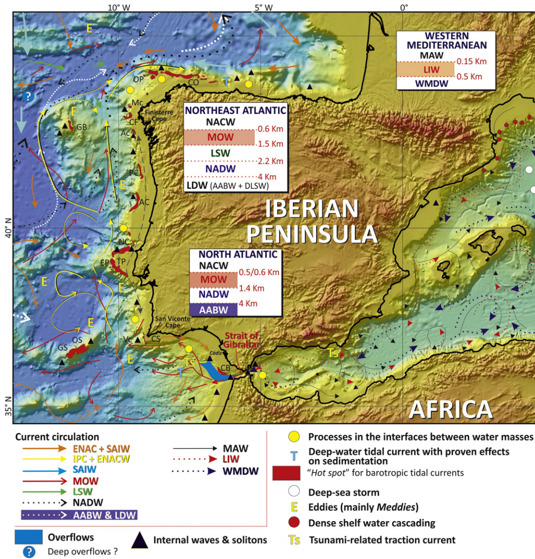
Fig. 19. Sketch summarizing the locations of permanent or intermittent oceanographic processes along the Iberian margins and their short- and long-term controls on sedimentary facies and seafloor morphology. These processes include overflows, barotropic currents, tides, eddies, deep-sea storms, horizontal vortices, internal waves, tsunamis, rogue waves and cyclonic waves. In one particular area, one of these processes may be dominant, but usually several processes act in tandem to determine the local direction and velocity of bottom currents. Legend for the Internal tide generation “hotspots”: AC = Arosa canyon; AV = Aveiro canyon; CB = Conil-Barbate; CF = cape of Finisterra; CS = cape of Sagres; CO = cape of Ortegal; EC = Estremadura promontory; GB = Galician bank; GS = Gettysburg seamount; MC = Murgia Canyon; NC = Nazaré canyon; OP = Ortegal promontory; OS = Ormonde seamount; PC = Porto canyon; TP = Tagus Plateau; VC = S. Vicente canyon. Legend for water masses by alphabetic order: AABW = Antarctic Bottom Water; ENAC = Eastern North Atlantic Current; ENACW = Eastern North Atlantic Central Water; IPC = Iberian Poleward Current; LDW = Lower Deep Water; LIW = Levantine Intermediate Water; LSW = Labrador Sea Water LSW; MAW = Modified Atlantic Water; MOW = Mediterranean Outflow Water; NADW = North Atlantic Deep Water; NASW = North Atlantic Superficial Water; SAIW = Subarctic Intermediate Water; WMDW = Western Mediterranean Deep Water.
