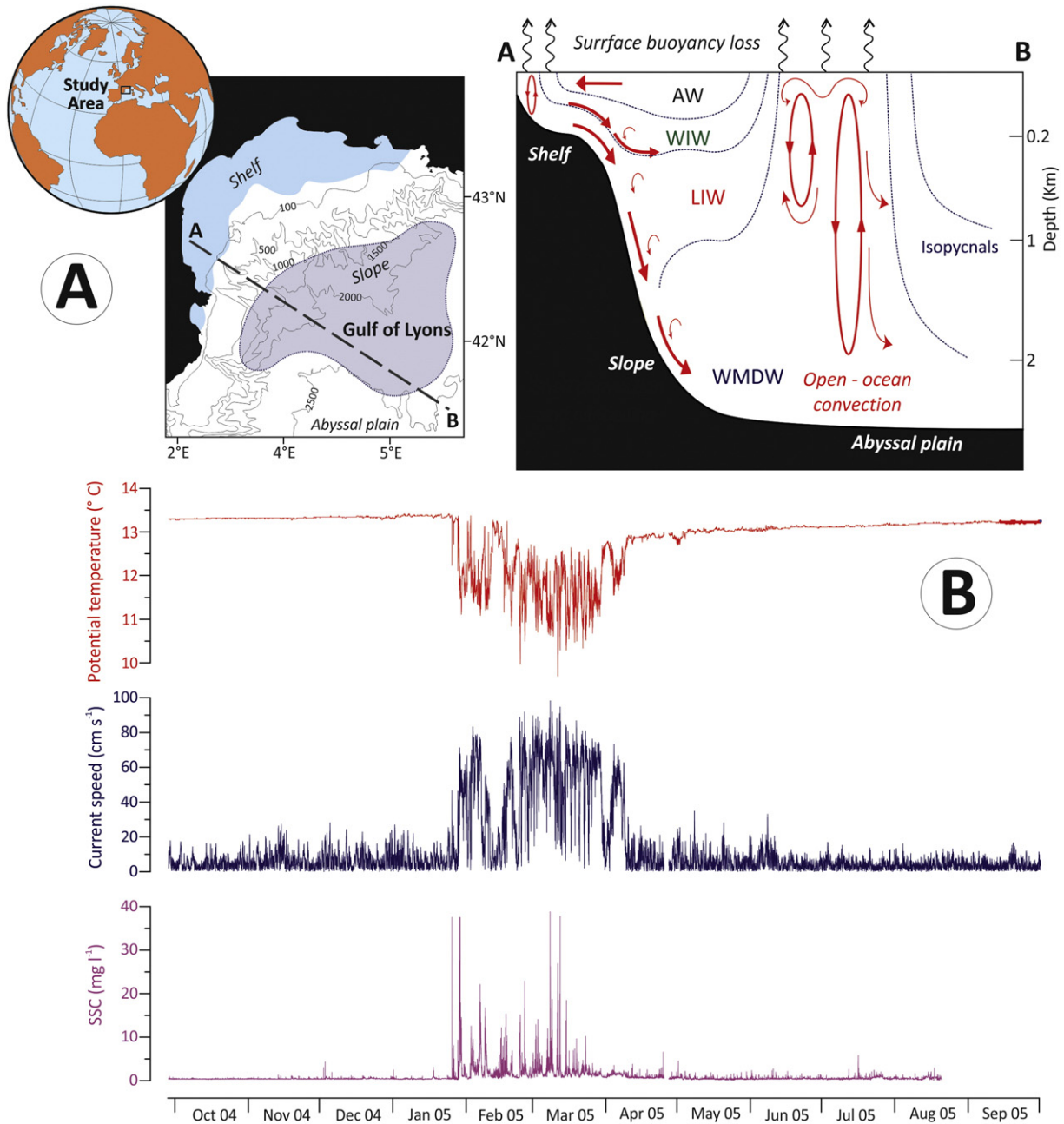
Fig. 11. A) Map of the Gulf of Lions area showing the regions of dense water formation and distribution (adapted from Puig et al., 2013). B) A dense shelf water cascading (DSWC) event in the Gulf of Lions' shelf illustrated by a time series of near-bottom potential temperature, current speed and suspended sediment concentration (SSC) recorded at 500 m depth (5 m above bottom) in the axis of Cap de Creus Canyon during the winter 2004–05. Adapted from Puig et al. (2008). Legend for water masses by alphabetic order: AW = Atlantic Water; LIW = Levantine Intermediate Water; WIW = Western Mediterranean Intermediate Water; WMDW = Western Mediterranean Deep Water.
