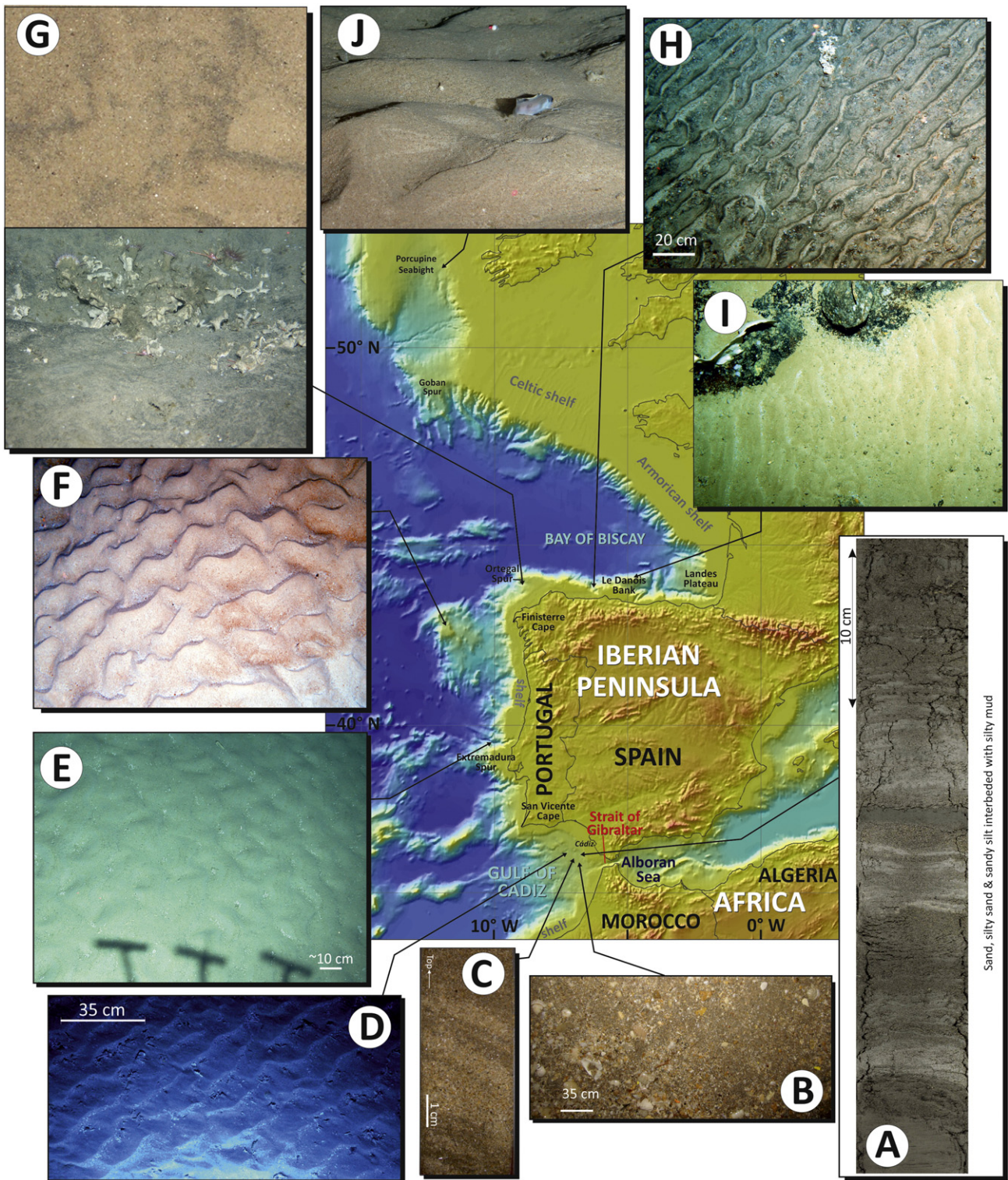
Fig. 17. Examples of deep water sandy deposits around the Iberian margins. Some of them are related to the action of contour currents, but other are related to other oceanographic processes as internal waves, tides, etc. Most of these deposits have not been studied yet and future work should clarify their characteristics and genesis. A) Examples of sandy contourite facies sampled during IODP Expedition 339, in the Gulf of Cadiz close to the exit of the Strait of Gibraltar (Modified from Hernández-Molina et al., 2014); B) coarse sands and bioclastic gravel deposits in the slope of the Gulf of Cadiz at the exit of the Strait of Gibraltar collected with the CONTOURIBER Project (2010); C) laminated sandy contourite facies, showing inclined lamination as a result of sand wave migration in the Gulf of Cadiz sand sheet in proximal sector (Stow and Faugères, 2008); D) contourite sandy deposits affected by bottom current and barotropic and internal tides in the slope channels of the middle slope of the Gulf of Cadiz (from Stow et al., 2013a); E) sandy turbiditic (reworked?) facies from ISIS from ca. 4300 m water depth in the Nazare Canyon (courtesy from V. Huvenne of NOCS, UK); F) sandy deposits on top of the Galicia Bank by bottom current (INDEMARES Project, Photo taken by F. Sánchez, IEO, Spain); G) example of sandy deposits from the middle slope of the Ortegale Spur (From A Selva Cruise, 2008 and R/V Belgica 09/14a cruise, EC FP7 IP HERMIONE project); H) submarine photographs of reworked sandy deposits within the Gaviera canyon, Cantabrian Sea (Photo taken by F. Sánchez, IEO, Spain); I) sandy deposits along the SE flank of the Le Danois Bank in the slope of the Cantabrian Sea (ECOMARG 3 Project, Photo taken by F. Sánchez, IEO, Spain); and J) sandy deposits in the Porcupine seabight, Irish continental slope (courtesy of MARUM, Germany).
