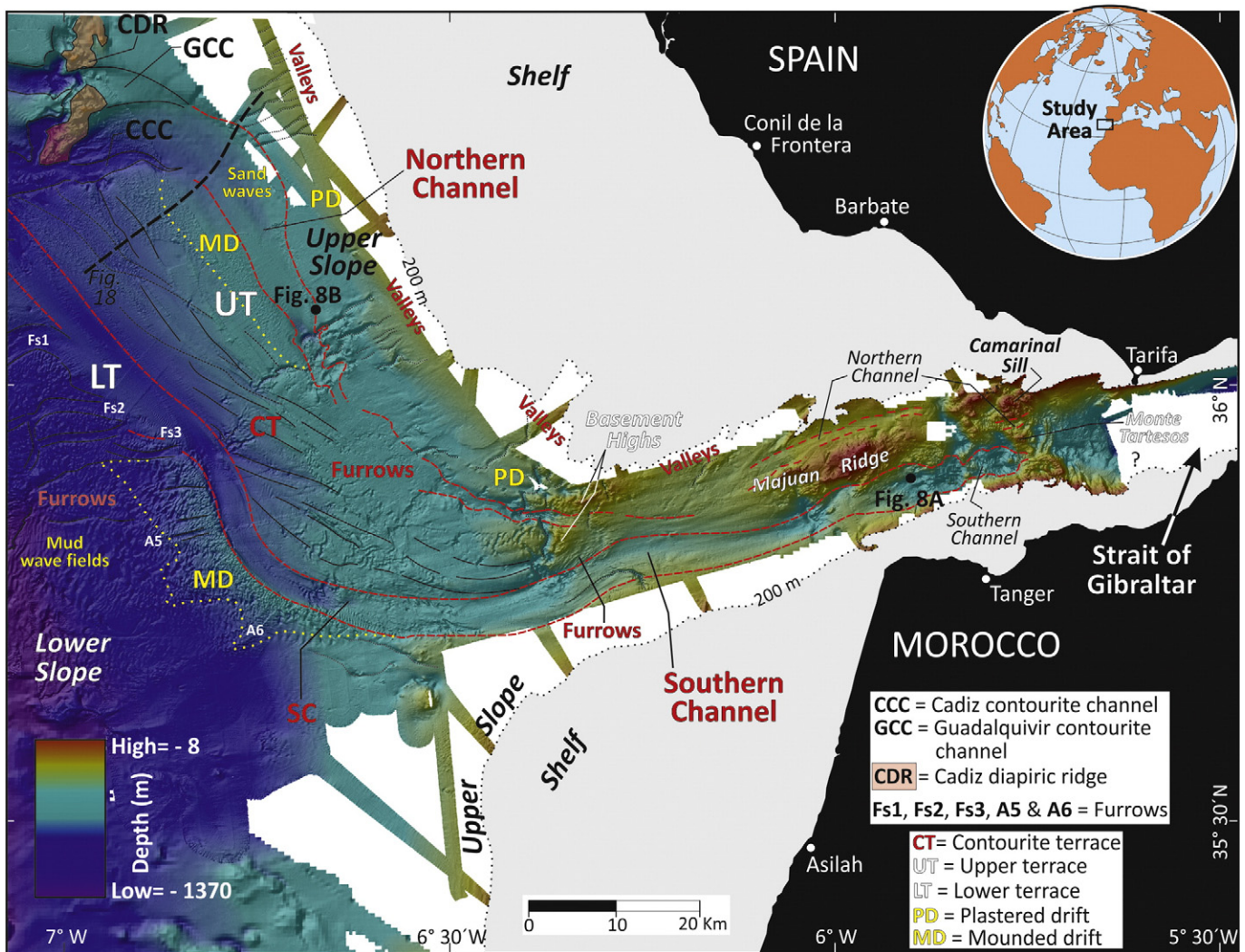
Fig. 2. Swath bathymetry at the exit of the Strait of Gibraltar. Main depositional and erosive features are shown (from Hernández-Molina et al., 2014 with permission from GSA). Note that furrows are oblique to the main channels due to the secondary circulation related to the benthic Ekman transport.
