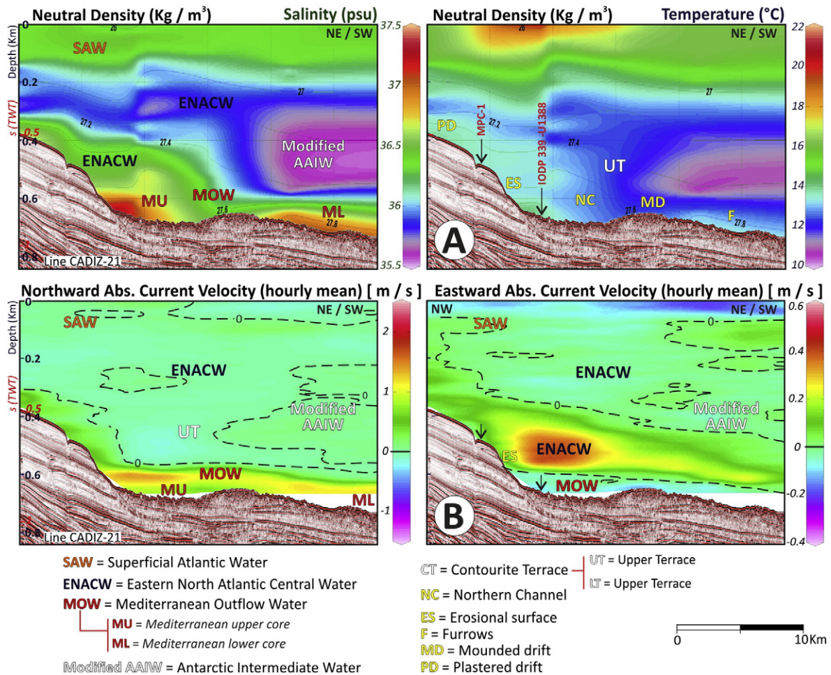
Fig. 18. Examples of combination of physical oceanographic and geologic/geophysical data showing the relationship between the long-term current regime, seafloor morphology and sub-bottom sediment geometry in the Gulf of Cádiz, from the exit of the Strait of Gibraltar (Hernández-Molina et al., 2014, with permission from Geological Society of America). A) Salinity and temperature data in the water columns. The black lines refer to isopycnals and neutral density ( \text{kg}/\text{m}^3 ); B) vertical sections of ocean velocity measured at the eastern area close to the exit of the Strait of Gibraltar. The water colour code displays the Acoustic Doppler Current Profiler (ADCP) velocity components. The panels on the left correspond to the velocity component in the east–west direction (positive values indicate currents towards the east), and the panels on the right correspond to the velocity component in the north–south direction (positive values indicate current towards the north). The dashed black lines indicate where the current velocity is zero. See Fig. 2 for section locations.
