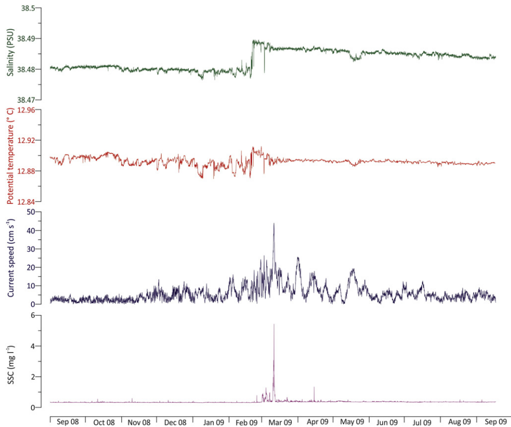
Fig. 9. Time series observations of near-bottom salinity, potential temperature, current speed and suspended sediment concentration (SSC) recorded at the Catalan continental rise (1890 m in depth), illustrating an example of a benthic storm occurring in the northwestern Mediterranean basin after the winter 2009 deep dense water formation event. Note the sharp increase of salinity and temperature associated to the arrival of the dense waters to the basin and the subsequent increase of near-bottom velocities with a peak >40 cm/s that caused resuspension of bottom sediments (modified from Puig et al., 2012).
