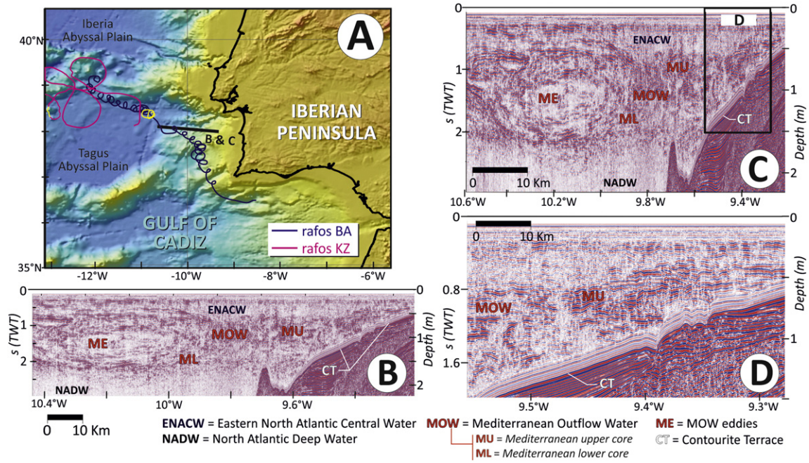
Fig. 5. A) Bathymetric map of the west Iberian margin, showing the trajectories of the RAFOS floats that were caught by Meddy-9 (blue line) and the cyclone C (magenta line) reported from Pinheiro et al. (2010); the yellow fractions of these trajectories correspond to the period between the 28th of August and the 3rd of September 1993, during which the seismic profile in B and C was acquired. B and C) Complete migrated seismic section showing the eddies (meddies) related to the Mediterranean Outflow Water (MOW) and their interaction with the seafloor (Pinheiro et al., 2010), including the water masses and the interaction of MOW with a contourite terrace in the middle slope. The segment to the East of the line was acquired from W to E, from the 2nd till the 3rd of September 1993. Approximate depth based on 1500 m/s sound speed, and longitude axis are indicated; C) Detail of a migrated section with interpreted upper (MU) and lower (ML) MOW (Pinheiro et al., 2010); and D) detail of a migrated section with the interpreted upper MU (Pinheiro et al., 2010). High amplitude reflections within the profiles, especially to the upper and lower boundaries of MOW and meddies are indicative of density contrast surfaces in the water column.
