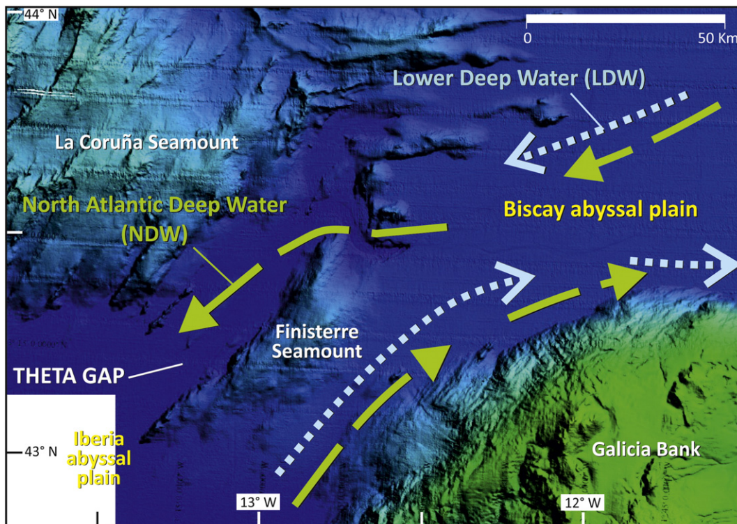
Fig. 3. Main morphologic features around the Theta Gap showing the regional water mass circulation.
