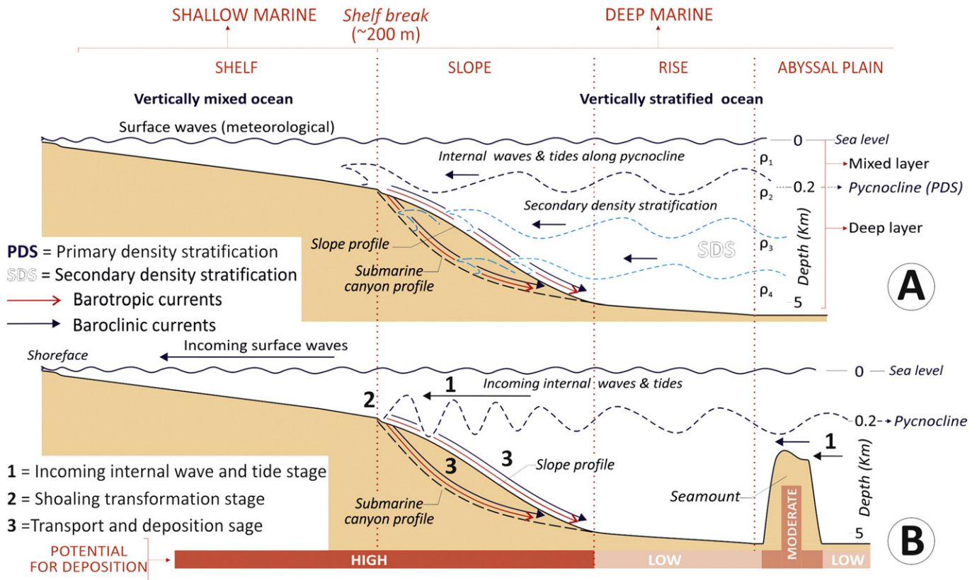
Fig. 12. A) Schematic diagram showing the position of the pycnocline (i.e., primary density stratification), where density gradient is the sharpest, between mixed (upper) and deep (lower) ocean layers of different densities (adapted from Shanmugam, 2013b). Internal waves and tides propagate along the boundaries of both primary and secondary density stratifications. Internal waves and astronomical internal tides propagate along the boundaries of density stratification in deep-marine environments. Barotropic currents (red arrow) are generated by surface waves and tides, whereas baroclinic currents (dark blue arrow) are generated by internal waves and tides; B) conceptual oceanographic and sedimentologic framework showing deposition from baroclinic currents on continental slopes, in submarine canyons, and on guyots. On continental slopes and in submarine canyons, deposition occurs in three progressive stages: (1) incoming internal wave and tide stage, (2) shoaling transformation stage, and (3) sediment transport and deposition stage. Continental slopes and submarine canyons are considered to be environments with high potential for deposition from baroclinic currents. In the open ocean, baroclinic currents can rework sediments on flat tops of towering guyot terraces, without the need for the three stages required for the deposition on continental slopes (From Shanmugam, 2012a, 2012b, 2013b).
