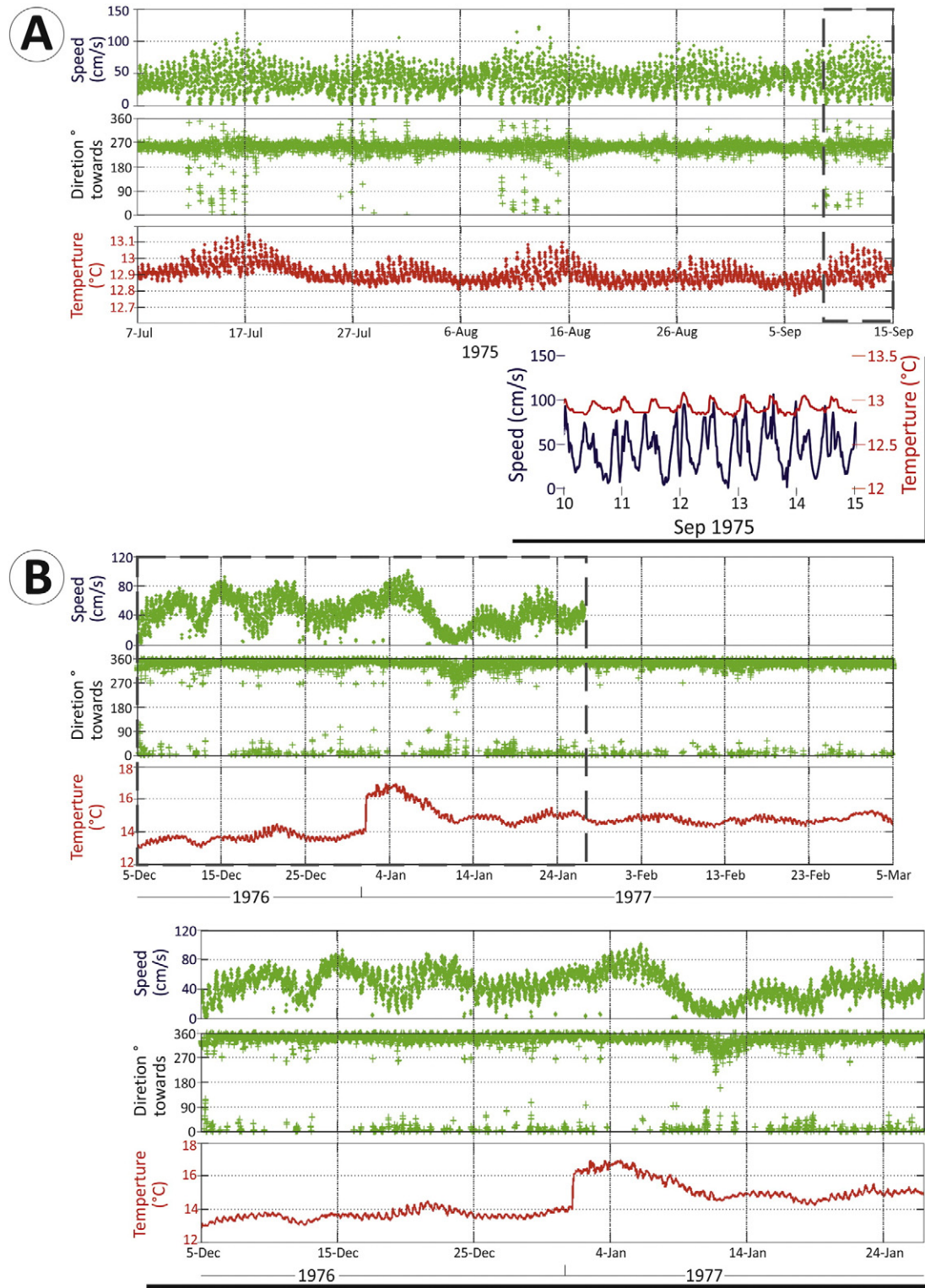
Fig. 8. Time series observations of the near-bottom current (78 m above the seafloor) at the Exit of the Strait of Gibraltar (A) for 79 days at 472 m water depth and at the eastern Gulf of Cadiz (B) for 97 days at 554 m water depth (see location in Fig. 2), showing a strongly directional MOW towards the WSW (A) and NNW (B) with speeds up to 1 m/s. A detail in (A) is illustrating the relation between the current speeds and temperature from 10 to 14 September of 1975. Inset in B depicts a semi-diurnal tidal periodicity with a spring-neap tidal cycle is clearly observed, which also modulates the near-bottom temperature. The jump in the temperature record in B is presumably due to the mooring turn-around operation and the sampling of a slightly different water parcel after its redeployment. Published with permission from British Oceanographic Data Center (BODC) and National Oceanographic Centre, Southampton (NOCS).
