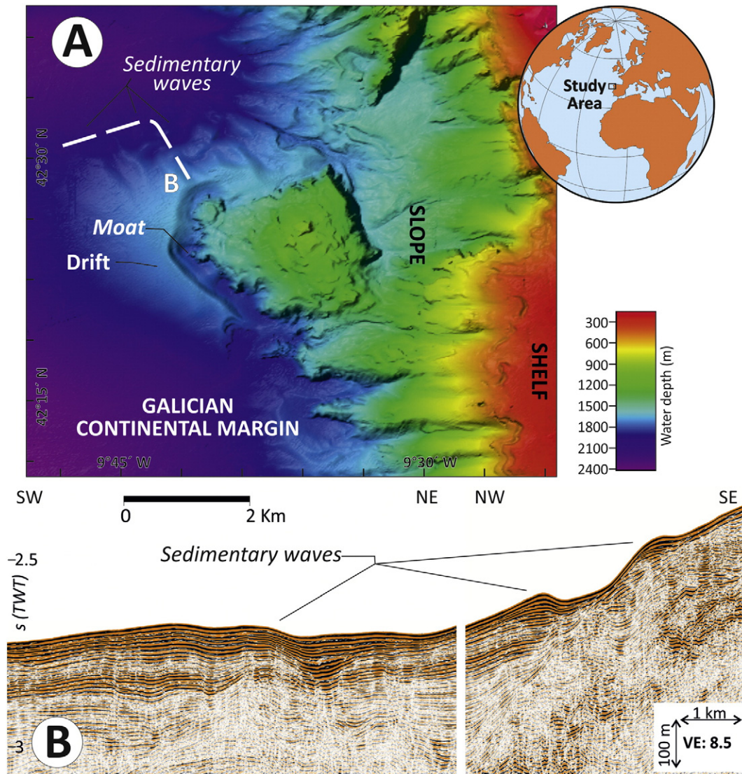
Fig. 14. Example of sedimentary waves in the Galician continental margin, which could be attributed to internal waves. A) Swath bathymetric map of the margin indicating the position of the sedimentary waves along the NW flank of a contourite drift in the lower slope; B) Seismic profile across the sediment waves (data courtesy from the MARUM project GALIOMAR, from Hanebuth et al., 2012).
