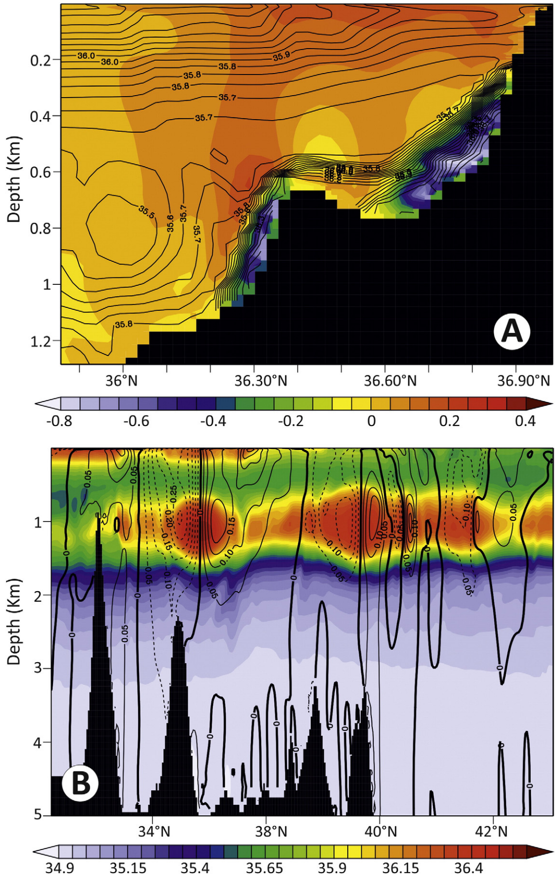
Fig. 10. A) A snapshot of simulated zonal component of velocity and salinity at 7.5°W showing the MOW undercurrents flowing westwards in the Gulf of Cadiz; B) Snapshot of simulated salinity and zonal component of velocity at 13°W, showing the large vertical extension of the velocity signal associated with the MOW eddies (meddies) downstream of Portimao Canyon (from Serra et al., 2010a).
