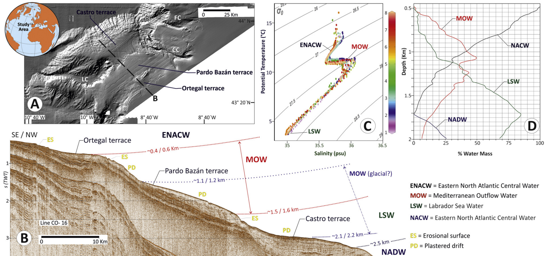
Fig. 4. Example of three contourite terraces (Ortegal, Pardo Bazán and Castro) along the continental slope northwest of Galicia and its relation with the interfaces between water masses. A) Multibeam bathymetry indicating the position of the terraces at water depths around 0.2–0.4 km; 0.9–2 km and 2.2–2.4 km (adapted from Maestro et al., 2013 ); B) seismic profile (CO-16) acquired during the CONTOURIBER-2 Cruise crossing the terraces (line position in A). Interfaces between regional water masses at present time is included, with the theoretical position of MOW during glacial stages (in blue); C) T/S diagram corresponding to eight profiles from ARGOS buoy (6900469, PROVOR Profiling Float CTS3- OVIDE Project) between the 9.11.2012 to 18.01.2013 (from Sánchez González, 2013 ); D) Water masses percentage in the adjacent area to the contourite terraces (from Sánchez González, 2013 ).
