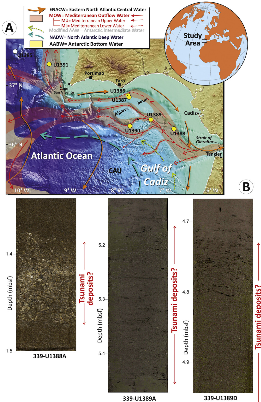
Fig. 16. A) Regional water masses and Gulf of Cádiz CDS site locations sampled during IODP Expedition 339; B) Sandy Holocene deposits drilled during IODP Expedition 339 (Sites U1388 and U1389) interpreted as tsunami deposits (Stow et al., 2013b, Pers. Comm., Yasuhiro Takashimizu, Niigata University, Japan).
