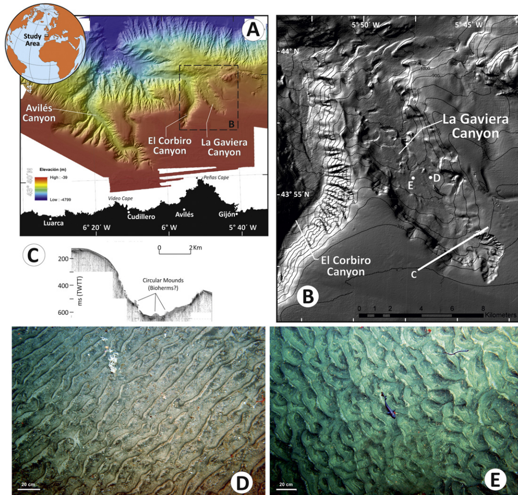
Fig. 15. Examples of sandy bedforms related to internal tides and waves within the Gaviera Canyon, in the Cantabrian margin. A) Regional area location; B) Shaded bathymetric map of part of the Cantabrian Sea margin (isobaths equidistance 100 m) indicating the position of the major canyons, with illumination from the NW (Gómez-Ballesteros et al., 2014). C) Topas profile crossing NE the head of the Gaviera canyon (Gómez-Ballesteros et al., 2014). Submarine photographs of the Gaviera canyon seafloor; D) at 863 m water depth ( -5.78628/43.92902 ) taken the 24 April 2010 at 15:05. Water temperature was about 9.93\text{ }^{\circ}\text{C} ; salinity of 35.76 and potential density of 27.54\text{ kg/m}^3 ; E) at 837.6 m water depth ( -5.77847\text{E}/43.93003\text{N} ) taken the 26 April 2010 at 15:41. Water temperature was about 9.95\text{ }^{\circ}\text{C} ; salinity of 35.75 and potential density of 27.53\text{ kg/m}^3 (Photo taken by F. Sánchez, IEO).
