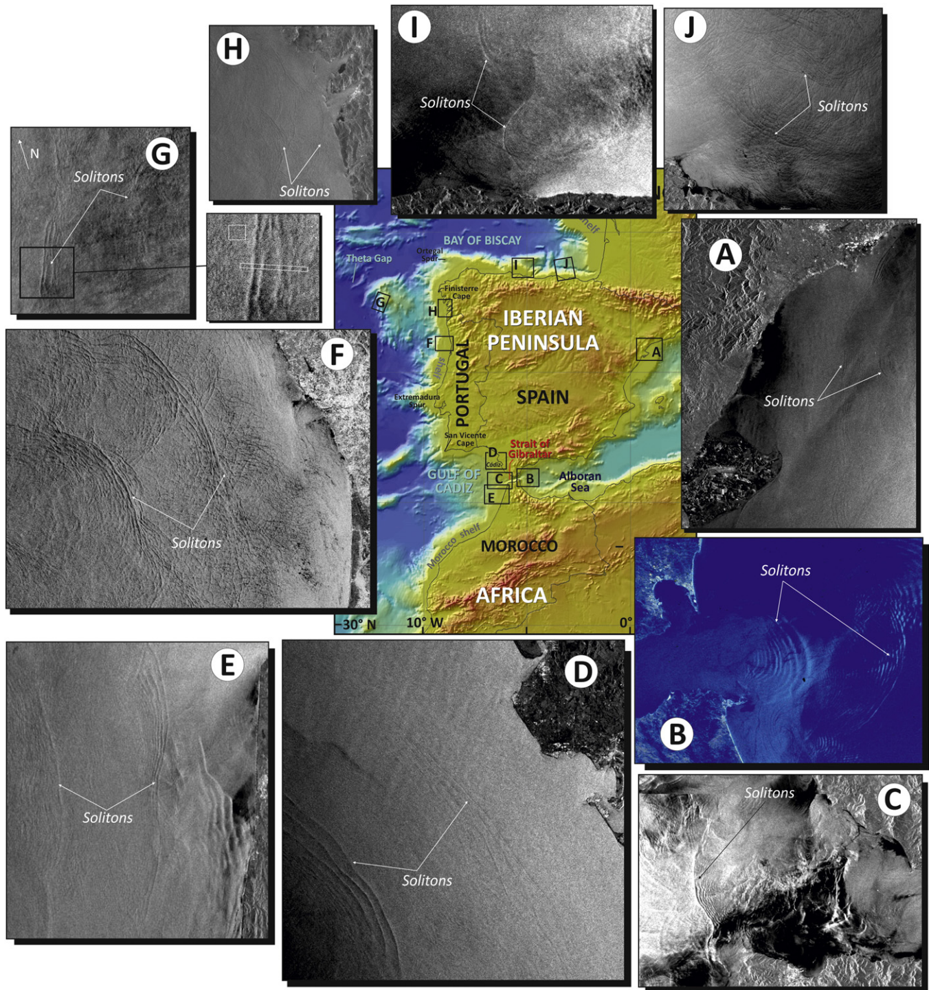
Fig. 13. Selected examples of internal solitons propagating towards the continental slope and shelf around the Iberian margins from: A) Catalanian margin; B) East of the Strait of Gibraltar; C) West of the Strait of Gibraltar; D) Cádiz; E) NW Morocco; F) NW Portugal; G) Galicia Bank; H) Rias Baixas (Galicia margin); I) Cantabrian margin (off Gijón); J) Cantabrian margin (off Bilbao). These oceanographic processes are ubiquitous around Iberia as well as in the adjacent continental margins from Morocco, France and Porcupine related mainly to the shelf break, seamounts and banks. Their real implications in sedimentary processes have not been considered until now although they represent energetic and constant oceanographic processes. Images are synthetic aperture radar images [from Apel, 2004 and EOLi (Earth Observation Link, European Space Agency, http://earth.esa.int/EOLi/EOLi.html )].
