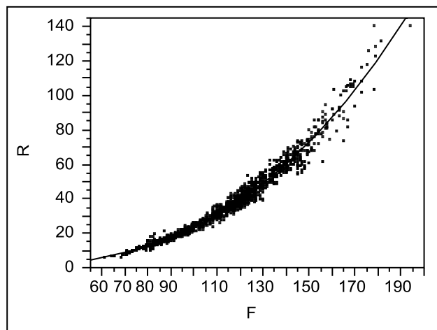
Figure 5. Plot of the non-linear fit between the round weight (RW kg) by size (FL cm) -see table 3 for additional information-: RW = 6.0568E^{-05} * FL^{2.793790} .
