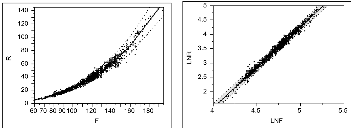
Figure 2. Bivariate lineal fit of the round weight (RW kg) by size (FL cm) –left panel- and bivariate fit of the Ln (RW) by Ln (FL) –right panel-, and 95% confidence intervals of the observations.
