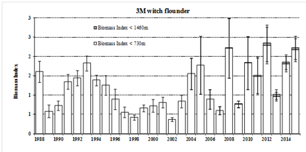
Fig.3. Biomass of 3M witch flounder is available from the EU-Flemish Cap survey in Division 3M
