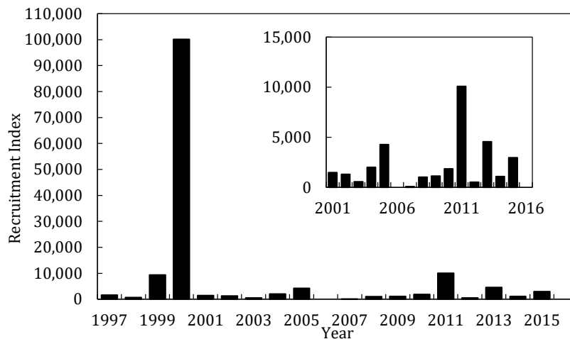
Fig. 17.4. White Hake in Div. 3NO and Subdiv. 3Ps: recruitment index for Age 1 males and females(combined) from Canadian Campelen spring surveys in Divs. 3NO and Subdiv. 3Ps n 1997-2015. Estimates from 2006 are not shown, since survey coverage in that year was incomplete. Inset plot depicts 2001-2015 on a smaller scale.
