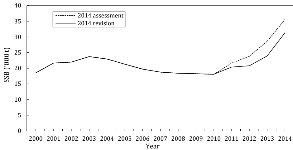
Fig. 11.9. American plaice in Div. 3LNO: comparison of spawning stock biomass estimates from 2014 and those estimates calculated using revised stock weights.
