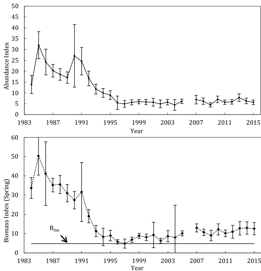
Fig. 16.2b. Thorny Skate in Divs. 3LN0 and Subdiv. 3Ps: abundance (top panel) and biomass (bottom panel) indices from Canadian spring surveys: 1984-2015.
