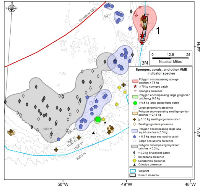
Fig.4. Location of significant concentrations of large sea squirts (encompassed by purple polygons) and erect bryozoans (encompassed by grey polygons) on the Tail of Grand Bank (Figure from NAFO, 2014).
