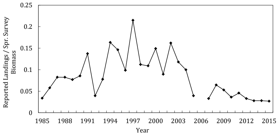
Fig. 16.7. Thorny skate in Divs. 3LNOPs:: estimates of Relative F from STACFIS-agreed commercial landings/Canadian spring survey biomass.
