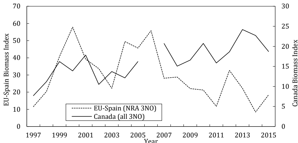
Fig. 16.4. Thorny skate in Divs. 3LNOPs: biomass indices from the EU-Spain survey and the Canadian spring survey in 1997-2015.
