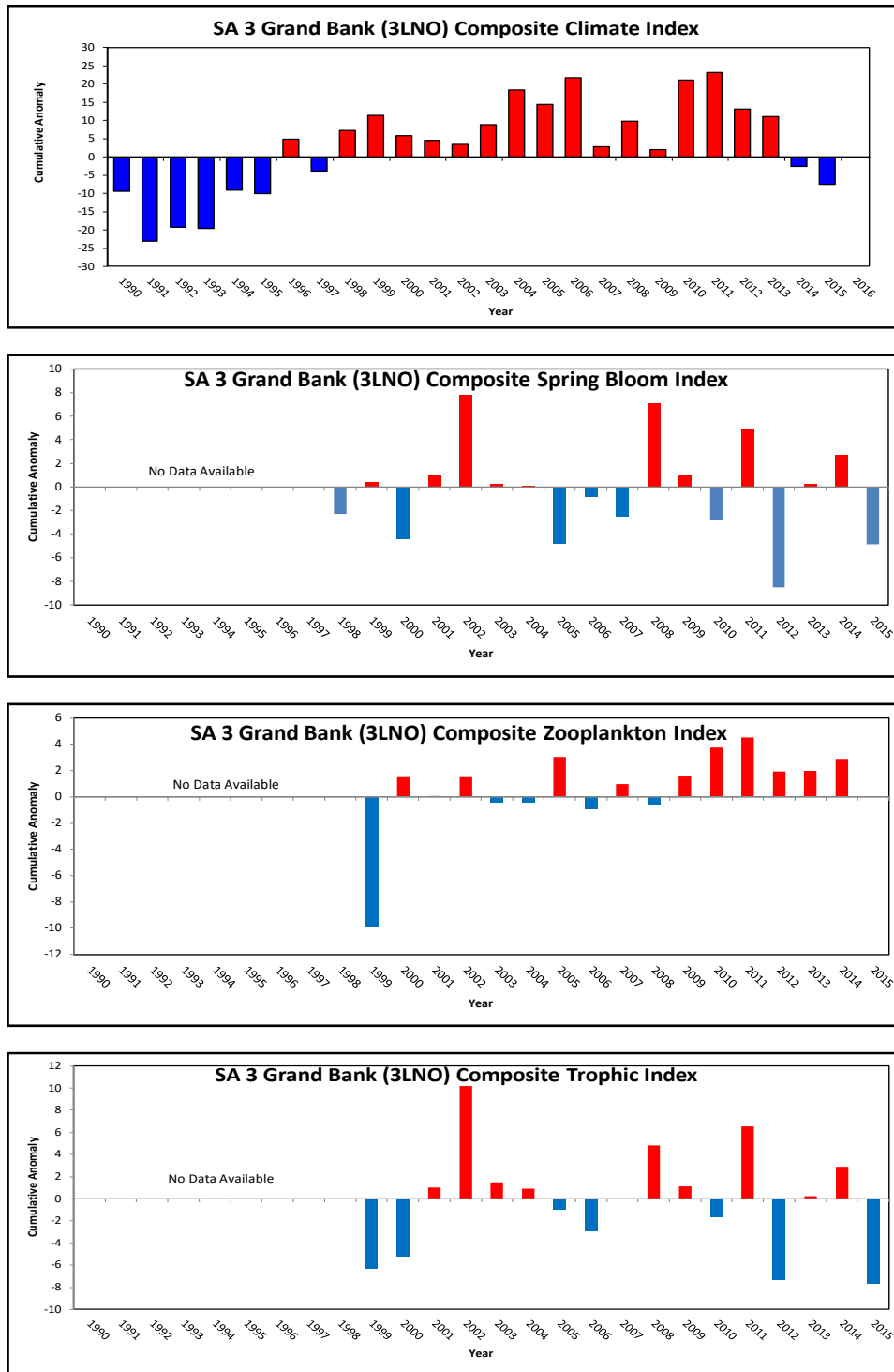
Fig. III.3. Composite ocean climate index for NAFO Subarea 3 (SA3 Divs. 3LNO) derived by summing the standardized anomalies (top panel) during 1990-2015, composite spring bloom (cumulative anomalies for magnitude and timing metrics of the spring bloom) index (Divs. 3LNO) during 1998-2015 (2 nd panel), composite zooplankton (summed functional plankton groups) index during 1999-2015 (3 rd panel), and composite trophic (summed nutrient and standing stocks of phyto- and zooplankton indices) index (bottom panel) during 1999-2015. Red bars are positive anomalies indicating above average levels while blue bars are negative anomalies indicating below average values.
