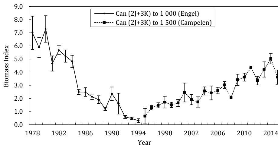
Fig. 18.2. Roughhead grenadier in Subareas 2+3: biomass indices (+/- SE) from the Canadian autumn (Div. 2J3K) survey.
