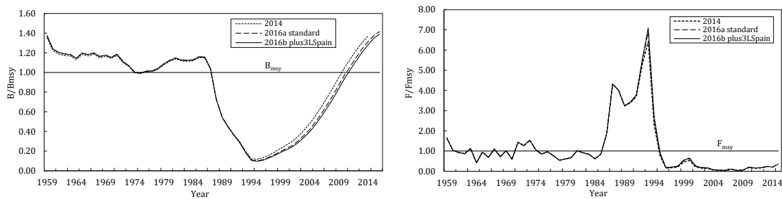
Fig. 10.4. Redfish in Divs. 3LN: B / B msy and F / F msy from ASPIC fit 2014 versus ASPIC fit 2016a and ASPIC fit 2016b assessments.
