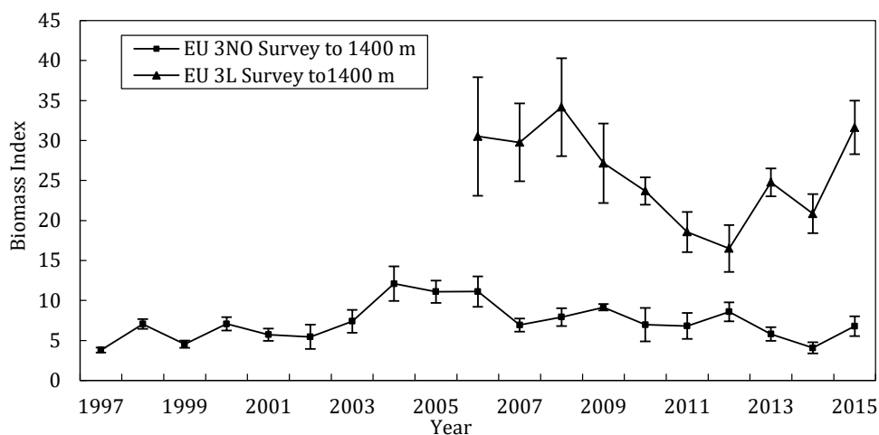
Fig. 18.5. Roughhead grenadier in Subareas 2+3: biomass indices (+/. SE) from the EU-Spanish Div. 3NO and 3L surveys.
