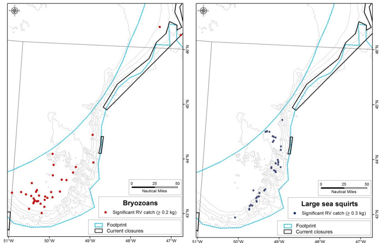
Fig.5. Left panel. Location of significant catches of bryozoans (above the 0.2 kg threshold). Right panel. Location of significant catches of large sea squirts (above the 0.3 kg threshold).
