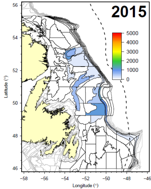
Fig. 19.3. Witch flounder in Divs. 2J+3KL : spatial distribution of biomass index from the Canadian survey during autumn 2015.
