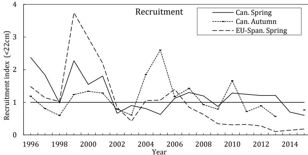
Fig.12.4. Yellowtail flounder in Div. 3LNO: Juvenile abundance indices from spring and autumn surveys by Canada (Can.) and spring surveys by EU-Spain. Each series is scaled to its mean (horizontal line).
