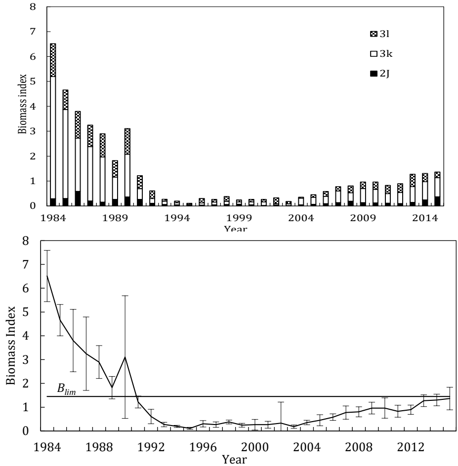
Fig. 19.2. Witch flounder in Divs. 2J+3KL : Index of biomass from Canadian autumn surveys by Division (top panel) and overall (bottom panel with 95 % confidence limits). Values are Campelen units or, prior to 1995, Campelen equivalent units.
