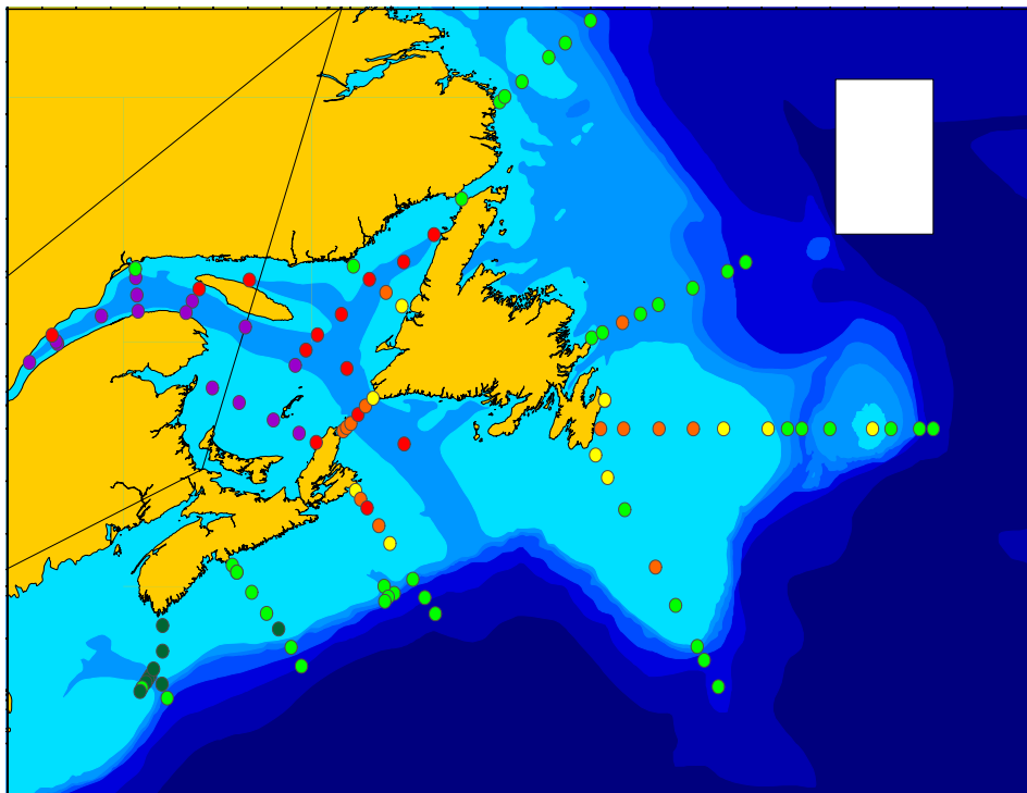
Fig. 1. Near bottom Aragonite saturation state determined during the AZMP Fall 2014 Oceanographic surveys (samples collected between 19 September and 7 December 2014).
