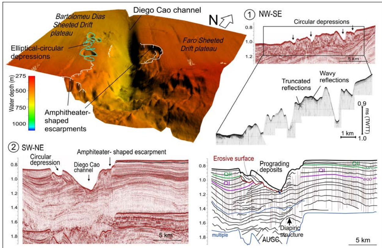
Fig. 2. 3D view of the Diego Cao channel showing the elliptical-circular depressions and amphitheater-shaped escarpments. Seismic profiles (Parasound and Airgun) reveal the main morphological and seismic characteristics.
