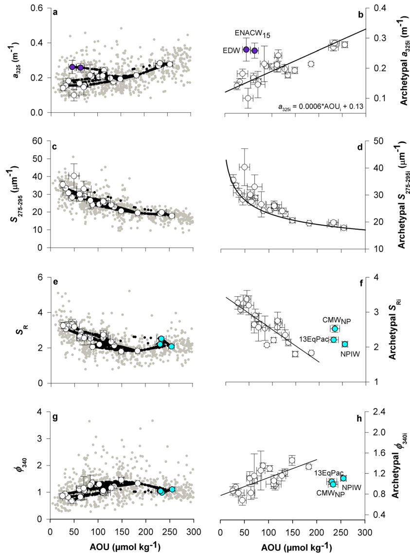
Figure 5. Relationships between the CDOM parameters (a) a_{325} , ( m^{-1} ), (c) S_{275-295} ( \mu m^{-1} ), (e) S_R (unitless), and (g) \phi_{340} (%) with apparent oxygen utilization (AOU, \mu mol kg^{-1} ) in the global dark ocean. In Figures 5a, 5c, 5e, and 5g, measured concentrations (gray dots), archetypal concentrations for each water type (white dots), and archetypal concentrations for each sample (black dots) are presented. Figures 5b, 5d, 5f, and 5h show the relationship between archetypal concentrations of the WT for each studied variable. We obtained the following functions: (b) a_{325i} = 6 (\pm 1) \times 10^{-4} AOU_i + 0.13 (\pm 0.01) , R^2 = 0.76 ( p < 0.001 , n = 20 ); (d) S_{275-295i} = 0.037 (\pm 0.002) e^{-0.0032 (\pm 0.0004) AOU_i} , R^2 = 0.82 ( p < 0.001 , n = 22 ); (f) S_{Ri} = -0.011 (\pm 0.002) AOU_i + 3.6 (\pm 0.1) , R^2 = 0.74 ( p < 0.001 , n = 19 ); (h) \phi_{340i} = 0.006 (\pm 0.003) AOU_i + 0.60 (\pm 0.08) , R^2 = 0.49 ( p = 0.001 , n = 19 ). Indigo and sky-blue dots were excluded from their respective regression models (see the text for justification).
