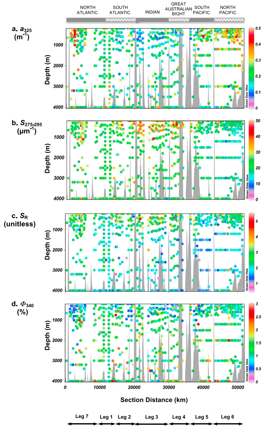
Figure 4. Distribution of (a) a_{325} ( m^{-1} ), (b) S_{275-295} ( \mu m^{-1} ), (c) S_R (unitless), and (d) \Phi_{340} (%) of the water samples intercepted during the Malaspina 2010 expedition. Note that the depth range starts at 200 m.
