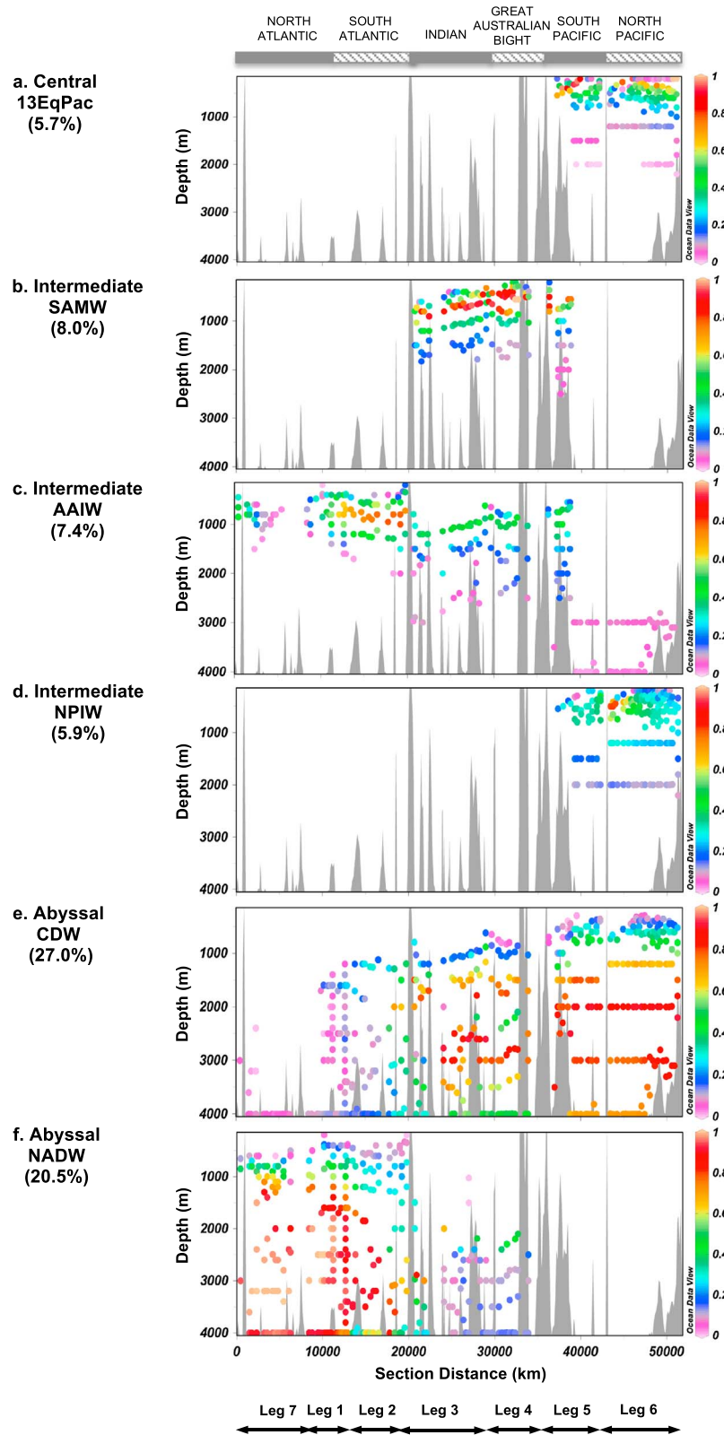
Figure 2. Distribution of the most representative water masses of the dark global ocean during the Malaspina 2010 circumnavigation: (a) Equatorial Pacific Central Water at 13 °C (13EqPac), (b) Sub-Antarctic Mode Water (SAMW), (c) Antarctic Intermediate Water (AAIW), (d) North Pacific Intermediate Water (NPIW), (e) Circumpolar Deep Water (CDW), and (f) North Atlantic Deep Water (NADW). Note that the proportion ranges from 0 (0%) to 1 (100%) and the depth range starts at 200 m.
