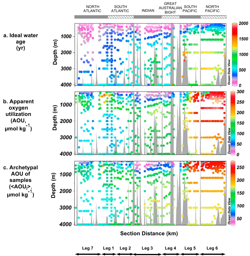
Figure 3. Distribution of (a) ideal water age ( \tau , years), (b) apparent oxygen utilization (AOU, \mu\text{mol kg}^{-1} ), and (c) archetypal apparent oxygen utilization ( \langle\text{AOU}_j\rangle , \mu\text{mol kg}^{-1} ) of the water samples intercepted during the Malaspina 2010 expedition. Note that the depth range starts at 200 m.
