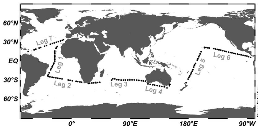
Figure 1. Cruise track of the Malaspina 2010 circumnavigation on board the Spanish R/V Hespérides from 16 December 2010 to 11 July 2011.
