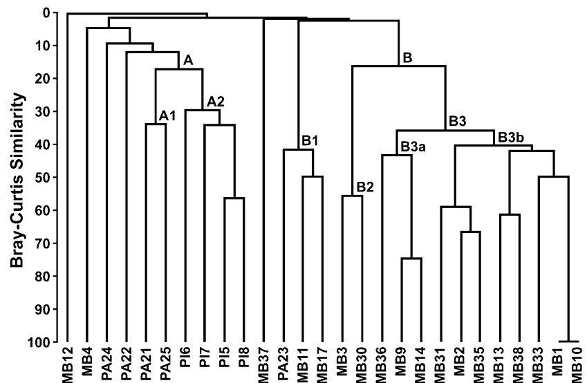
Fig. 3 Faunistic assemblages in the study are determined by cluster analysis based on Bray-Curtis Similarity.
