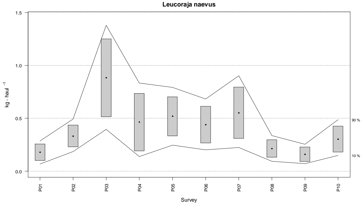
Figure 21. Changes in Leucoraja naevus biomass index ( \text{kg} \cdot \text{haul}^{-1} ) during Porcupine survey time series (2001-2010). Boxes mark parametric standard error of the stratified biomass index. Lines mark bootstrap confidence intervals ( \alpha = 0.80 , bootstrap iterations = 1000).
