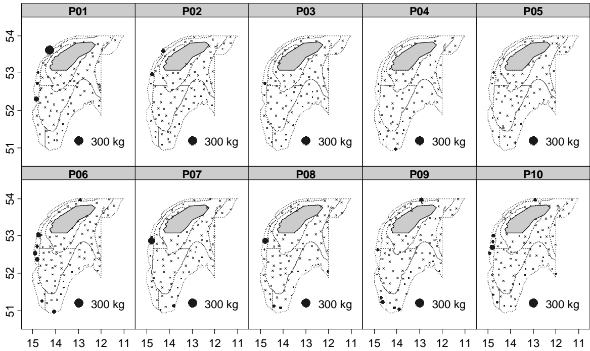
Figure 7. Geographic distribution of birdbeak dogfish ( D. calcea ) catches ( \text{kg}\cdot\text{haul}^{-1} ) during Porcupine survey time series (2001-2010).
