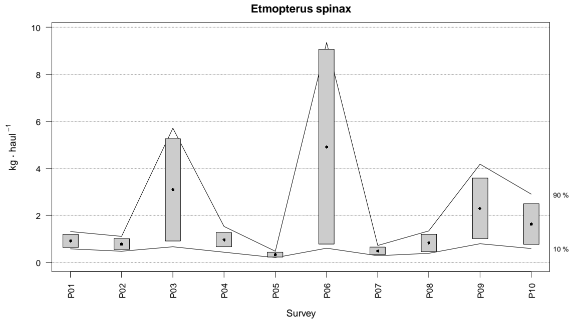
Figure 9. Changes in velvet belly ( Etmopterus spinax ) biomass index (kg · haul -1 ) during Porcupine survey time series (2001-2010). Boxes mark parametric standard error of the stratified biomass index. Lines mark bootstrap confidence intervals ( \alpha = 0.80 , bootstrap iterations = 1000).
