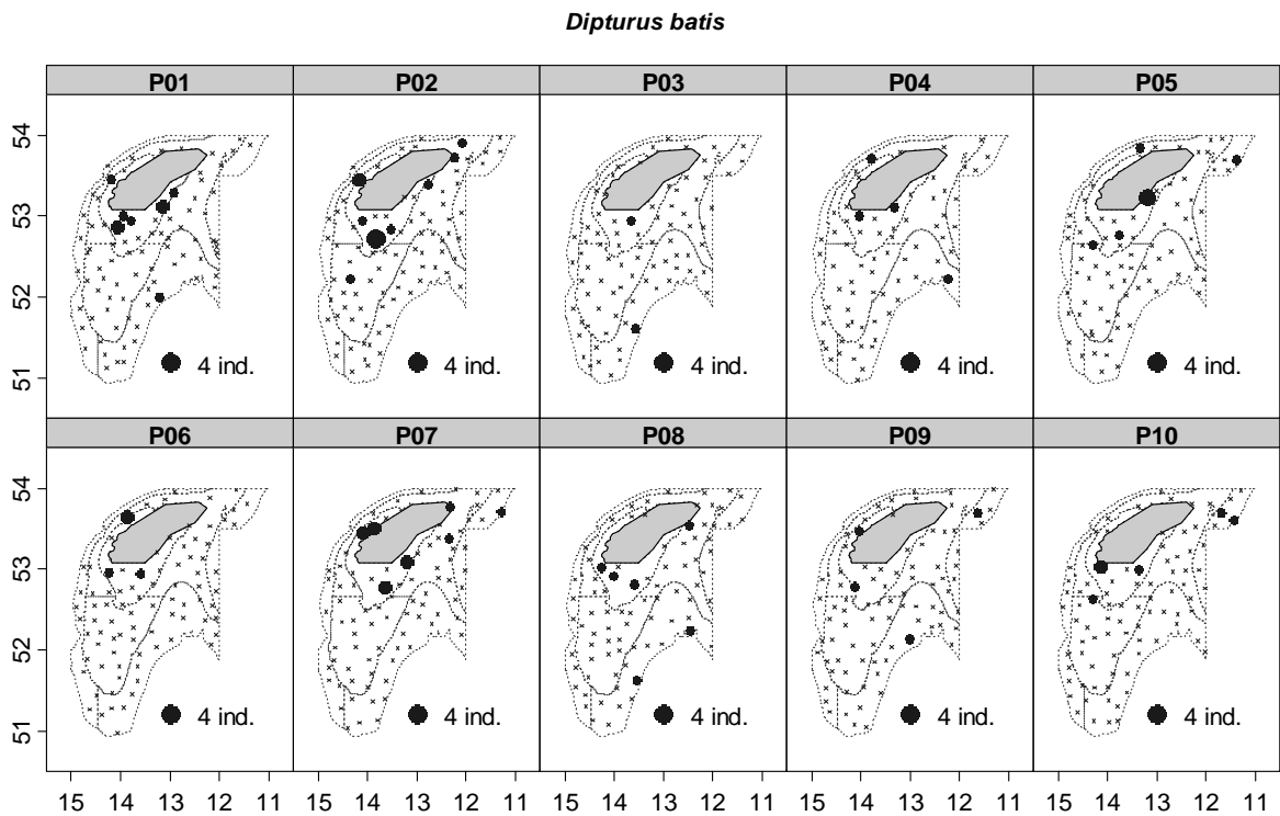
Figure 28. Geographic distribution of common skate ( D. batis ) catches ( \text{ind} \cdot \text{haul}^{-1} ) in Porcupine survey time series (2001-2010).
