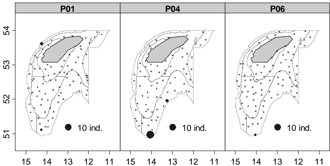
Figure 30. Geographic distribution of Siki shark catches (ind.·haul -1 ) in Porcupine bank surveys (2001-2010). These years shown above were the only three ones with catches out of the historical series.
