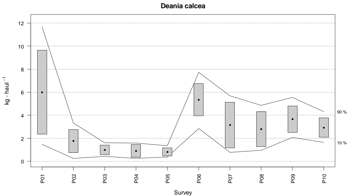
Figure 6. Changes in birdbeak dogfish ( Deania calcea ) biomass index ( \text{kg}\cdot\text{haul}^{-1} ) during Porcupine survey time series (2001-2010). Boxes mark parametric standard error of the stratified biomass index. Lines mark bootstrap confidence intervals ( \alpha = 0.80 , bootstrap iterations = 1000).
