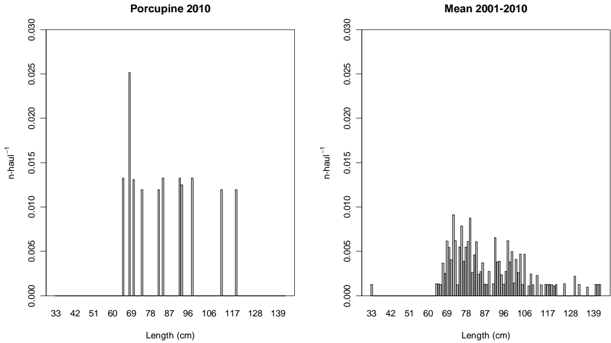
Figure 19. Stratified length distributions of bluntnose sixgill shark ( H. griseus ) in 2010 Porcupine survey and mean values during Porcupine survey time series (2001-2010).
