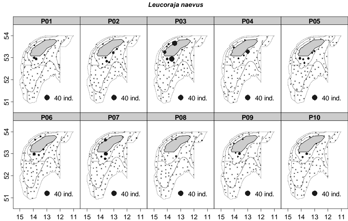
Figure 23. Geographic distribution of Leucoraja naevus catches (ind · haul -1 ) during Porcupine survey time series (2001-2010).
