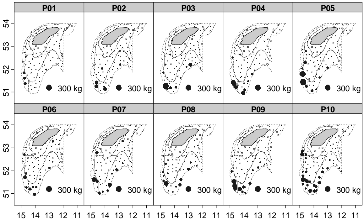
Figure 5. Geographic distribution of blackmouth catshark ( G. melastomus ) catches ( \text{kg}\cdot\text{haul}^{-1} ) during Porcupine survey time series (2001- 2010).
