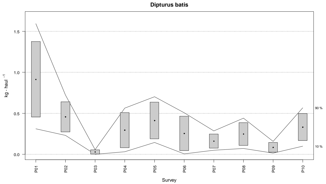
Figure 27. Changes in common skate ( Dipturus batis ) biomass index ( \text{kg} \cdot \text{haul}^{-1} ) during Porcupine survey time series (2001-2010). Boxes mark parametric standard error of the stratified index. Lines mark bootstrap confidence intervals ( \alpha = 0.80 , bootstrap iterations = 1000).
