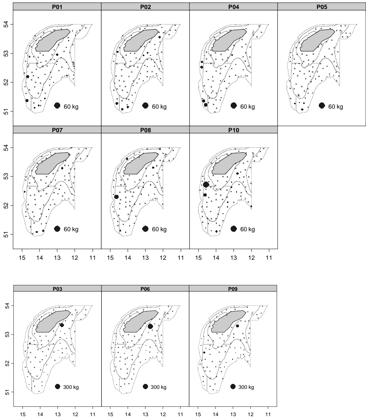
Figure 10. Geographic distribution of velvet belly ( E. spinax ) catches ( \text{kg}\cdot\text{haul}^{-1} ) during Porcupine surveys: in years of low biomass abundances (2001-2, 4-5 and 7-8-10) and high abundance (2003, 6 and 9), respectively upper and lower panels.
