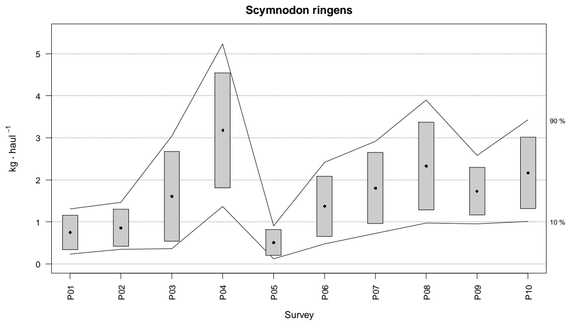
Figure 12. Changes in knifetooth dogfish ( Scymnodom ringens ) biomass index (kg · haul -1 ) during Porcupine survey time series (2001-2010). Boxes mark parametric standard error of the stratified biomass index. Lines mark bootstrap confidence intervals ( \alpha = 0.80 , bootstrap iterations = 1000).
