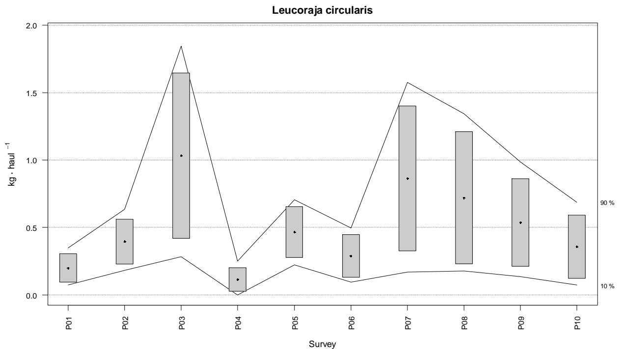
Figure 24. Changes in sandy ray ( Leucoraja circularis ) biomass index (kg · haul -1 ) during Porcupine survey time series (2001-2010). Boxes mark parametric standard error of the stratified biomass index. Lines mark bootstrap confidence intervals ( \alpha = 0.80 , bootstrap iterations = 1000).
