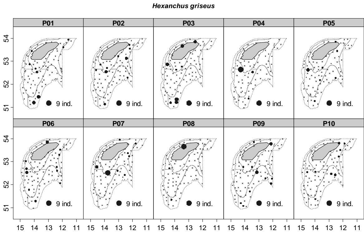
Figure 20. Geographic distribution of bluntnose sixgill shark ( H. griseus ) catches ( \text{ind} \cdot \text{haul}^{-1} ) in Porcupine surveys (2001-2010).
