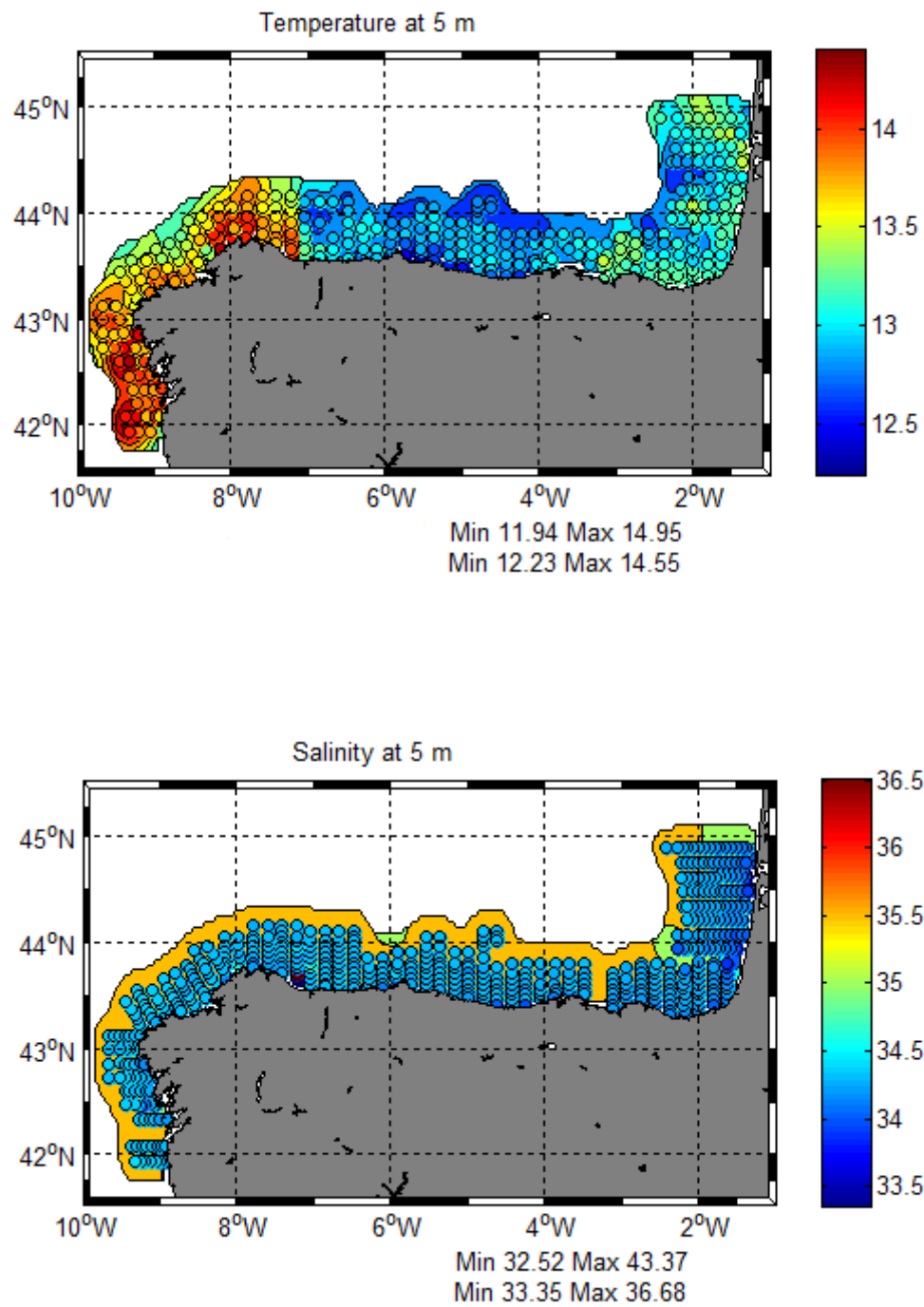
Figure 1. Temperature ( ^{\circ}\text{C} ) and salinity (PSU) at 5 m depth from CTD Sea Bird 37
