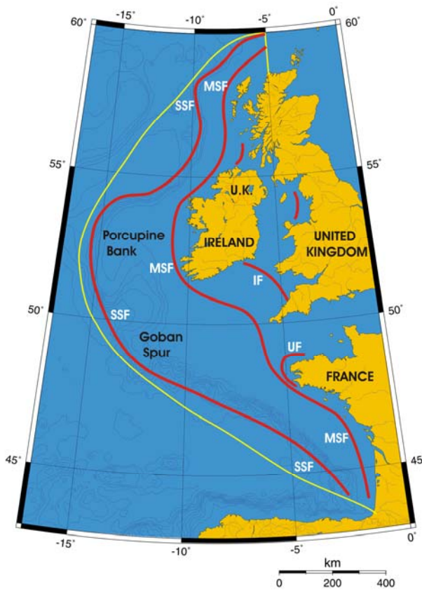
Figure XIII-37.1. Fronts of the Celtic-Biscay Shelf LME. IF, Irish Front; MSF, Mid-Shelf Front; SSF, Shelf-Slope Front; UF, Ushant Front. Yellow line, LME boundary. After Belkin et al. (2009).
