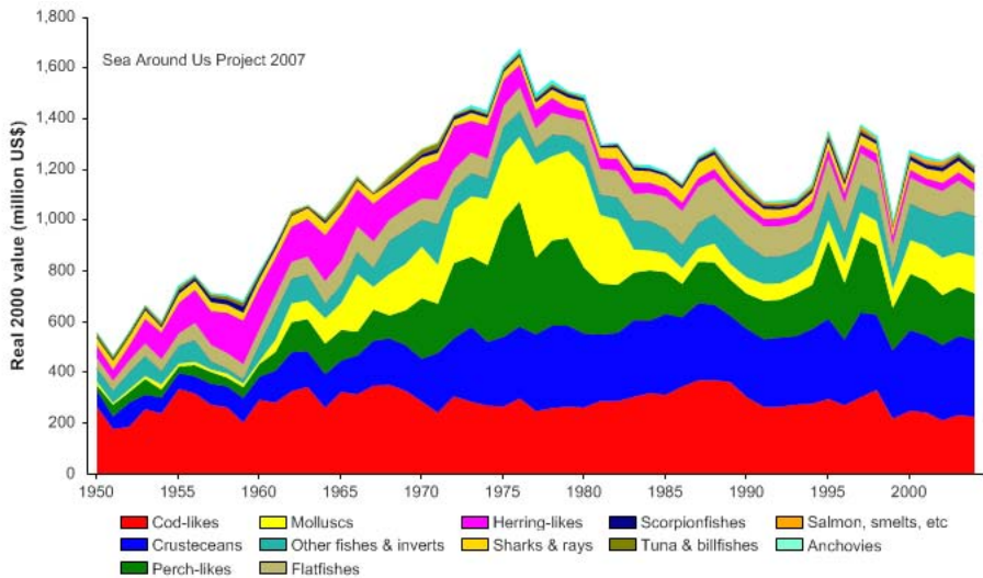
Figure XIII-37.5. Value of reported landings in the Celtic-Biscay Shelf LME by commercial groups (Sea Around Us 2007).
