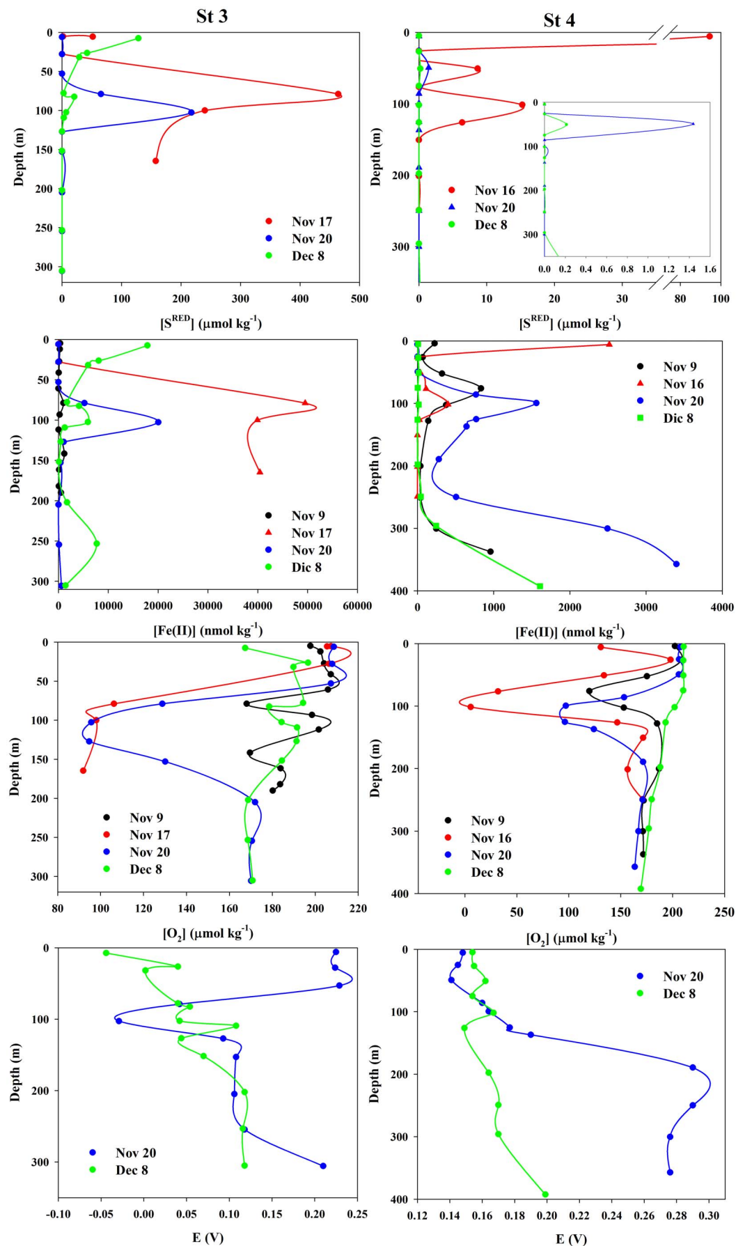
Figure 4 | Evolution of the concentration of reduced species close to the volcano. Vertical profiles of reduced sulfur species ( S^{\text{RED}} ), total Fe(II) and oxygen concentrations ( \mu\text{mol kg}^{-1} ), and Redox Potential (E, Volts), at stations 3 and 4 in November and December 2011.
