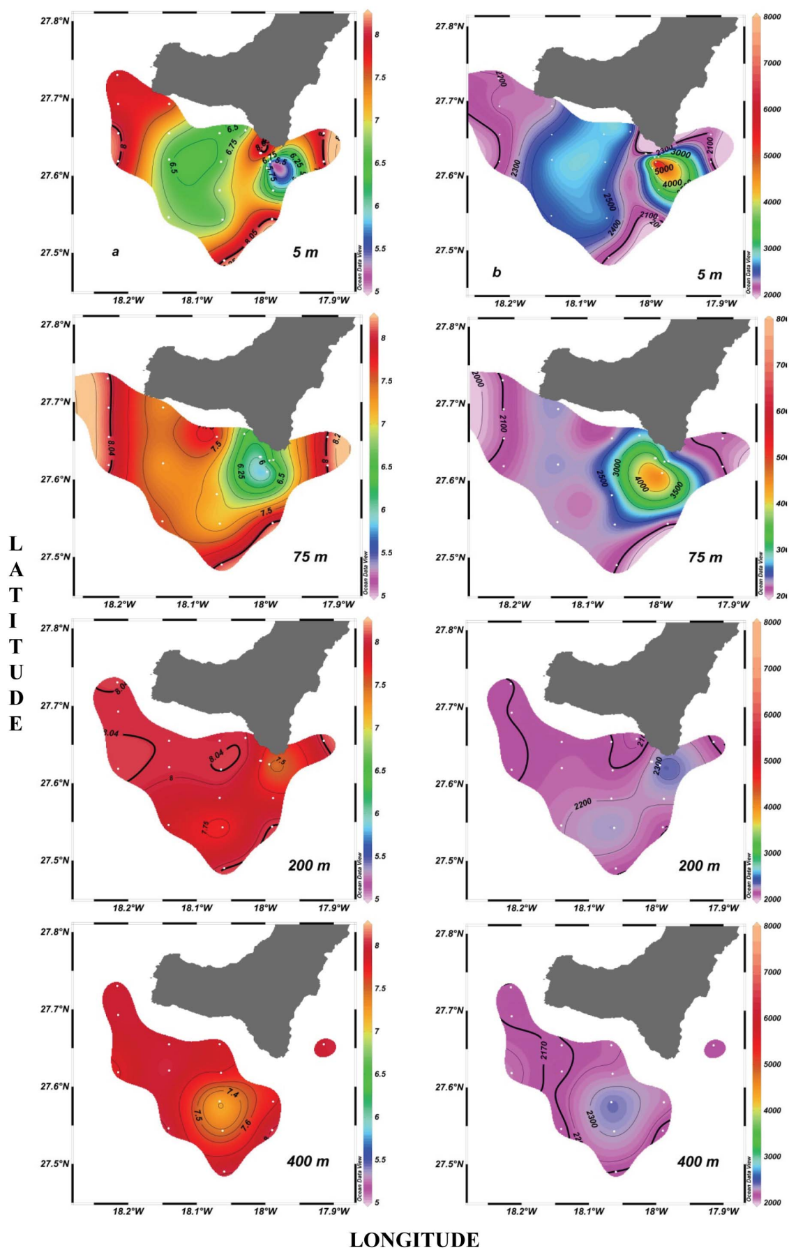
Figure 2 | Carbonate system variables distributions around the volcanic area. (a) pH in total scale at in situ conditions and (b) total dissolved inorganic carbon ( C_T , \mu\text{mol kg}^{-1} ) distributions at 5, 75, 200 and 400 m depth in the southwest of the island of El Hierro during Leg 3 in November 4 th to 9 th 2011.
