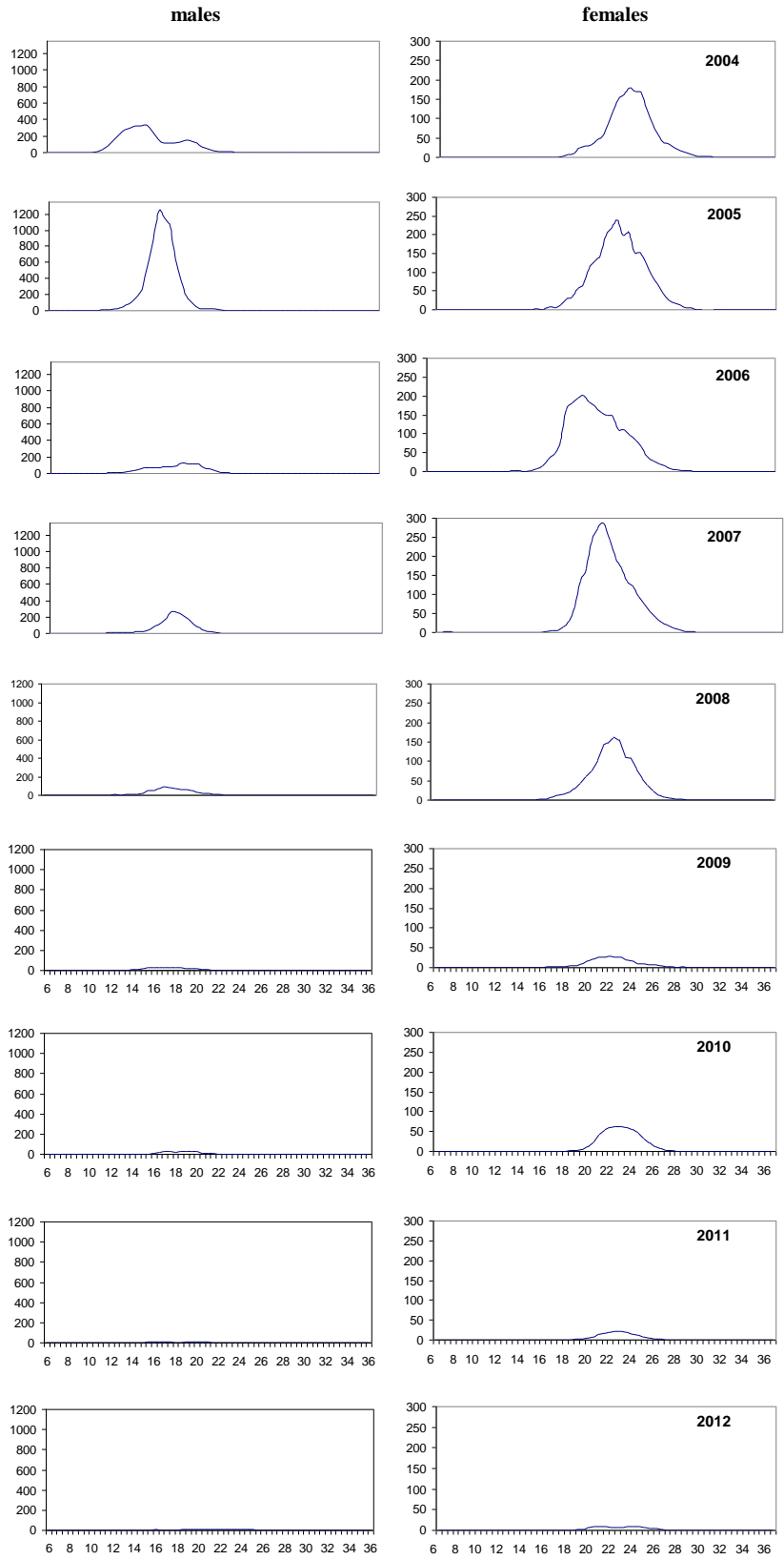
Figure 6. Shrimp size distribution from Flemish Cap 2004 -2012 surveys. Y-Axis=Frequency (10 6 ), X-Axis=Carapace Length (mm).
