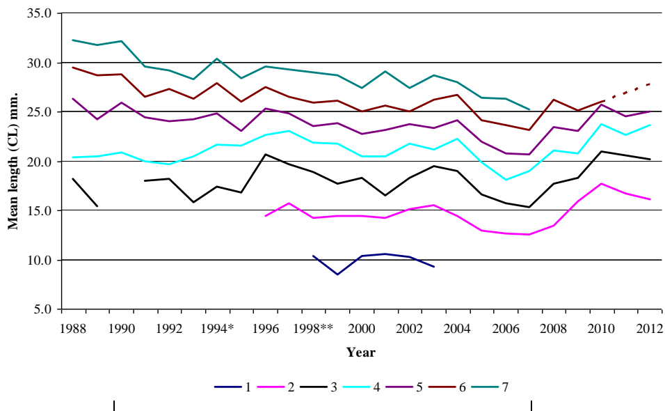
Figure 10. Shrimp mean lengths at age in the series of EU surveys on Flemish Cap.
