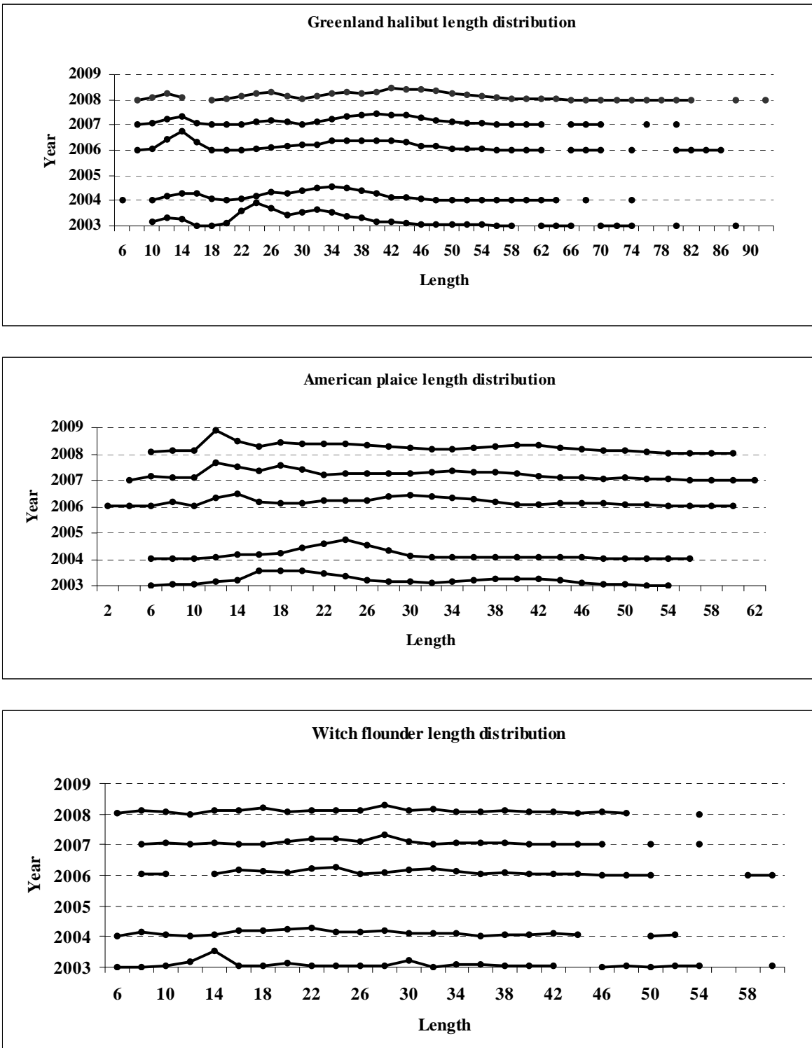
FIGURE 5.- Greenland halibut, American plaice and witch flounder length distribution (cm) in NAFO 3L: 2003-2008.
