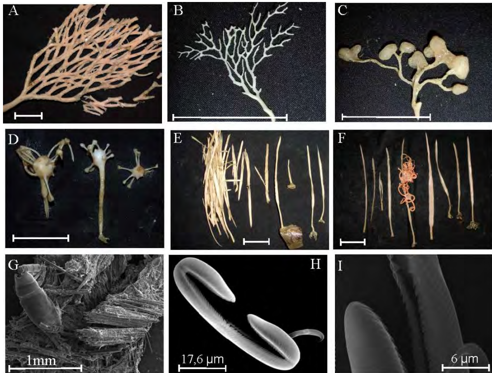
Fig. 8. Study carnivorous sponges. A. Asbestopluma sp. B. Asbestopluma sp. C. Chondrocladia sp. D. Chondrocladia sp. E. Euchelipluma sp. F. Euchelipluma sp. and brittle stars linked to one of the specimens. (Scale A-F 5 cm). G. Crustacean attached to the sponge spicules of Euchelipluma sp. H. Euchelipluma sp. Spicules: placochela and sigma. I. Placochela central detail
