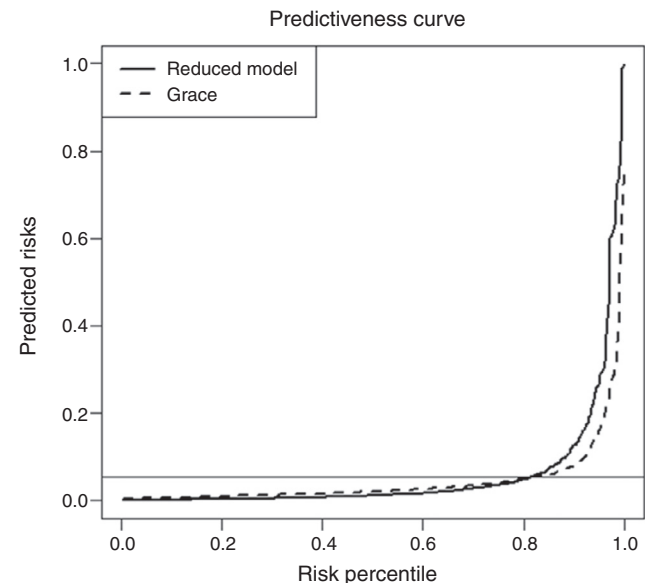
Figure 3 Predictiveness curves comparing the GRACE risk score and the reduced model. The reduced model correctly assigns lower risk to patients with lower risk percentiles and higher risk to patients with higher risk percentiles. The horizontal line represents the prevalence of in-hospital death (5.4%).
