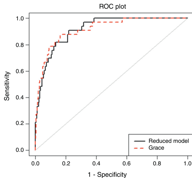
Figure 1 Receiver operating characteristic curve analysis comparing the GRACE risk score and the simplified prediction model (p=0.916).
