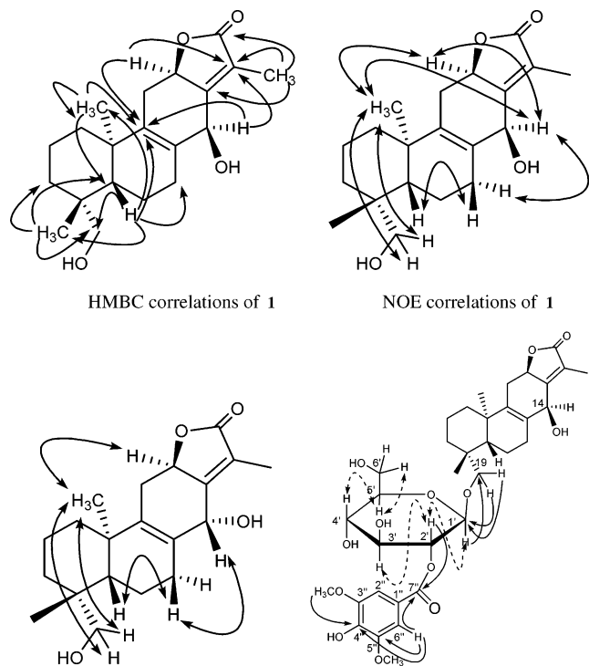
Figure 1. Important NMR correlations (HMBC: \rightarrow ; NOESY: \leftrightarrow ; ^1\text{H} - ^1\text{H} COSY: \dashleftarrow ) of 1 , 2 , and 5 .
