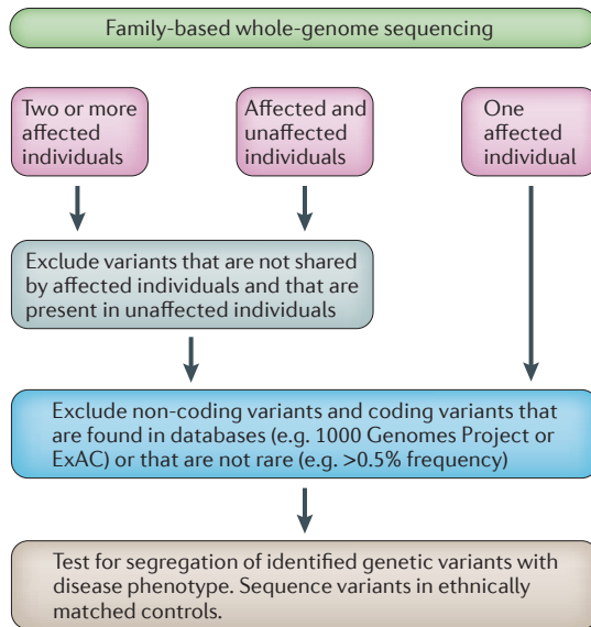
Figure 1 | Workflow for the whole-genome sequencing filtering approach in human family data. Usually, one, two or more affected individuals, or affected and unaffected individuals, in a family have their genomes or exomes sequenced. Variants that are not predicted to be nonsense, missense or splice-site variants are usually excluded from further analyses because it is unlikely that they are causal. When the mode of inheritance of a disease is known, this information can be used to aid the selection of variants. For example, for an autosomal dominant disease, the affected pedigree member's sequence data should display a heterozygous causal variant. Sequence data on additional pedigree members can help to reduce the number of variants that could potentially be disease causing. A final filtering step is performed in which those variants that are present in the databases dbSNP , 1000 Genomes , ExAC and Exome Variant Server are excluded. Additionally, bioinformatic tools, such as Polyphen-2 (REF. 102), and measures of conservation, for example, PhyloP 103 , are often used to predict whether a variant is deleterious and therefore likely to be disease causing. Even after filtering steps, there may be many variants that need to be followed up in the remaining family members to elucidate whether the variant (or variants) segregate with the disease phenotype. If the family is from a population that is not represented in databases, then ethnically matched controls need to be sequenced to evaluate the frequency of the variant (or variants).
