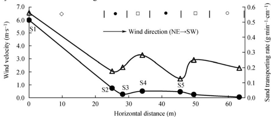
Figure 1 Variation of the wind speed at the height of 1 m and the sand transporting rate at 20 cm height above the ground inside and outside the shelter forest as measured in interdunes. ◇ Shifting sand; ● sand-obstructing forest; □ open space in forest; ○ sand-binding forest; △ wind velocity; ● sand transporting rate.
