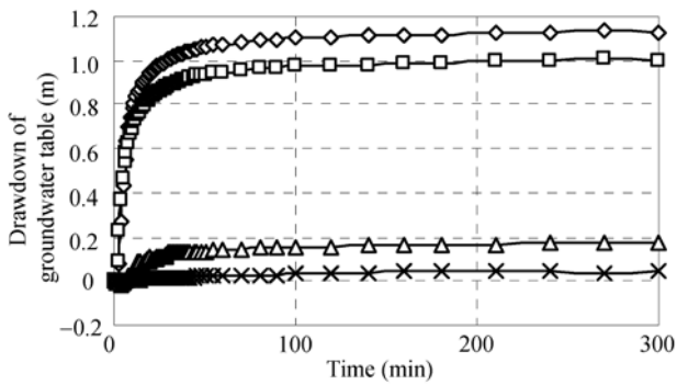
Figure 5 The variation of drawdown as a function of pumping time. —◇—, No. 1 observation well; —□—, No. 3 observation well; —△—, No. 9 observation well; —×—, No. 24 observation well.
