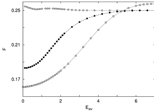
FIG. 2. Shot-noise suppression factor \mathcal{F} vs the value of the energy-averaging interval E_{av} for the three different billiards SIS (open square), Bun1 (filled square), and Bun2 (open circle).
