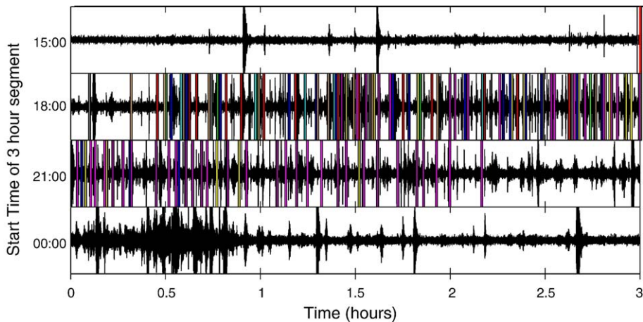
Fig. 1. Twelve hours of a low-frequency earthquake swarm on May 19 and 20, 1997, recorded on station MBGA in Montserrat in 4 consecutive time windows. Each vertical bar identifies a single event and the colour represents the family, which matches the colours in Fig. 3a.
