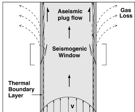
Fig. 7. A schematic cartoon illustrating the formation of shear fractures and their subsequent evolution into faults within a seismogenic window. Once formed the fractures move up due to the ascent of magma allowing friction-controlled plug flow to form. The opening of the fractures allows increased gas loss to the surroundings. The transition from seismogenic slip to aseismic plug flow may be due to frictional heating, as discussed in Section 3.1.
