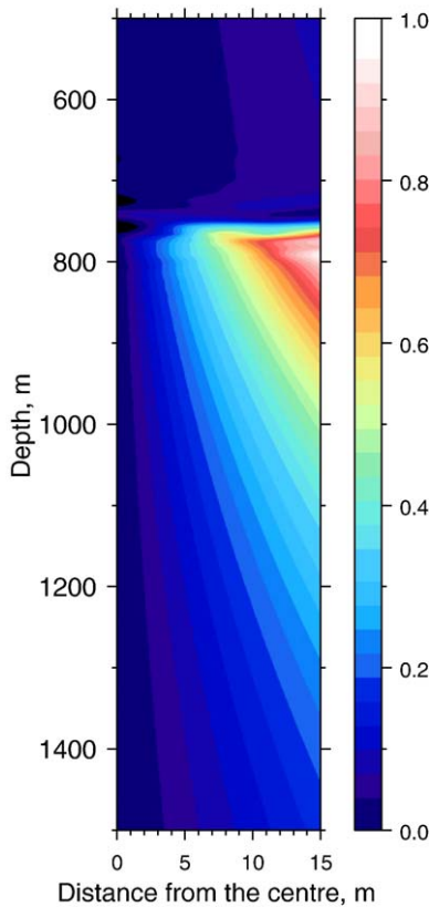
Fig. 6. Brittle failure ratio as defined in Eq. (4) between conduit centre and conduit wall. Note that failure occurs near the conduit wall where ratio exceeds 1; magma ascends above this depth as a plug under friction-controlled conditions.
