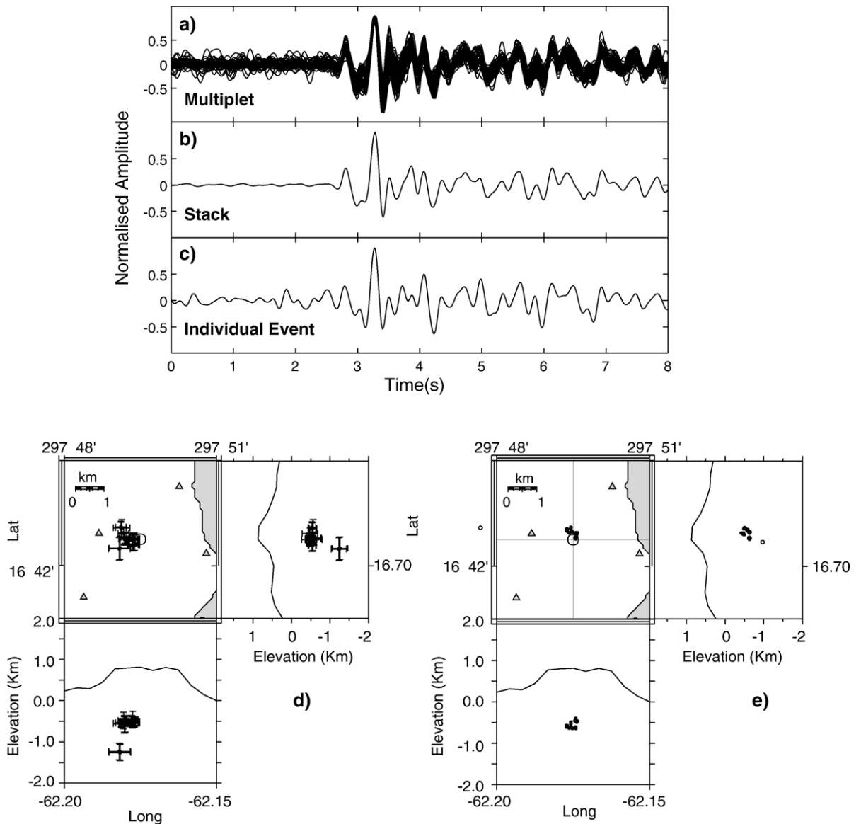
Fig. 2. Event family recorded in June 1997 on station MBGA in Montserrat; (a) 19 individual events, (b) stacked trace after cross correlation and aligning of individual events, and (c) individual event. Note the difficulty which would be encountered in isolating the correct P -phase from this individual event. (d) Hypocentre location of a series of 55 events using HYPOELLIPSE and a 3-layer velocity model; (e) hypocentral estimates for the same series of 55 events using VELEST where simultaneously a 3-layer velocity model is estimated. The average rms residual of the events is 0.013 s or one sample at 75 Hz, translating to \pm 40 m. The source locations cluster within a constant velocity zone and are approximately 500 m from any velocity boundary.
