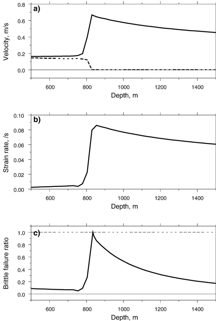
Fig. 5. (a) Variation of velocity with depth, solid-line is the velocity in conduit centre and the dashed line is the velocity at the conduit wall. (b) Variation of strain rate with depth 0.5 m from conduit wall. (c) Brittle failure ratio (Eq. (4)) 0.5 m from conduit wall plotted between the depths of 500–1500 m, brittle failure where ratio exceeds 1.
