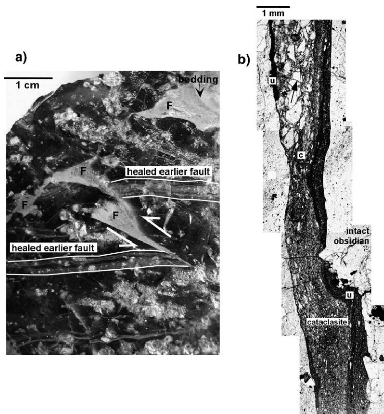
Fig. 4. (a) Part of a network of irregular fractures in obsidian at Skridugil Conduit, Raudufossafjöll, Iceland. The fault network (f) is filled with pale grey fragmented material, which locally exhibits bedding (indicated). An earlier healed fault zone has an apparent offset of 2 cm where cut by a fracture. Modified from Tuffen and Dingwell (2004). (b) Photomicrograph of a fault zone within obsidian. The zone is between 1 and 2 mm thick and filled with cataclasite (pale grey, labelled c) and ultracataclasite (dark grey, labelled u), which have the same composition as the surrounding obsidian (o). The arrow indicates where an obsidian clast within the cataclasite (near-white) is cut by a small fracture, indicating in-situ grain size reduction. Modified from Tuffen and Dingwell (2004).
