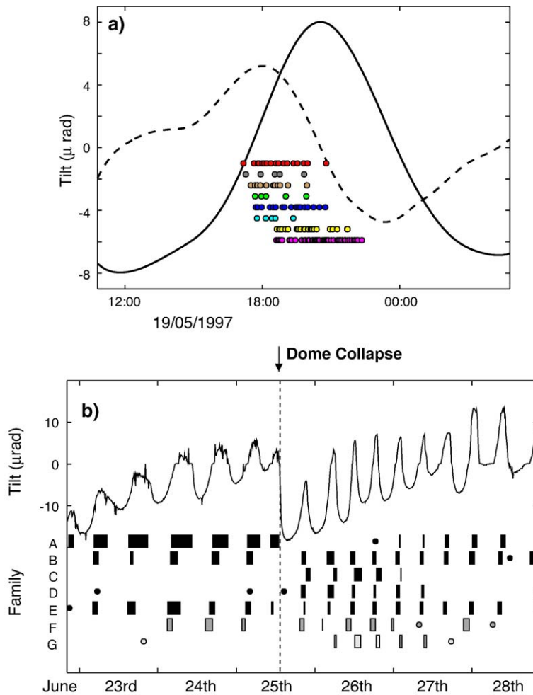
Fig. 3. (a) Families as shown in Fig. 1 together with tilt (solid line) and its time derivative (dashed line), both low-pass filtered. (b) Waveform families compared to the tilt record over the 6 days between June 23 and June 28, 1997. Note that different families represent different source locations: the oblongs represent the families, with different shades and patterns distinguishing between the different waveform groups A to G. The start of the oblong is positioned where the first event of that family occurs in that swarm and the end coincides with the last event. The dome collapse occurred at approximately 12:45 on June 25, 1997.
