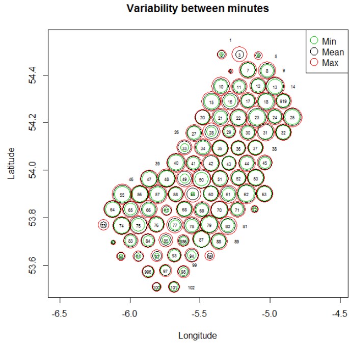
Figure 6: FU15 western Irish Sea grounds: Plot of the variability in density between minutes for each station in 2014.
