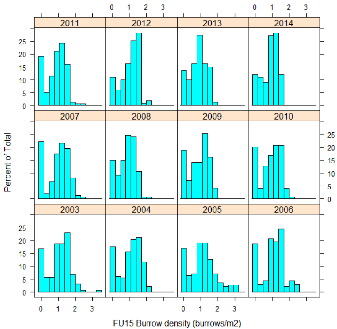
Figure 5: FU15 western Irish Sea grounds: Histogram of burrow density distributions by year from 2003-2014.
