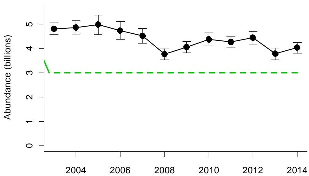
Figure 11: FU15 western Irish Sea grounds: Time series of geo-statistical abundance estimates (in billions of burrows) from 2003 -2014. Error bars correspond to the 95% confidence intervals. Dashed green line is MSY B_{\text{trigger}} of 3.0 billion burrows.
