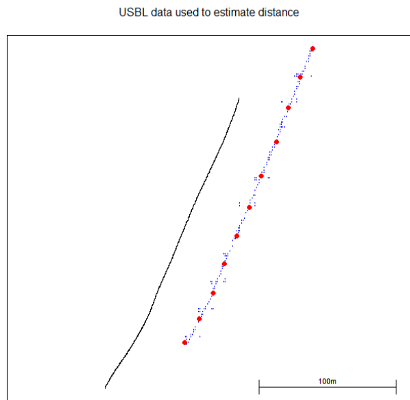
Figure 2: FU15 western Irish Sea grounds: R - tool quality control plot for station 18 of the 2014 survey.
