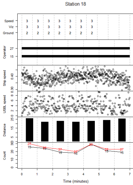
Figure 2: FU15 western Irish Sea grounds: R - tool quality control plot for station 18 of the 2014 survey.
