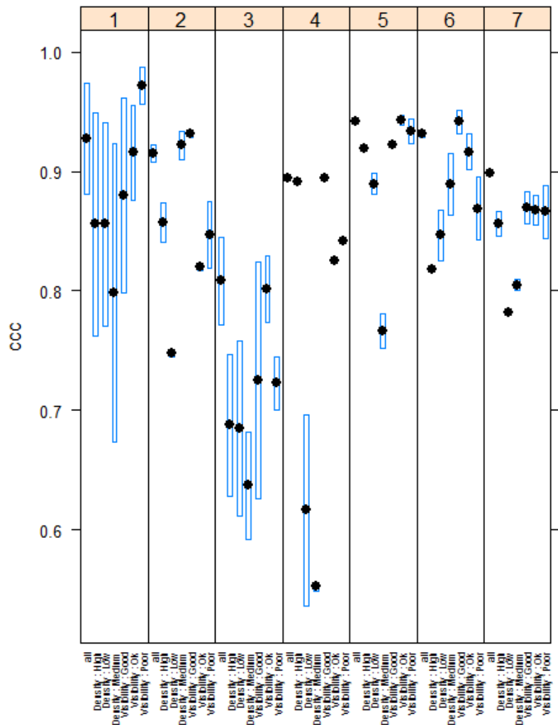
Figure 1: FU15 western Irish Sea grounds: 2014 count performance against the reference counts as measured by Linn's CCC for FU15 reference set. Each panel represents an individual. The x-axis (from left to right) shows all stations pooled, high density, low density, medium density and visibility good.
