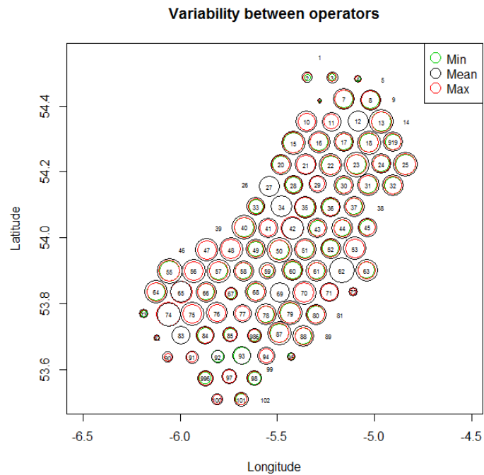
Figure 7: FU15 western Irish Sea grounds: Plot of the variability in density between operators (counters) for each station in 2014.
