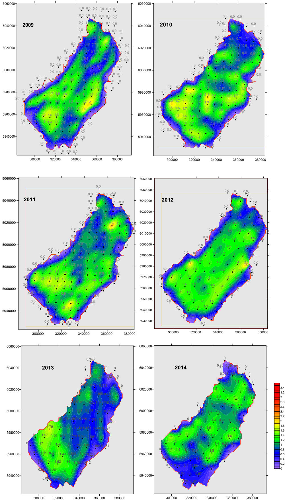
Figure 10: FU15 western Irish Sea grounds: Contour plots of the krigged density estimates by year from 2009 -2014.
