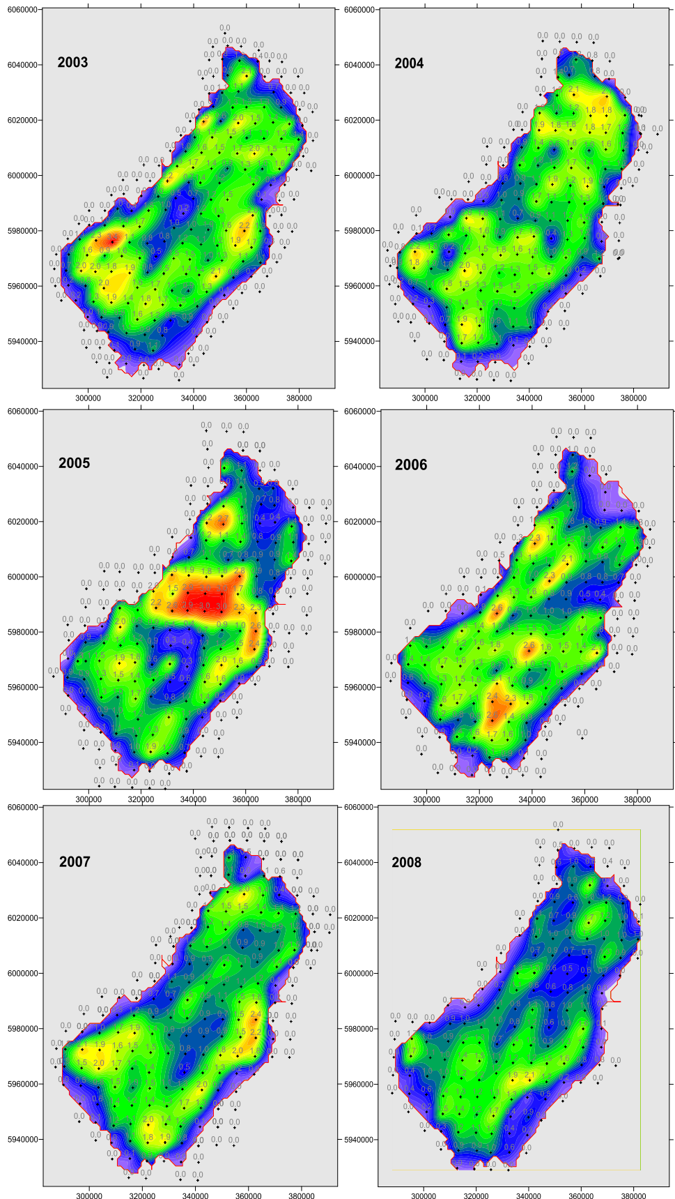
Figure 9: FU15 western Irish Sea grounds: Contour plots of the krigged density estimates by year from 2003 -2008.
