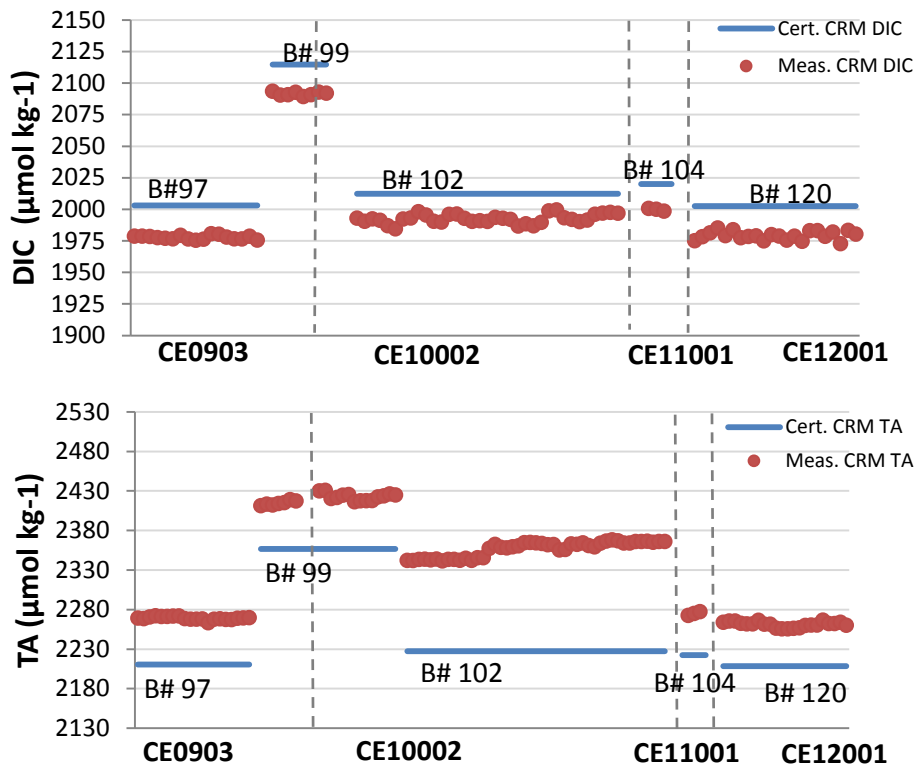
Fig. 2. DIC and TA CRM measured values plotted against certified values for each of the surveys. Dashed lines indicate a new survey.
