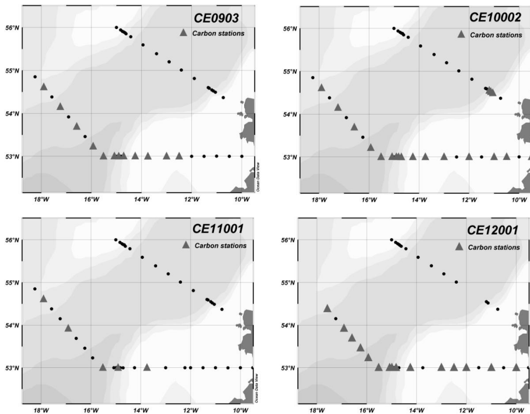
Fig. 1. Station positions from the surveys CE0903 (February 2009), CE10002 (February 2010), CE11001 (January 2011) and CE12001 (January 2012). Stations with triangle symbols are where carbonate parameters were measured. Note in CE11001 only surface samples were taken, in other years samples were taken through the water column.
