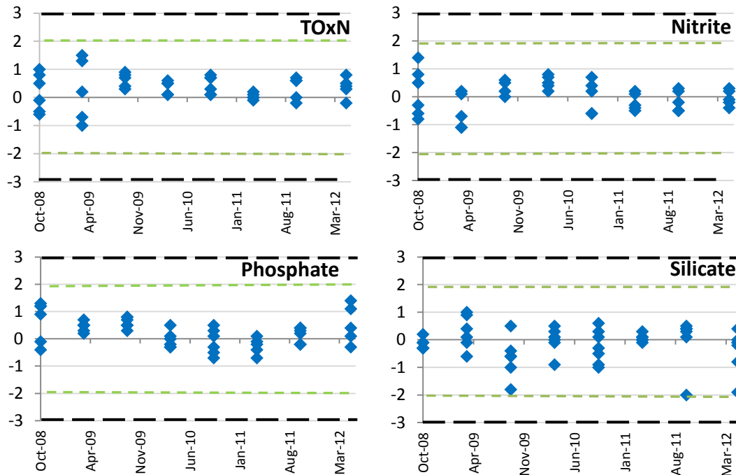
Fig. 4. z scores of 8 QUASIMEME rounds of nutrients in the marine environment between October 2008 and May 2012, where the green dashed lines indicate a z score of 2. The dashed black line at a z score of \pm 3 designates unsatisfactory performance.
