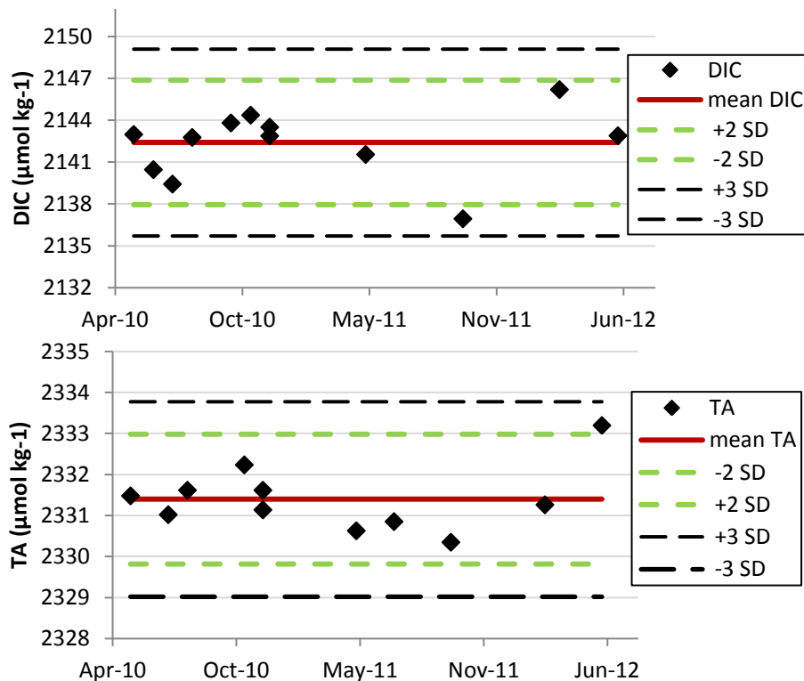
Fig. 3. Average monthly (from at least 2 sample bottles) DIC and TA concentrations over 2 yr of storage. The mean and standard deviations for DIC were based on the first year of storage when concentrations were within \pm 3 \mu\text{mol kg}^{-1} around the mean, while both years of storage results were used for TA as they were all within \pm 2 \mu\text{mol kg}^{-1} of the mean.
