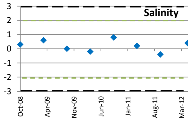
Fig. 5. z scores of 8 QUASIMEME rounds of nutrients in the marine environment between October 2008 and May 2012, where the green dashed lines indicate a z score of 2. The dashed black line at a z score of \pm 3 designates unsatisfactory performance.
