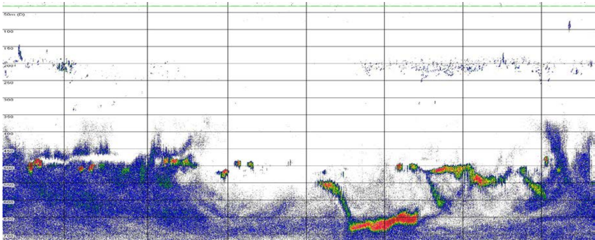
a). Blue whiting echotracess recorded along the 55°30N in the Hebrides target area by the RV Celtic Explorer. Echotracess were observed 15 nmi west of the shelf break in open water. Note the maximum school depth of 680m, the deepest schools recorded during the survey reached 720m.
