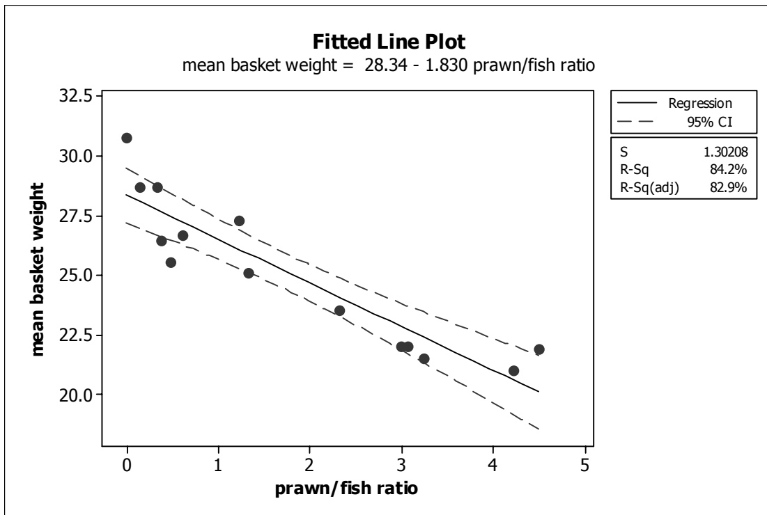
Figure 3.1. Fitted line plot of mean basket weights per haul (kg) against Nephrops /fish ratio.
