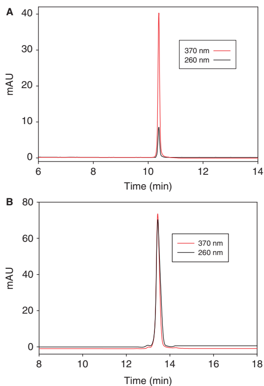
Figure 3. Calculation of \epsilon_{370}^{SeU} and \epsilon_{260}^{SeU} via RP-HPLC analysis. (A) HPLC profile of 3'-SeUMP at 260 nm (solid line) and 370 nm (dashed line). (B) HPLC profile of 5'-SeUU-3' dimer at 260 nm (solid line) and 370 nm (dashed line). The samples ( 3'-SeUMP and 5'-SeUU-3' ) were analyzed on a Welchrom XB-C18 column ( 4.6 \times 250 mm, 5 \mu ) at a flow of 1.0 ml/min and with a linear gradient of 5–50% B in 20 min, with a retention time of 10.3 and 13.6 min, respectively. Buffer A: 10 mM TEAAc (pH 7.1); B: 50% acetonitrile in 10 mM TEAAc (pH 7.1).
