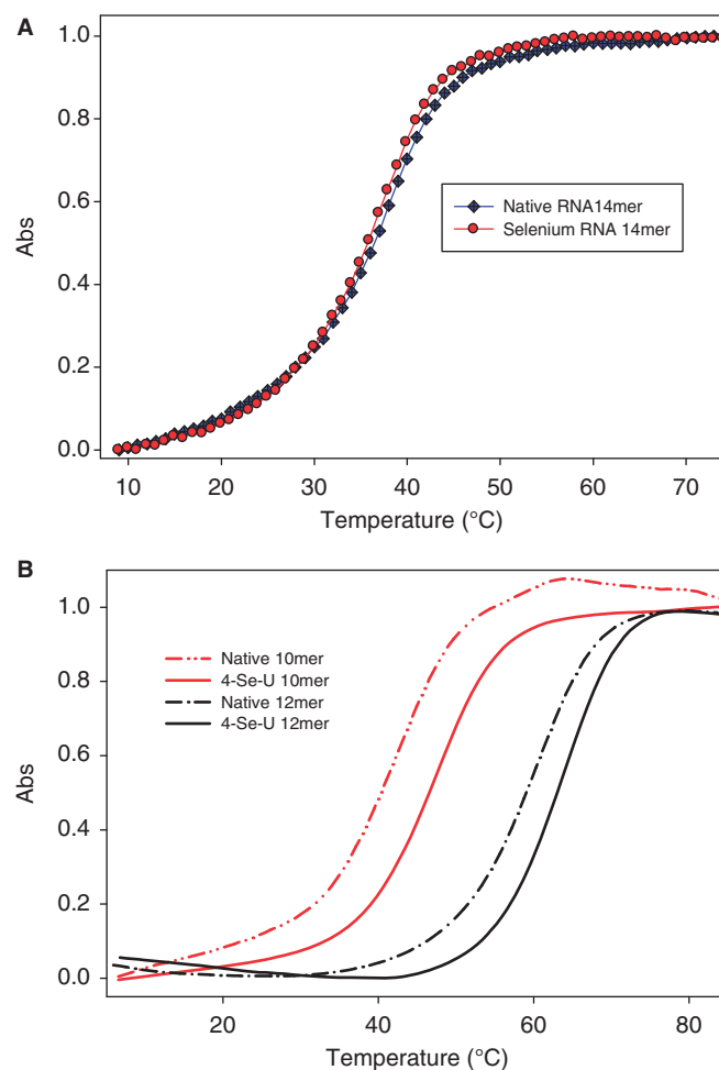
Figure 4. (A) Normalized T_m curve of Se-RNA ( 5'-UUA-SeU-AUAUAUAUAA-3' ) 2 , compared with the corresponding native RNA. The Se-RNA (circle line): T_m = 37.3 \pm 0.5^\circ\text{C} ; the native (diamond line): T_m = 38.0 \pm 0.3^\circ\text{C} . (B) Normalized T_m profiles of Se-RNA 10mer ( 5'-rU-SeU-AGCUAGCU-3' ) 2 and 12mer ( 5'-U-SeU-CGCGAUCGCG-3' ) 2 , compared with their corresponding natives. The native RNA-10mer (gray dash-dot line): T_m = 42.2 \pm 0.2^\circ\text{C} ; the Se-RNA 10mer (gray solid line): T_m = 47.1 \pm 0.3^\circ\text{C} ; the native RNA 12mer (black dash-dot line): T_m = 59.4 \pm 0.3^\circ\text{C} ; the Se-RNA 12mer (black solid line): T_m = 63.2 \pm 0.3^\circ\text{C} .
