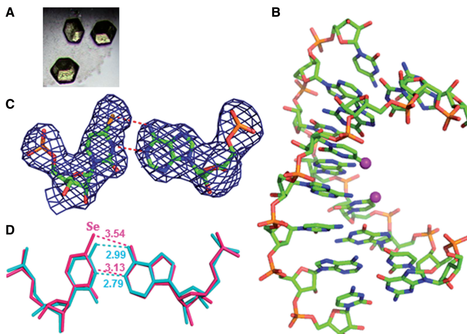
Figure 7. The yellow crystals and structures of the 4-Se-U RNA octamer, ( 5' -GUG- ^{76}\text{SeU} -ACAC- 3' ) 2 . The Se atoms are labeled as purple balls. (A) Crystal image. (B) The Se-RNA duplex structure (PDB ID: 4IQS; 2.75 Å resolution). (C) Electron density map (2F o -F c ) and model of the ^{76}\text{SeU}\cdot\text{A} pair at the level of 1.0 \sigma . (D) Superimposition of ^{76}\text{SeU}\cdot\text{A} pair (in pink) with native U2 \cdot A15 pair (in cyan); the H-bond lengths are indicated individually.
