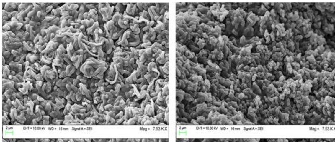
Figure 21 Photomicrographs of interior of calcium-alginate bead (left) and calcium-alginate PVA bead (right).
