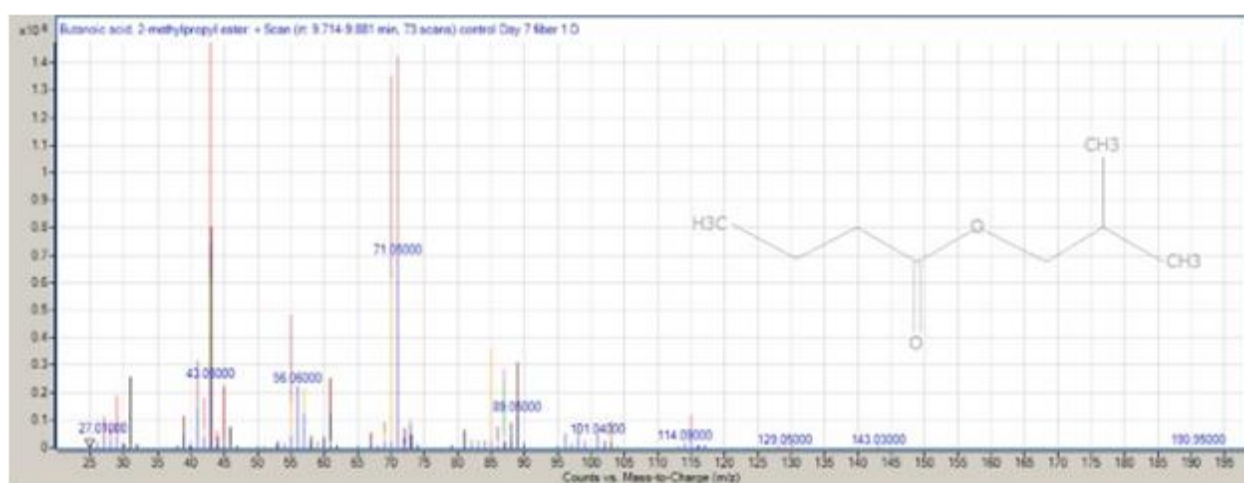
3. Mass spectrum of butanoic acid, 2-methylpropyl ester
