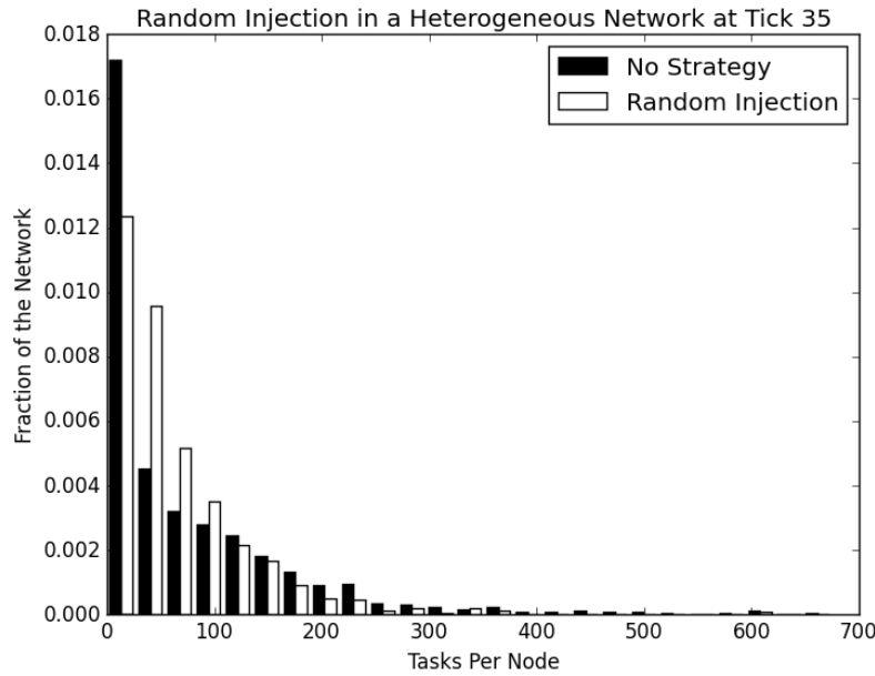
Figure 8.12: The workload distribution of heterogenous networks after 35 ticks. We can see the network using the random injection strategy is experiencing a better distribution of work.
