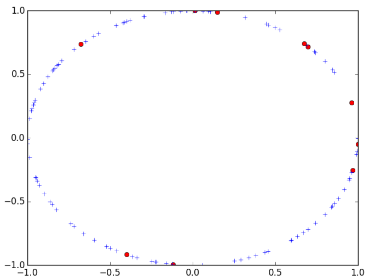
Figure 8.2: A visual example of data and nodes in a Chord DHT with 10 nodes (represented by red circles) and 100 tasks (blue pluses). Nodes are responsible for all the tasks that fall along the perimeter between themselves and their predecessor, which is the closest node counterclockwise.
