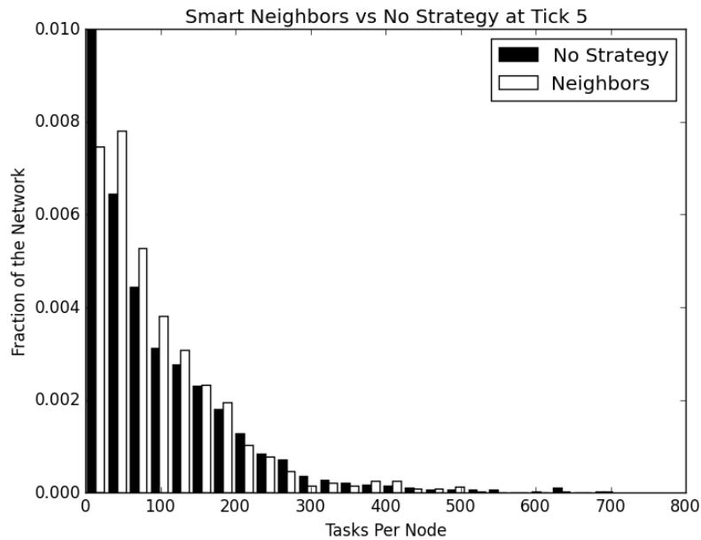
Figure 8.15: The workload in the networks after 5 ticks. We can see that the network using neighbor injection has directed more nodes that would be idling to perform work. This is especially apparent in comparison to Figure 8.13.
