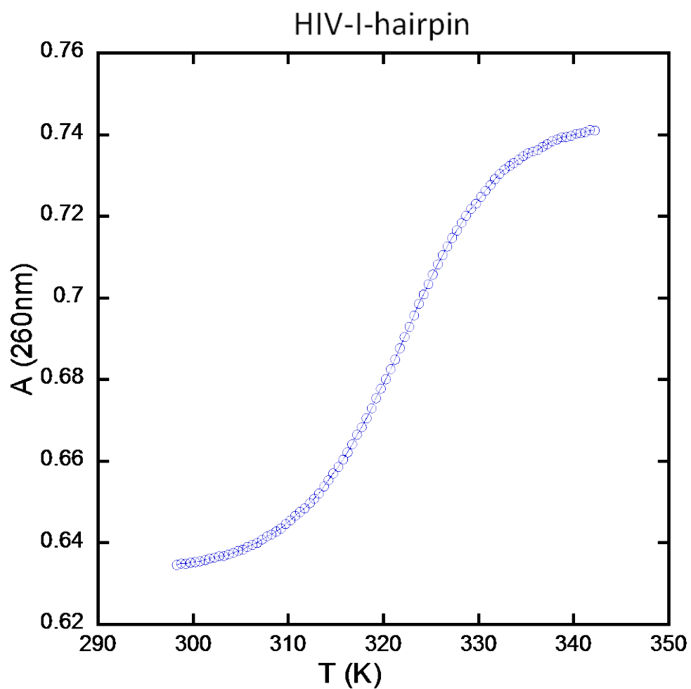
Figure 3.13 T m curve for HIV-I-hairpin. T m is 322.7 K.
