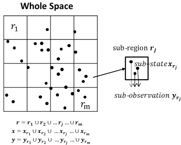
Figure 3.1 Example of state partitioning and generated sub-states and sub-observations.
