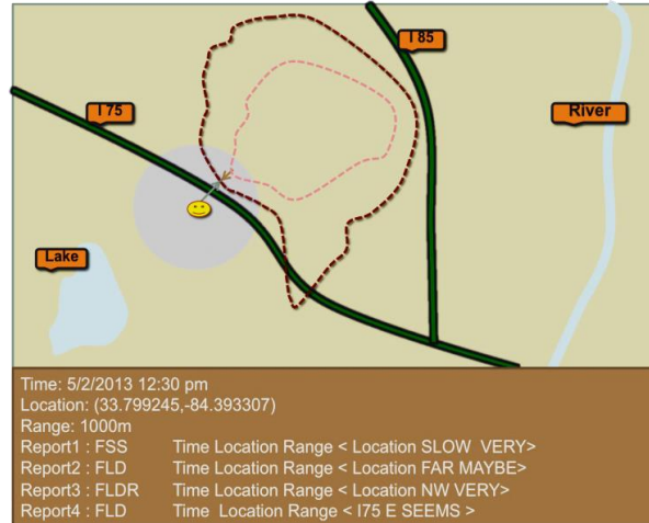
Figure 5.3 An example of soft data and corresponding fire shape
