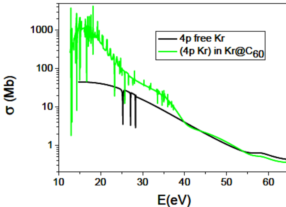
Figure4.13 Cross sections of 4p of free Kr and 4p Kr inside Kr@C 60
