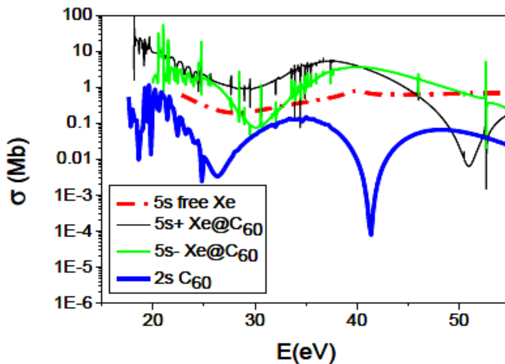
Figure 4.20 Cross sections of 5s of free Xe, 2s of C_{60} and hybridized states
