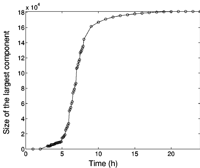
FIG. 4. The size of the largest component (cluster) over time. A sharp transition is observed at about 6 a.m. when people move from home to work or school.
