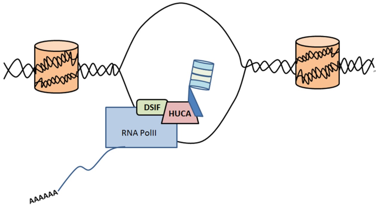
Figure 2.1 Proposed Mechanism
