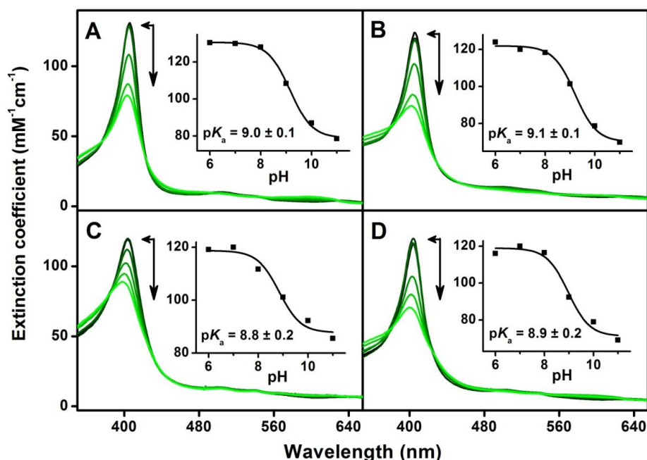
Figure 3.4.3 Effect of pH on the optical absorption spectra of cmTDO and its mutants (8 \mu\text{M} ). (A) WT TDO, (B) Q73F, (C) H72S, (D) H72N. This experiment was performed over the pH range from 6 (black) to 11 (green) in multi-component buffer solutions containing 50 mM Tris, 50 mM MOPS, and 50 mM glycine. The pH difference between each two adjacent data set is 1 unit. The arrows indicate the trends of changes in the spectra. The insets present the changes in the Soret band absorption intensity as a function of pH. The solid lines are the best fits of the experimental data to one-proton titration curves.
