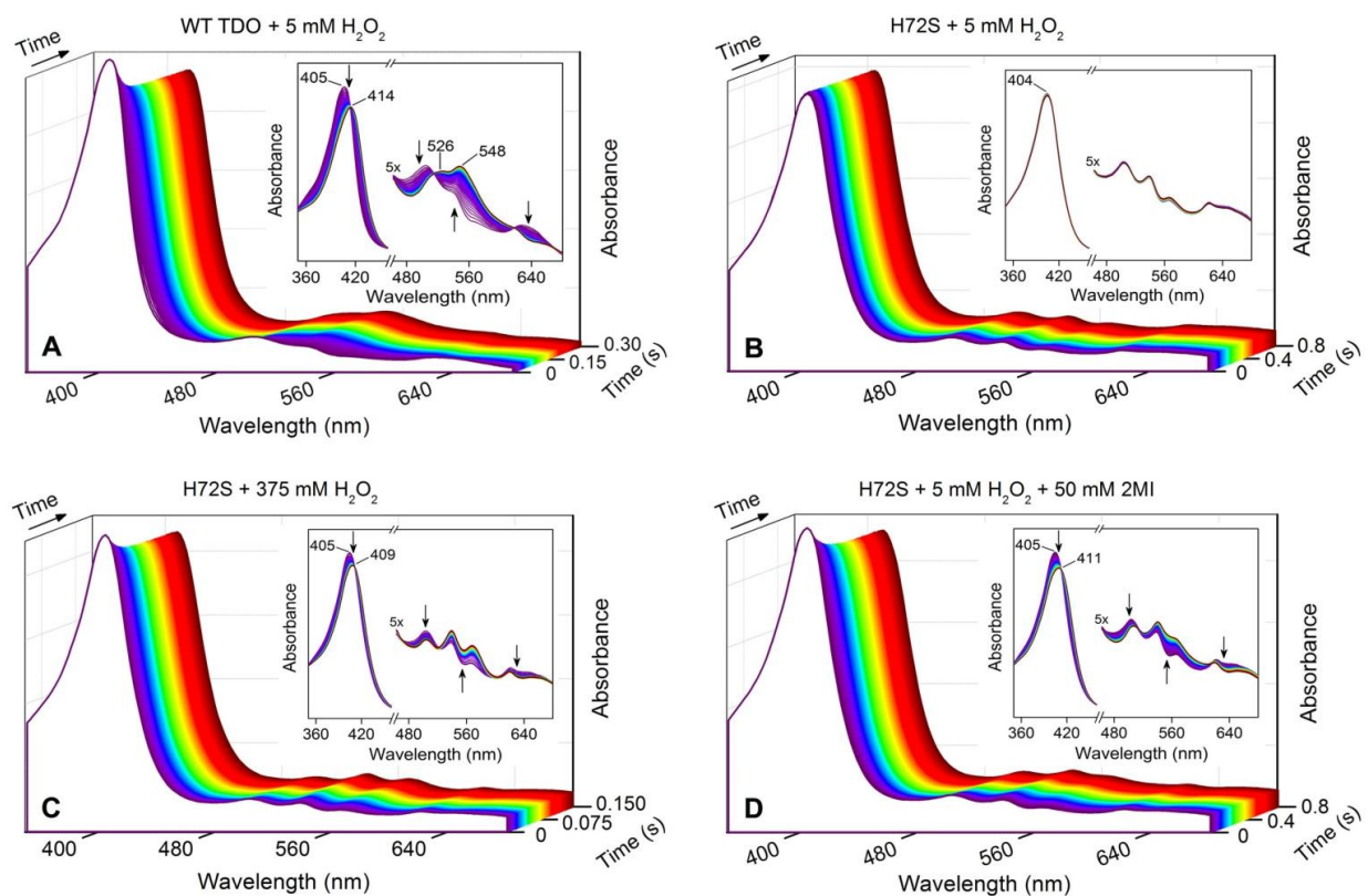
Figure 3.4.10 Time-resolved stopped-flow UV-vis spectra of the reactions between cmTDO (15 \mu\text{M} ) and \text{H}_2\text{O}_2 at 4 ^\circ\text{C} . (A) WT TDO + 5 mM \text{H}_2\text{O}_2 (0–0.3 s); (B) H72S + 5 mM \text{H}_2\text{O}_2 (0–0.8 s); (C) H72S + 375 mM \text{H}_2\text{O}_2 (0–0.15 s); (D) H72S + 5 mM \text{H}_2\text{O}_2 with 50 mM 2MI in the reaction system (0–0.8 s). The insets are expanded views of the visible bands. The arrows indicate the trends of changes in the spectra.
