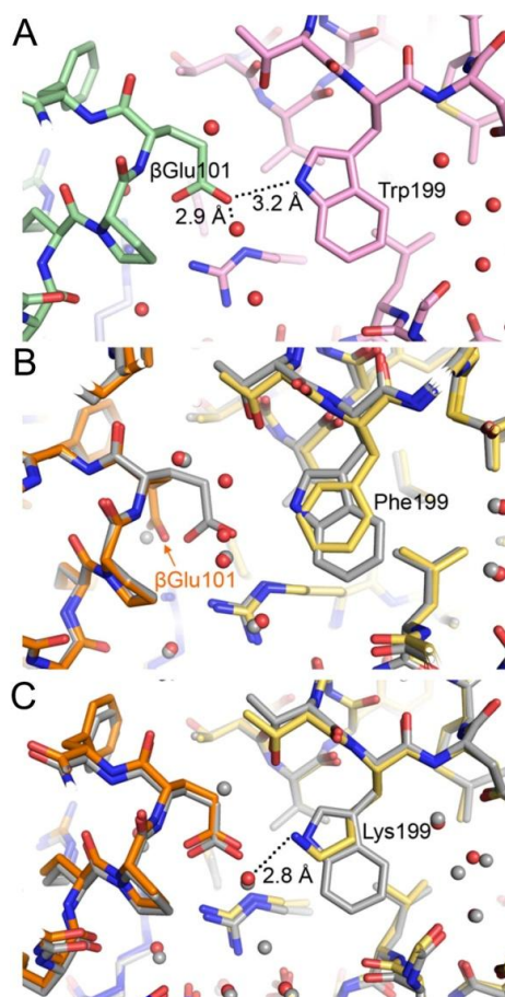
Figure 5.4.4 Interface structure of the MauG-preMADH complex near residue 199. (A) H-bonding network in the WT MauG-preMADH structure (PDB entry 3L4M) involving Trp199 and \beta Glu101 of preMADH (WT MauG, pink; \beta -preMADH, green; \alpha -preMADH, blue). Overlays of 3L4M with the W199F MauG-preMADH coordinates (B) and the W199K MauG-preMADH coordinates (C) are also shown (W199F/K MauG, yellow; \beta -preMADH, orange; \alpha -preMADH, blue; WT MauG-preMADH, gray).
