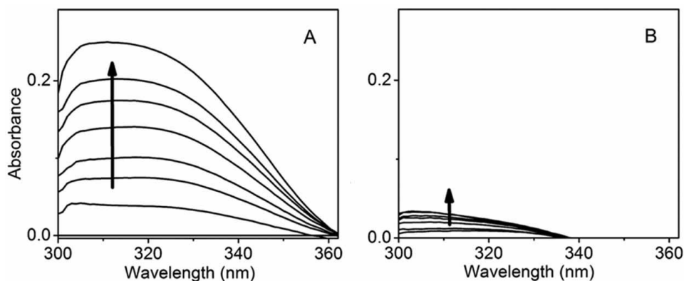
Figure 2.4.7 Effect of hydroxyurea on the production of NFK in an anaerobic reaction system containing ferric TDO (5 \mu\text{M} ), L-Trp (5 mM), and titrated H 2 O 2 . H 2 O 2 was titrated to a final concentration of 175
