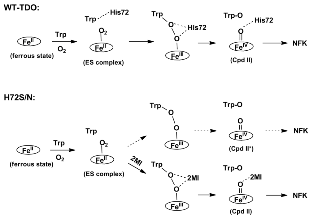
Figure 3.5.2 Proposed role of His72 in catalysis during the dioxygenase reaction cycle of cmTDO. “Cpd II” differ from “Cpd II*” by an additional H-bonding interaction to either the His72 residue or 2MI.
