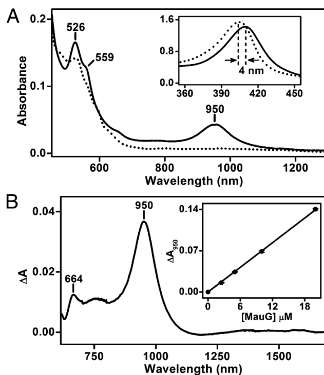
Figure 6.4.1 The bis -Fe(IV) state of MauG exhibits a spectral feature in the NIR region. (A) Vis-NIR spectra of MauG (5 \mu\text{M} ) before (dotted trace) and after (solid trace) addition of ten eq. of \text{H}_2\text{O}_2 . The inset shows an expanded view of the Soret region. (B) Vis-NIR difference spectrum of MauG (5 \mu\text{M} ) obtained in \text{D}_2\text{O} -based buffer by subtracting the initial spectrum of di-ferric MauG from the one after the addition of ten eq. of \text{H}_2\text{O}_2 . The inset presents the absorption change at 950 nm ( \Delta A_{950} ) as a function of [\text{MauG}] \mu\text{M} with the ratio of [\text{H}_2\text{O}_2] to [\text{MauG}] kept at 10:1. The solid line is the linear fit of the experimental data.
