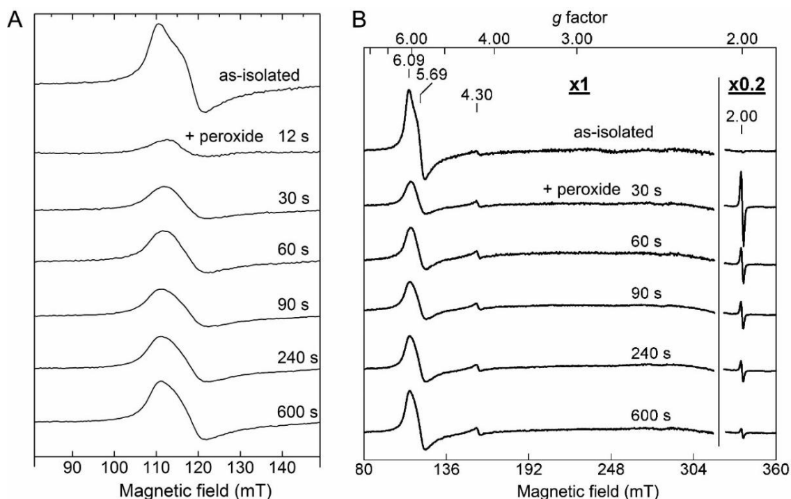
Figure 2.4.3 Changes in the EPR signals of cmTDO during the reaction of ferric TDO ( 150\ \mu\text{M} ) with \text{H}_2\text{O}_2 ( 900\ \mu\text{M} ). (A) EPR spectra of TDO before and after the reaction with \text{H}_2\text{O}_2 . (B) Overall EPR spectra with a zoom-in view of the g = 2 region. The time points at which the EPR samples were frozen after the addition of \text{H}_2\text{O}_2 are listed in the figures. The spectra were collected at the following conditions: temperature, 10 K; microwave frequency, 9.44 GHz; microwave power, 1 mW; and modulation amplitude, 0.8 mT.
