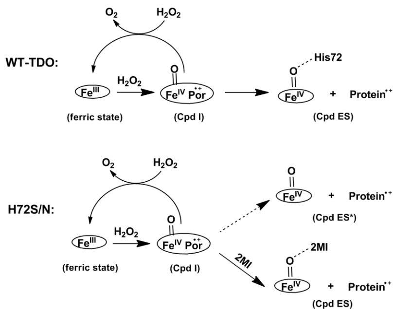
Figure 3.5.1 Proposed role of His72 in stabilizing the ferryl species in cmTDO in the reaction with H 2 O 2 . The catalase-like cycle of TDO has been reported previously [96]. “Cpd ES” differ from “Cpd ES*” by an additional H-bonding interaction to either the His72 residue or 2MI. The accumulation of “Cpd ES*” can be observed only in the presence of highly concentrated H 2 O 2 ( i.e. , over 100 mM).
