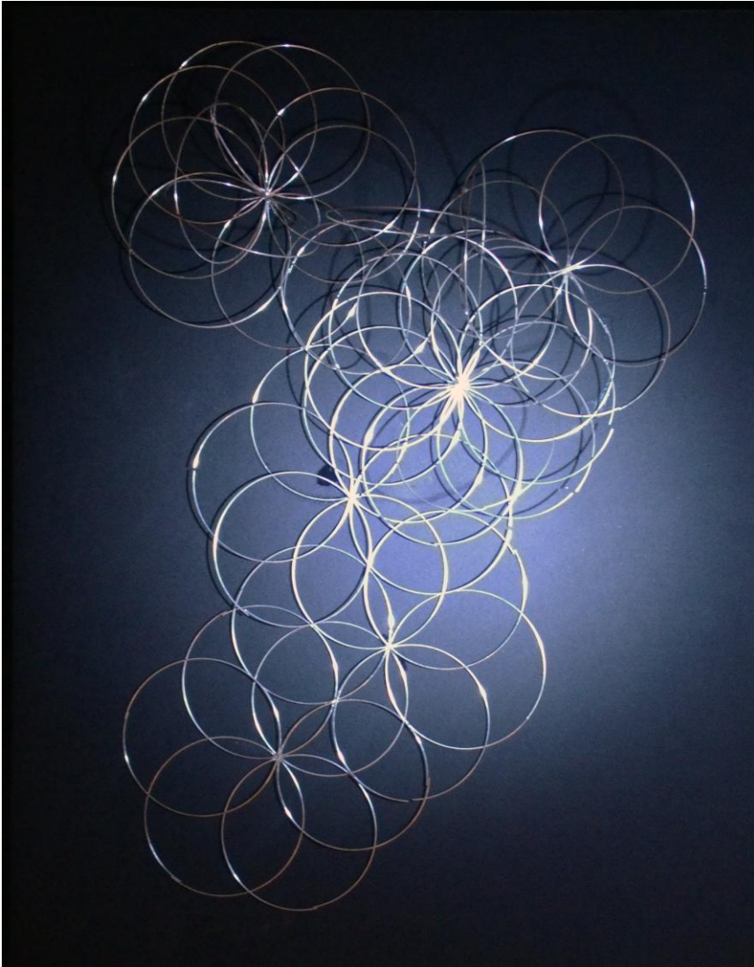
Figure 19. Circle Exploration: Pattern Finding, 6-point geometries
