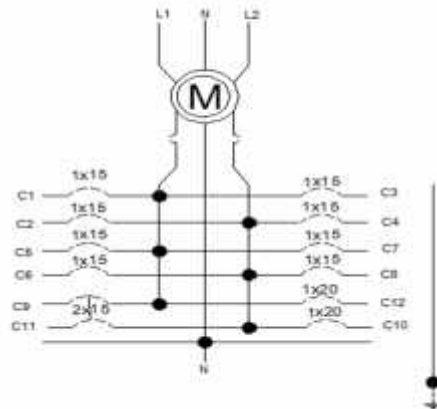
Figura18.Diagrama unifilar tablero 4
