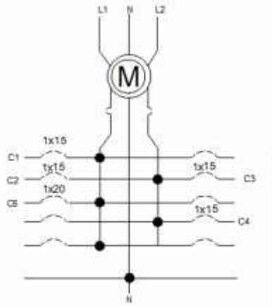
Figura14. Diagrama unifilar tablero principal
