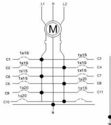
Figura17.Diagrama unifilar tablero 3
