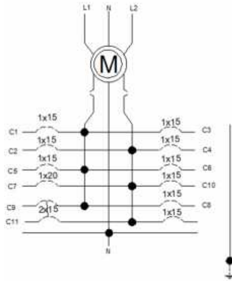
Figura16.Diagrama unifilar tablero 2
