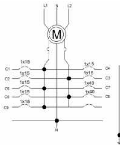
Figura19.Diagrama unifilar tablero 5
