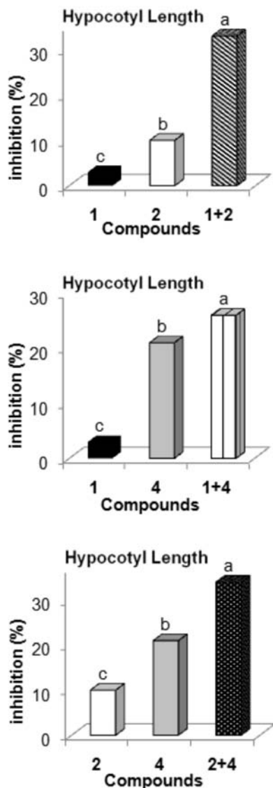
Figure 6. Allelopathic effect of stilbenes 1 , 2 e 4 , separately, and in pairs, over the hypocotyl development of malícia weed seedling. Data is shown in percentages of inhibition in relation to control treatment; distilled water. Letters show significant differences by the Tukey test (5%).
