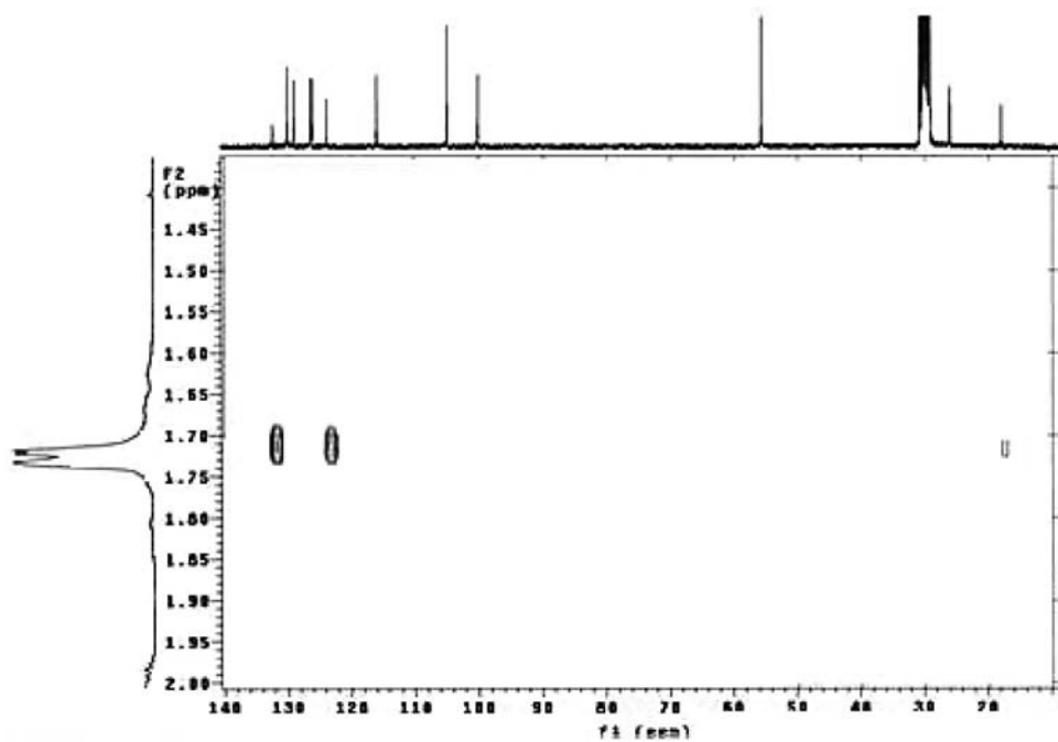
Figure S6. HMBC NMR experiment of the compound 2 (expansion 2).
