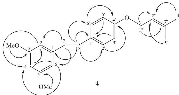
Figure 2. Key HMBC (H → C) correlations of compound 4 .
