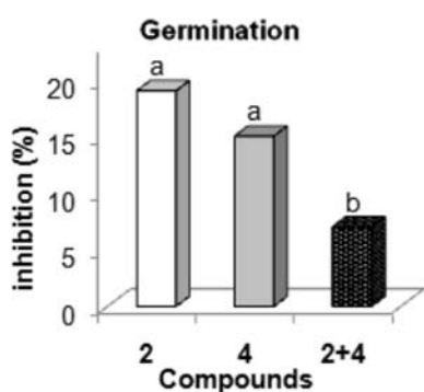
Figure 4. Allelopathic effect of stilbenes 1 , 2 and 4 , separately, and in pairs, over seed germination of malicia weed seedling. Data is shown in percentages of inhibition in relation to control treatment; distilled water. Letters show significant differences by the Tukey test (5%).
