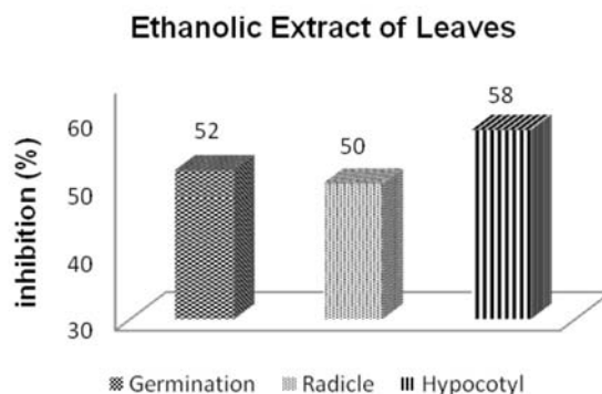
Figure 3. Effects of ethanolic extract from Deguelia rufescens var. urucu leaves over germination and development malícia weed seedling. Data is shown in percentages of inhibition in relation to control treatment, distilled water.
