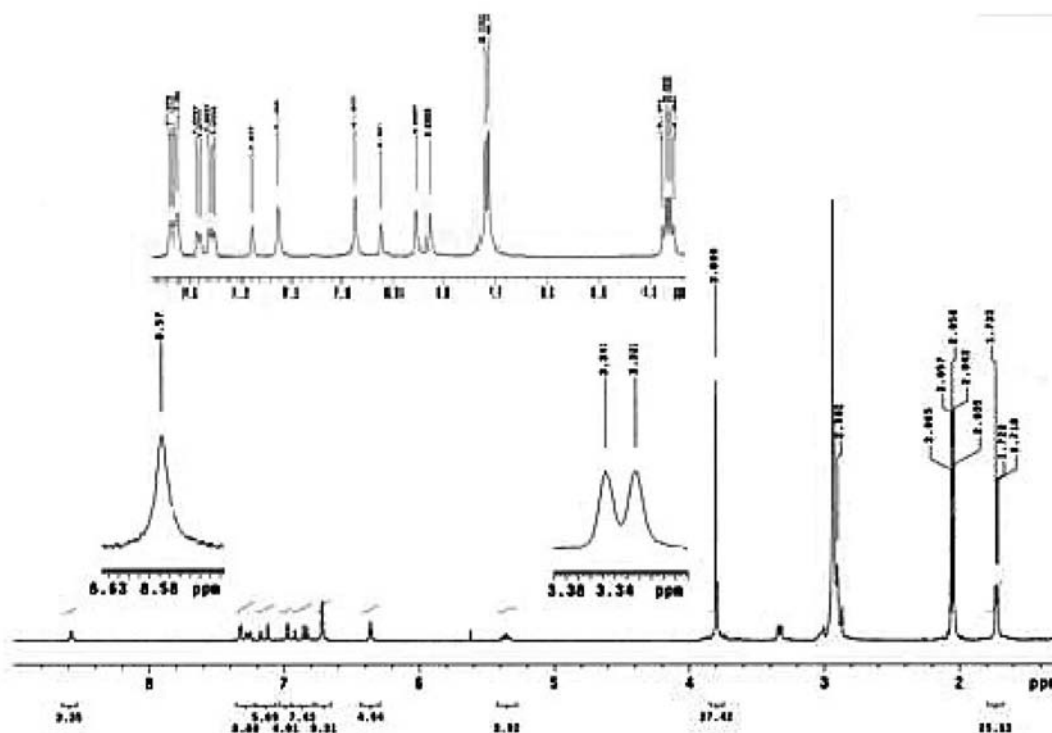
Figure S1. 1 H NMR spectrum [in (CD 3 ) 2 CO, 300 MHz] of the compound 2 isolated from leaves of Deguelia rufescens var. urucu .
