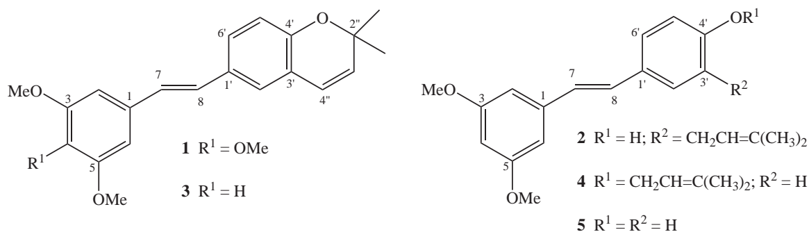
Figure 1. Chemical structure of stilbenes 1-5 , isolated from Deguelia rufescens var. urucu leaves.
