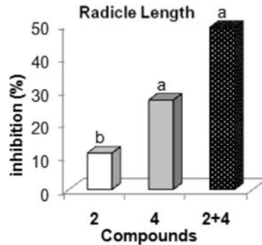
Figure 5. Allelopathic effect of stilbenes 1 , 2 e 4 , separately, and in pairs, over root development of malicia weed seedling. Data is shown in percentages of inhibition in relation to control treatment; distilled water. Letters show significant differences by the Tukey test (5%).
