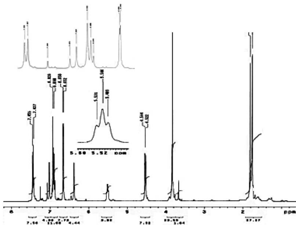
Figure S7. ^1\text{H} NMR spectrum (in \text{CDCl}_3 , 300 MHz) of the compound 4 isolated from leaves of Deguelia rufescens var. urucu .
