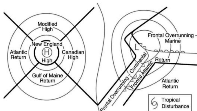
Fig. 2. Circulation-to-environment synoptic weather classification for the East Coast of New England
