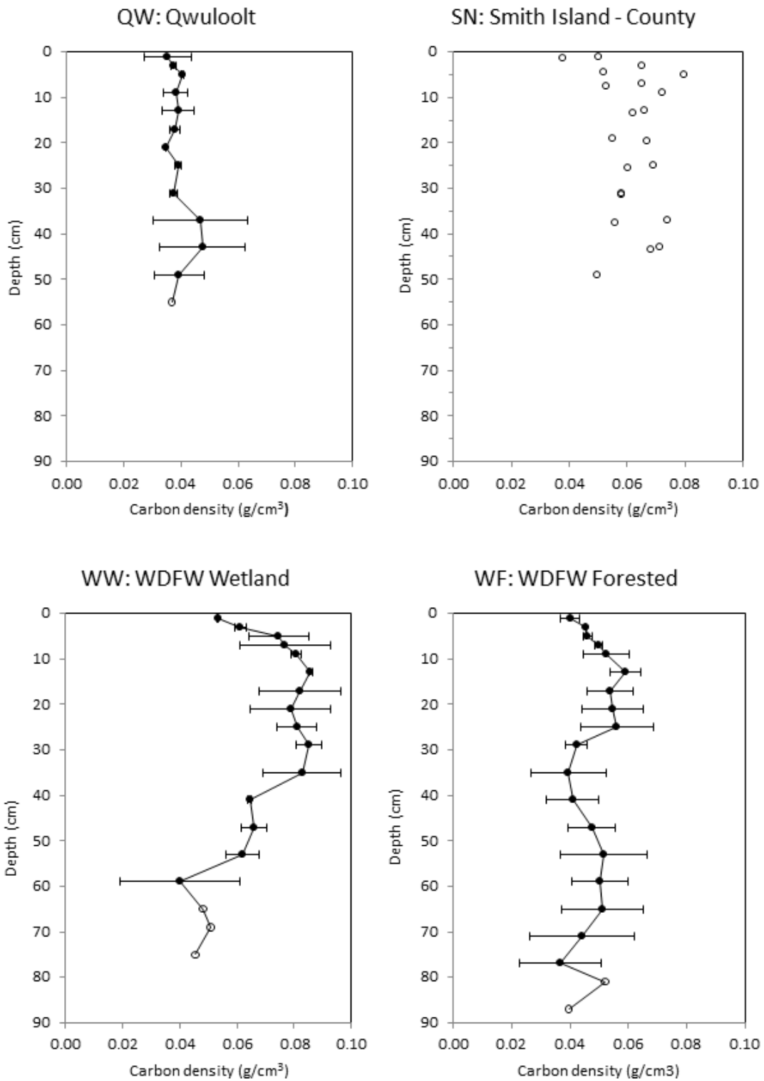
Figure 16. Carbon density profiles at sites intended for future restoration. Error bars represent ± 1 standard deviation (n = 2). Hollow points denote depths with no replication.
