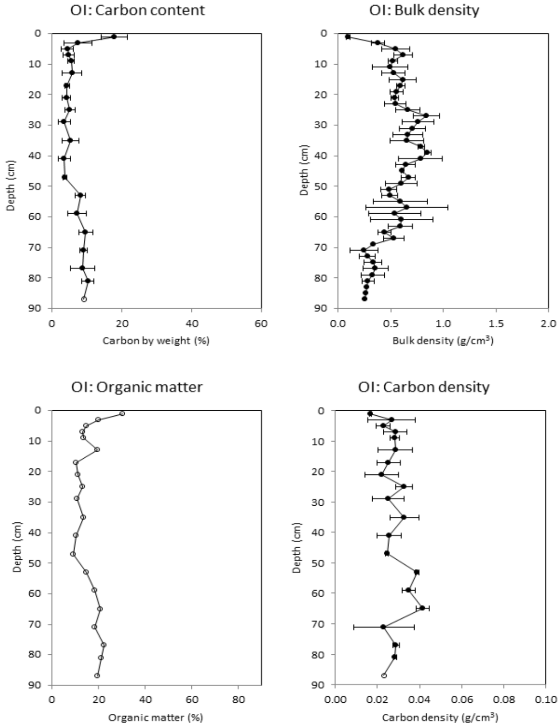
Figure 25. Otter Island soil profile with carbon content, bulk density, organic matter content, and carbon density. Error bars represent ± 1 standard deviation (n = 2). Hollow points denote depths with no replication.
