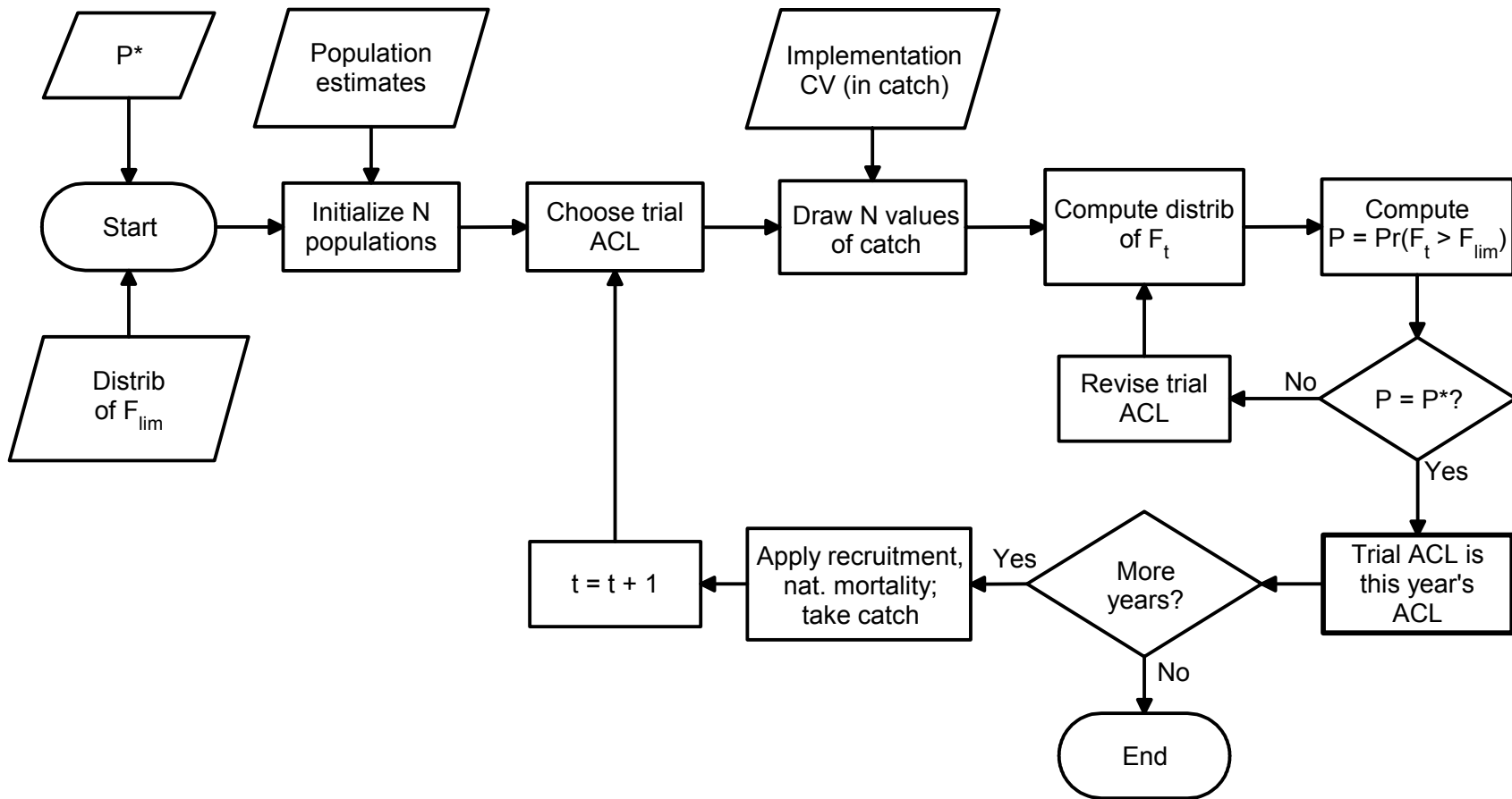
Figure 1. Algorithm for computing ACLs by PASCL method. Input quantities shown as parallelograms.
