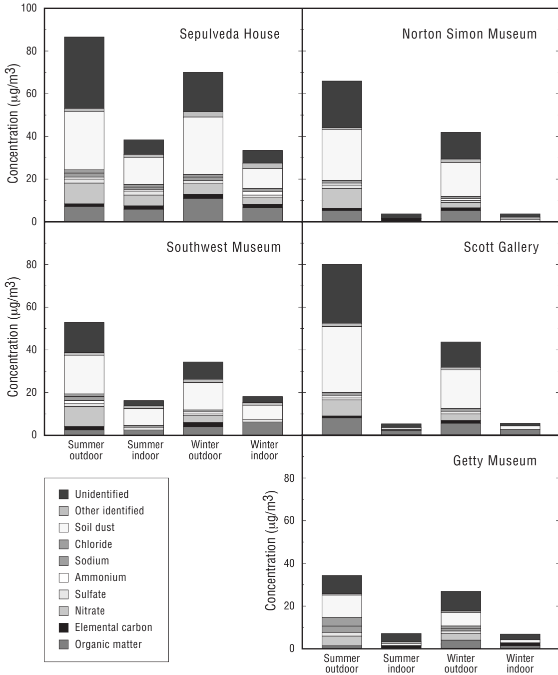
Figure 2.6. Seasonal mean chemical-mass balances for outdoor and indoor coarse particles.
