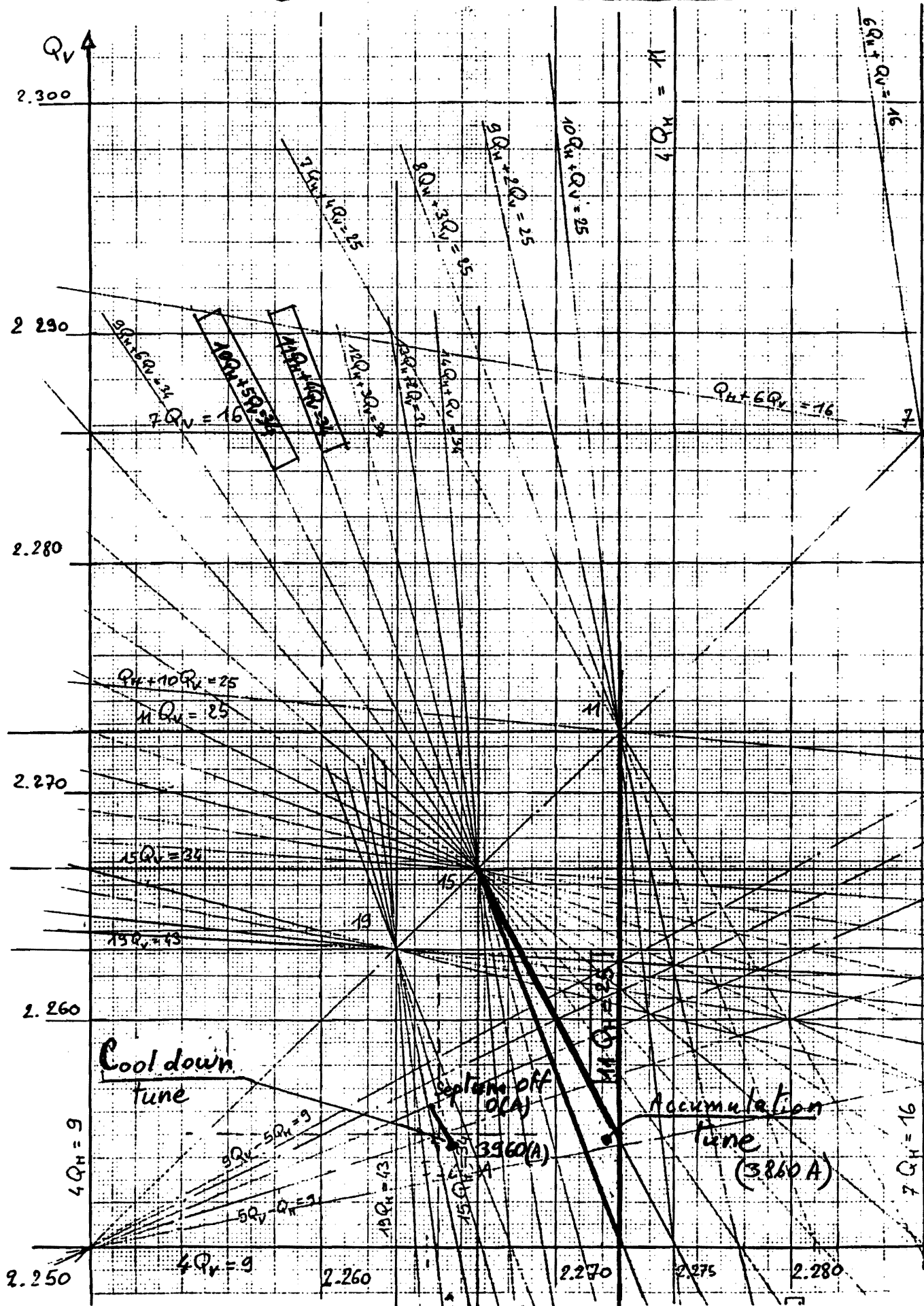
Fig 4 AA working diagram
