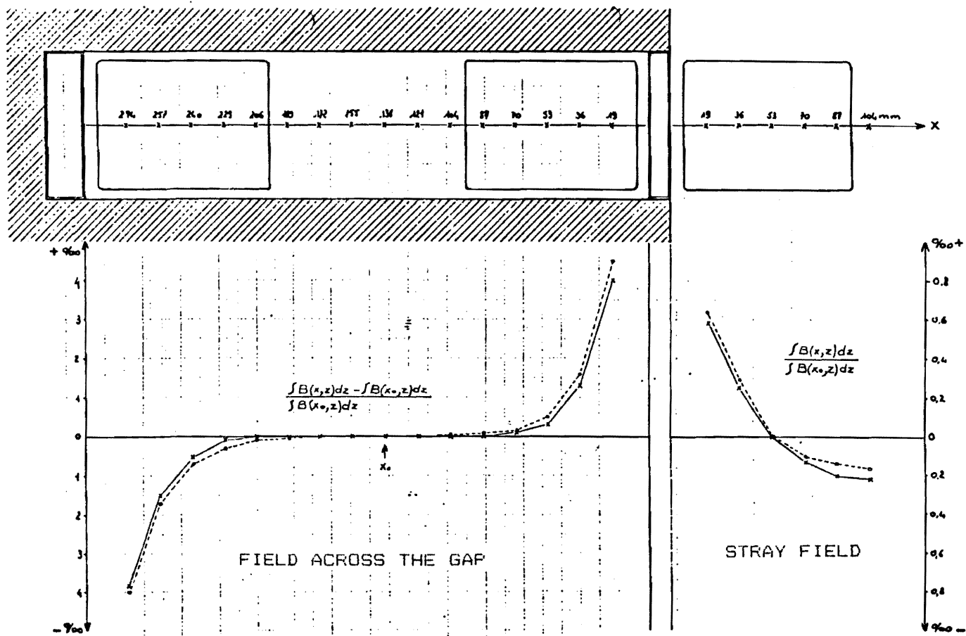
Fig 5 INJECTION/EJECTION SEPTUM MAGNET PERFORMANCE
